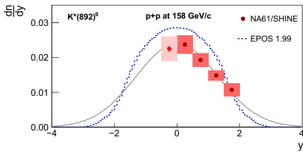
Fig. 14 Comparison of K^*(892)^0 rapidity distribution from NA61/SHINE (points) and the EPOS1.99 model (dashed line). The fitted Gaussian function to NA61/SHINE points (solid line) is given by Eq. (17); the first point (with y < 0 ) was not included in the fit (see the text for details)
