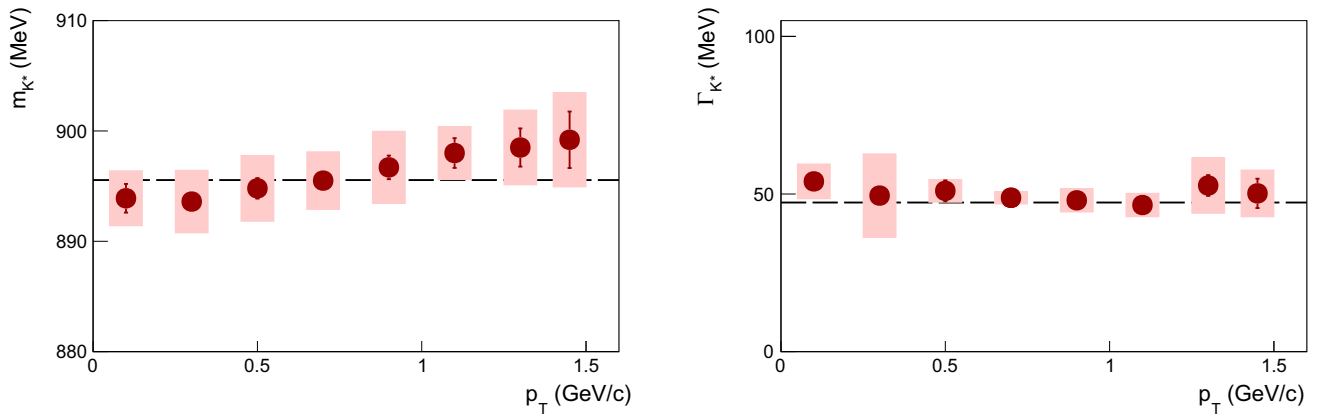
Fig. 8 The transverse momentum dependence of mass and width of K^*(892)^0 mesons fitted for 0 < y < 0.5 . The numerical data are listed in Table 2. The horizontal lines represent PDG values m_0 = 895.55 MeV and \Gamma_0 = 47.3 MeV [35]
