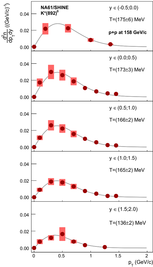
Fig. 10 Transverse momentum spectra \frac{d^2n}{dy dp_T} for five bins of rapidity. The fitted function (solid line) is given by Eq. (12). The numerical values are listed in Table 3 and the fitted inverse slope parameters T for each bin are given in the legends
