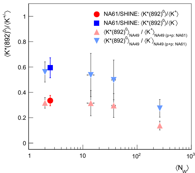
Fig. 16 The system size dependences of \langle K^*(892)^0 \rangle / \langle K^+ \rangle and \langle K^*(892)^0 \rangle / \langle K^- \rangle yield ratios in p+p, C+C, Si+Si and Pb+Pb collisions at 158A GeV/c. N_W denotes the number of wounded nucleons taken from Ref. [4]. The numerical values are listed in Table 8. For better visibility the NA61/SHINE points are shifted on the horizontal axis
