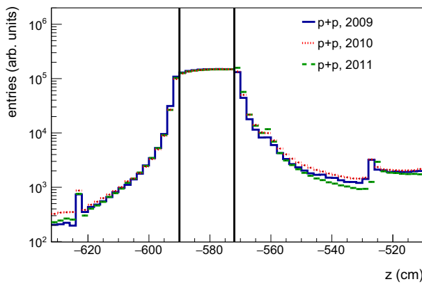
Fig. 2 Left: distributions of the z -coordinate of the reconstructed interaction vertex ( z ) for events recorded with the target inserted (2009, 2010 and 2011 data). Histograms are normalized to the same integral in the range -590 < z < -572 cm. Right: distributions of the z -coordinate of the reconstructed interaction vertex for target-inserted
