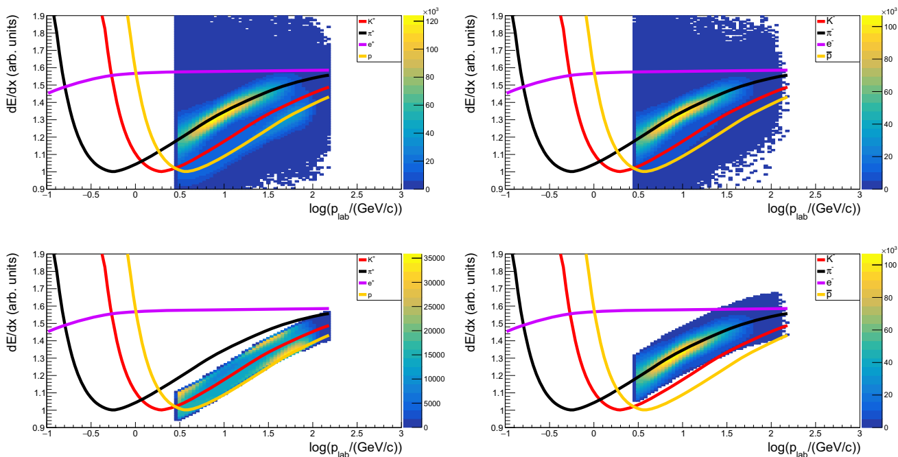
Fig. 3 Top: the values of dE/dx versus \log(p_{lab}/(\text{GeV}/c)) for positively (left) and negatively (right) charged particles after track cuts (i)–(vi) from Sect. 3.4. The Bethe–Bloch curves are also drawn. Bottom: selection of K^+ (left) and \pi^- (right) candidates
