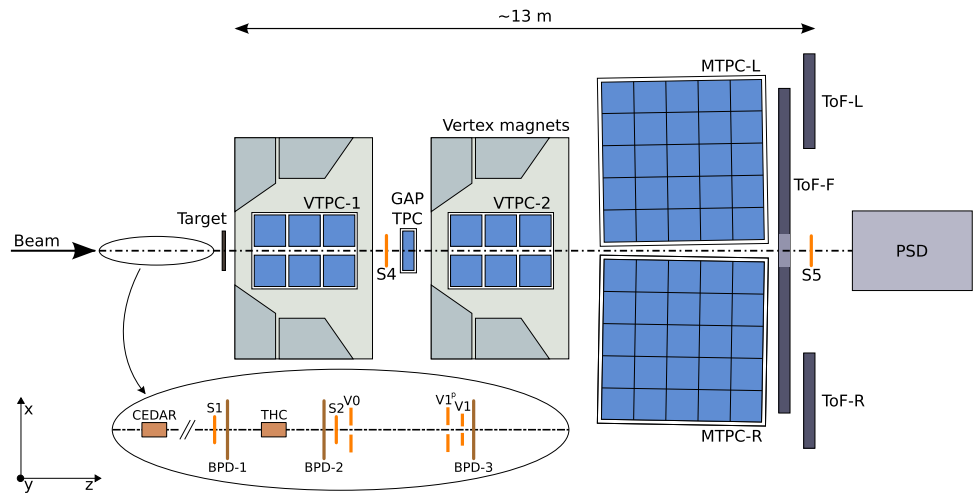
Fig. 1 The schematic layout of the NA61/SHINE experiment at the CERN SPS (horizontal cut, not to scale). The beam and trigger detector configuration used for data taking in 2009 is shown in the inset (see Refs. [28, 29] for detailed description). The chosen coordinate system is drawn on the lower left: its origin lies in the middle of the VTPC-2, on the beam axis
