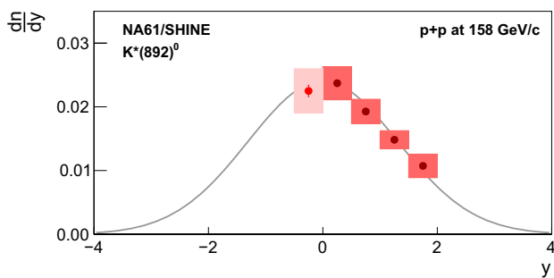
Fig. 12 The p_T -integrated and extrapolated rapidity distribution. The fitted Gaussian function (solid line) is given by Eq. (17); the first point (with y < 0 ) was not included in the fit (see the text for details). The numerical data are listed in Table 5
