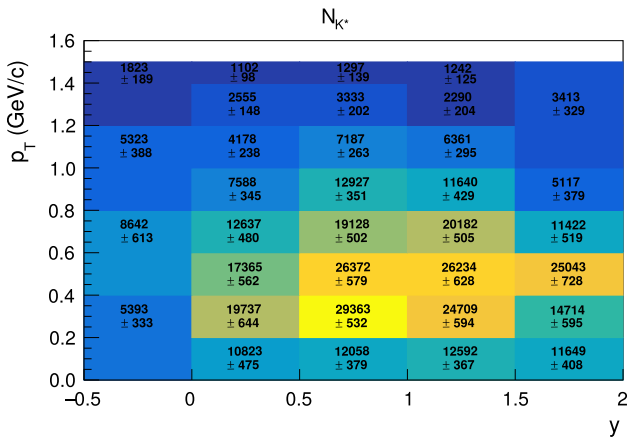
Fig. 6 Uncorrected numbers of K^*(892)^0 obtained from the extraction procedure described in Sect. 3.6. The values are shown with statistical uncertainties
