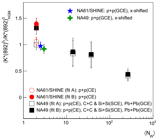
Fig. 15 The mean multiplicity of K^*(892)^0 for p+p reactions (this analysis and NA49 measurement [4]), as well as results of NA49 for C+C, Si+Si and Pb+Pb [4] interactions at 158A GeV/c divided by the HGM predictions [41] for fit B (closed circle and closed squares) and fit A (open circle and open squares), see the text for details. Closed star and cross symbols show p+p measurements compared to HGM predictions for the Grand Canonical Ensemble formulation [42,43]. N_w denotes the number of wounded nucleons taken from Ref. [4]
