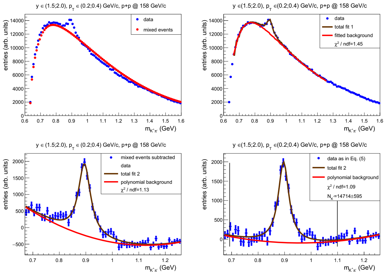
Fig. 5 Same as Fig. 4 but for 1.5 < y < 2.0 and 0.2 < p_T < 0.4 GeV/c
