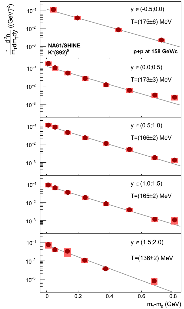
Fig. 11 Transverse mass spectra \frac{1}{m_T} \frac{d^2n}{dm_T dy} for five bins of rapidity. The numerical values are listed in Table 4. The solid lines represent function given by Eqs. (12) and (13) with A and T parameters taken from Fig. 10
