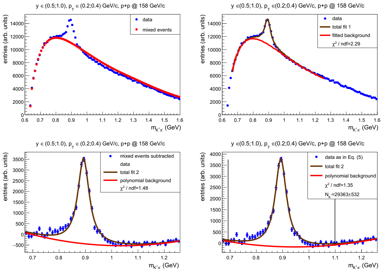
Fig. 4 The example of the procedure of signal extraction for K^*(892)^0 in rapidity bin 0.5 < y < 1.0 (all rapidity values in the paper are given in the center-of-mass reference system) and transverse momentum bin 0.2 < p_T < 0.4 GeV/c for p+p collisions at 158 GeV/c. Top, left: data signal (blue points), and background histogram (red points) obtained from mixed events (standard method). Top, right: data signal
