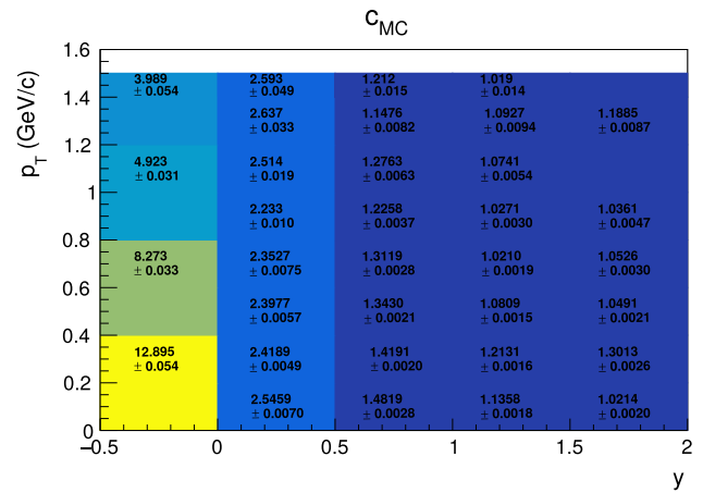
Fig. 7 Correction factors c_{MC} with statistical uncertainties
