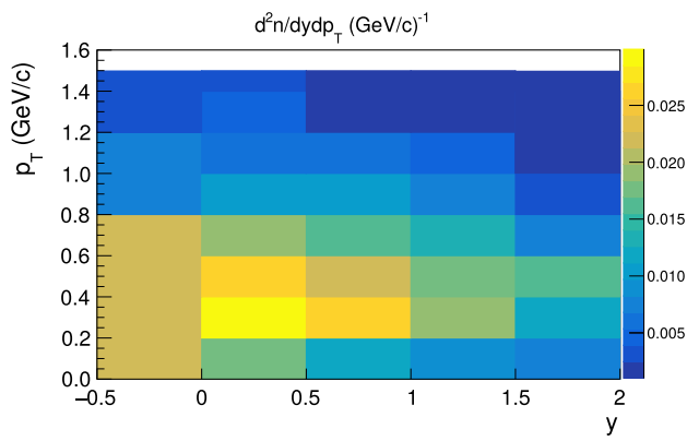
Fig. 9 Double-differential K^*(892)^0 spectra in inelastic p+p interaction at 158 GeV/c in bins of (y, p_T) as obtained from Eq. (10). The numerical values are given in Table 3
