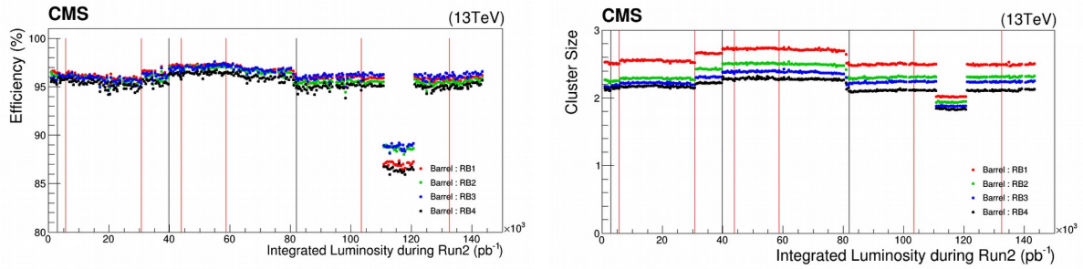
Figure 5: RPC efficiency and cluster size history vs integrated luminosity for the four barrel stations: The plots represent Run-2 history. (Run-1 integrated luminosity is 27 fb -1 ). Each point corresponds to an average efficiency or cluster size per station in a given LHC fill.
