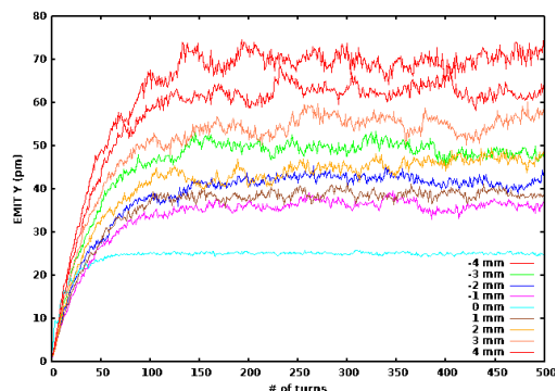
Figure 5: Projected vertical emittance of the weak beam observed at the IP for the corrected lattice in the presence of beam-beam elements at different longitudinal waist positions of the strong beam
