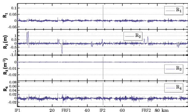
Figure 2: Coupling parameters around the ring for the corrected lattice.
