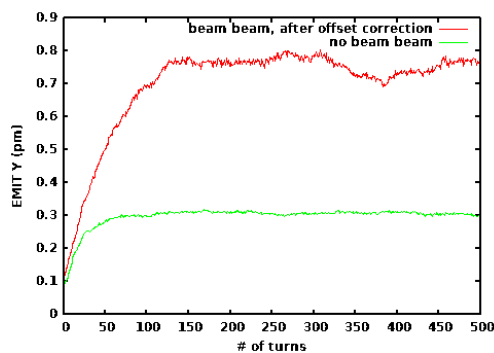
Figure 7: Projected vertical emittance of the weak beam observed at the IP with a beam-beam element after offset correction (red) and without beam-beam element (green).
