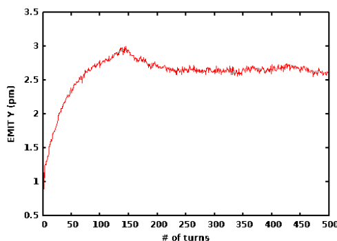
Figure 8: Projected vertical emittance of the weak beam observed at the IP with a beam-beam element after adjusting the invariant vertical emittance of the ring to 0.4 pm.
