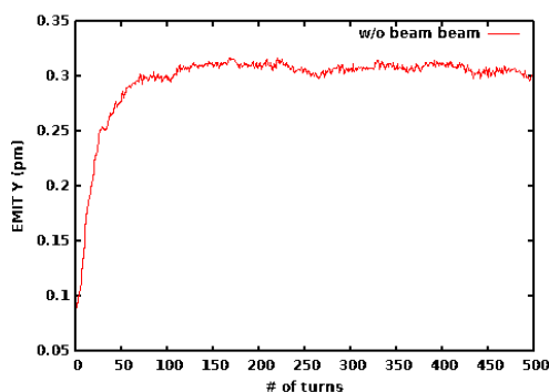
Figure 3: Projected vertical emittance of the weak beam observed at the IP for the corrected lattice without any beam-beam element.
