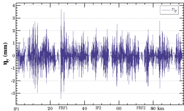
Figure 1: Vertical dispersion around the ring for the corrected lattice.
