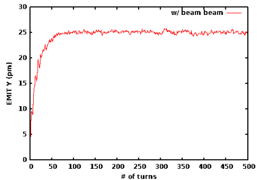
Figure 4: Projected vertical emittance of the weak beam observed at the IP for the corrected lattice in the presence of beam-beam elements
