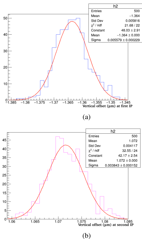
Figure 6: Vertical offset of the weak beam in the presence of beam-beam elements (a) at the first IP and (b) at the second IP.
