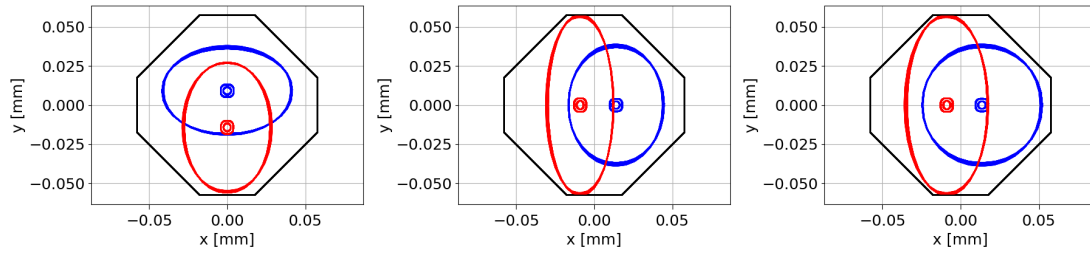
Figure 3: Beam 1 and 2 envelopes at a reference value of 12.7 \sigma in Q3 right of IR5 for Round (left), Flat (centre), and FlatCC (right). The protected aperture depends on the detailed optics (see Table 3). Round optics has more aperture margin than flat optics ( 0.4\sigma ). In flat optics, D1 has a smaller aperture in the horizontal plane by 0.1\sigma to be reviewed once measured mechanical tolerances from prototypes will be available.
