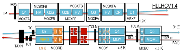
Figure 1: HLLHCv1.4 layout of the right side of IR1 and IR5 with quadrupoles (Q), non-linear corrector package (CP), dipoles (D), collimators and masks (TC), crab cavities (CC), and passive absorbers (TAX).
