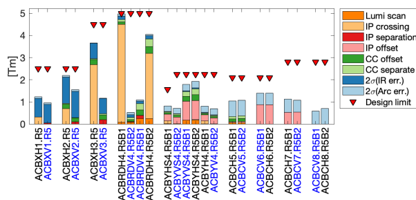
Figure 2: Orbit corrector budget in IR1 and IR5 at 7 TeV. The strength budget includes operational settings (IP crossing and separation, luminosity scan) and correction of imperfections (IP offset, offset and separation at the CCs, and compensation of local and global quadrupole misalignments). The IP offset is meant to compensate for the small step in the Q5 area due to the full remote alignment. The remaining strength can be used to further refine the orbit without using the full remote alignment (e.g. 0.5 mm of IP shift).
