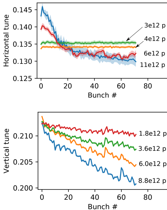
Figure 1: Horizontal (top) and vertical (bottom) bunch by bunch detuning measured in the SPS for trains of 72 bunches of various intensity. The measurement was carried out using a special BPM with single bunch capability. In the horizontal plane no detuning is observed until a threshold is reached. This strongly non-linear behavior is the fingerprint of electron-cloud, that requires a certain beam intensity in order for the cloud to build-up. The linear detuning observed in the vertical plane instead can be attributed to transverse impedance.
