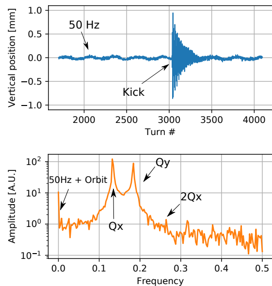
Figure 2: Example of the vertical betatron motion (top) measured by one BPM and spectrum (bottom). In the time domain the 50 Hz noise appears as a steady oscillation with \sim 866 turns period and overlaps the V_{00} line in the frequency domain.
