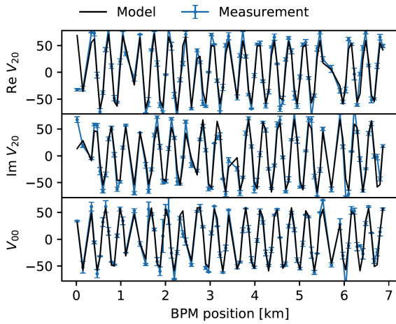
Figure 3: Variation (blue) of the real and imaginary part of the V_{20} spectral line and the V_{00} orbit distortion induced by switching on the static sextupolar field. The analytical model (black) is fitted to the data to obtain the skew-sextupole strength.
