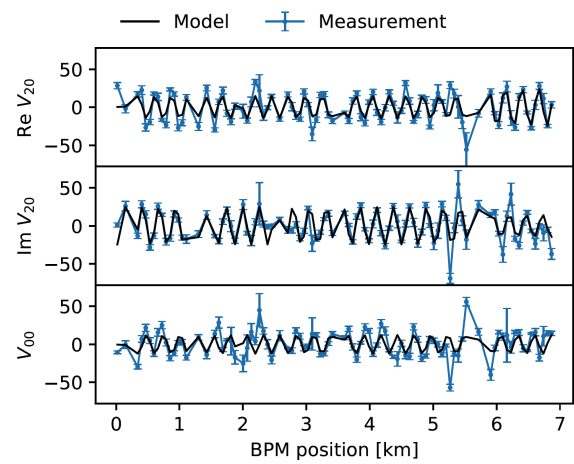
Figure 4: Variation (blue) of the real and imaginary part of the V_{20} spectral line and the V_{00} orbit distortion induced by changing the crab cavity voltage from 100 kV to \sim 1 \text{ MV} . The analytical model (black) is fitted to the data to obtain the crab cavity skew-sextupolar field strength.
