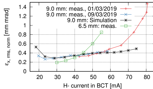
Figure 5: Emittance measurements on a source with 9 mm bore diameter in comparison to measurements with 6.5 mm. The puller voltage was reduced from 10 kV for the latter to 9.5 kV for the former to reduce beam losses in the solenoid.
