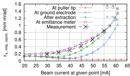
Figure 4: Emittance as a function of beam current at various points throughout the extraction. Puller voltage constant at 10 kV. Left to right in Fig. 1: after the tip of the puller electrode ( z=10 mm), at the ground electrode ( z=48 mm), after the system ( z=14 cm) and at the position of the emittance meter ( z=1.08 m). The electron to ion ratio was set to 2 in the simulation and between 2-3 for the measurement.
