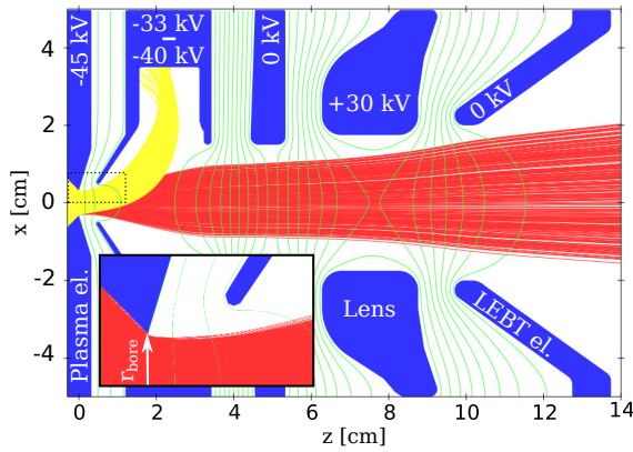
Figure 1: The present extraction system of the Linac4 ion source [7]. Both the source potential and the voltage on the lens are typically left at the given values, while the puller voltage can be chosen between 5 kV to 12 kV.
