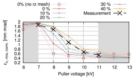
Figure 3: Comparison of rms emittances from simulation and measurement as a function of the electric field in the extraction gap. The extracted beam current is 50 mA. Percentages indicate the increase of density in the plasma region in the simulation.
