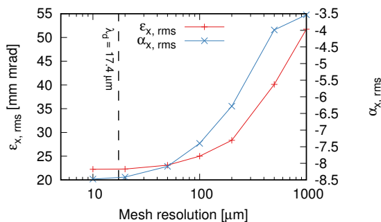
Figure 2: Beam emittance (un-normalized) and divergence of a 30 mA H^- beam after the extraction gap at different resolutions of the cylindrical grid.
