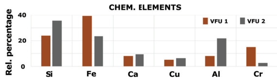
Figure 2: (VFU) EDX analysis results for the two vacuum filter units. The spectra do not reveal information on oxidation states due to the detection limit on light elements. VFU 1 also contained traces of Ti, Ag, F (<0.3% and VFU 2 showed traces (< 0.4%) of Ag and F.
