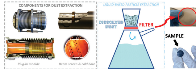
Figure 1: The available UHV components included the plug-in modules (PIMs), beam screen (BS) and cold bore (CB) which are visible in the left part. Liquid-based particle extraction was used to prepare the samples suitable for electron microscopy (middle and right part).
