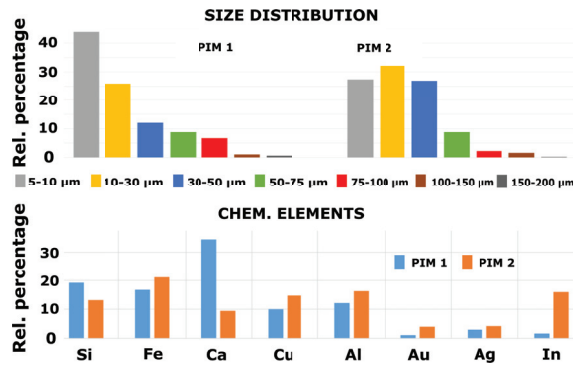
Figure 5: (PIM) The upper part shows the size distributions for particles extracted from PIM 1 and 2. The corresponding chemical composition can be found directly underneath.
