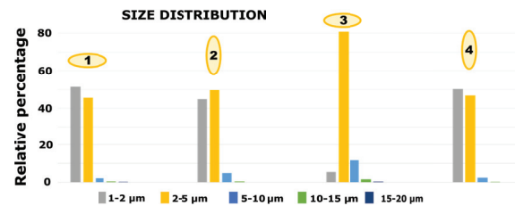
Figure 4: (Wipe test) The size ranges differ from other plots as the samples were the first once to be analysed. Later on, smaller sizes up to 5 μm were excluded. The table includes the total number of particles as a reference.
