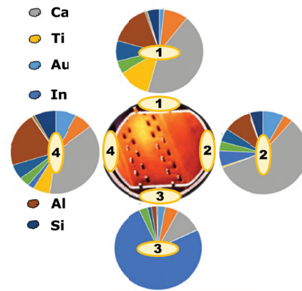
Figure 3: (Wipe test) Beam screen and four positions of wiping. The materials for each position are illustrated by separate pie charts arranged clock-like around the beam screen.
