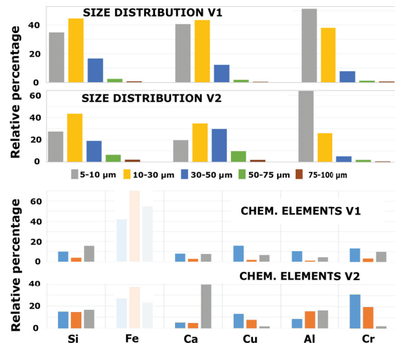
Figure 7: (CB) The top part shows the size distribution for V1 and V2. The results for each of the 3 dusters are grouped into one column. Iron is excluded. The lower part shows the percentage of the most abundant elements and shows the probable contaminants introduced by the measurement in V2.
