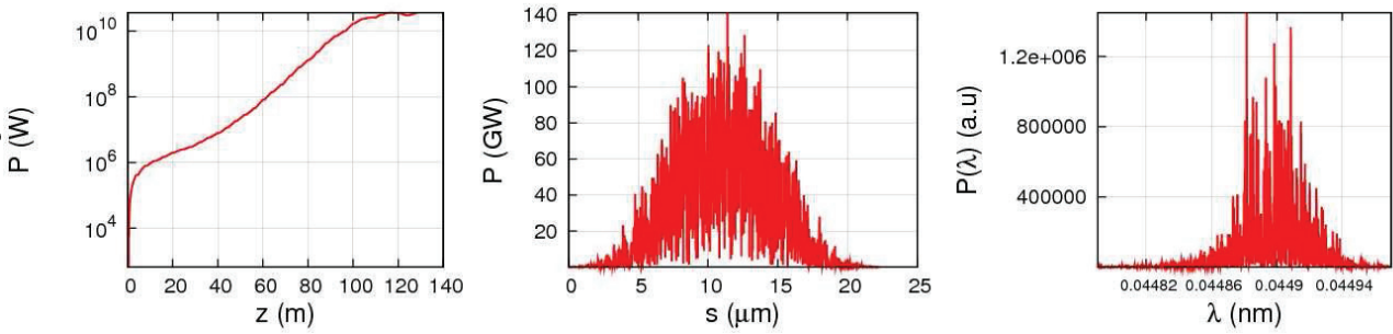
Figure 2: Genesis simulation results for 0.45 Å laser wavelength ( K = 4.24 ). Left: Evolution of the pulse power along the undulator. Middle: Spatial profile of the radiation pulse. Right: Wavelength spectrum of the radiation.
