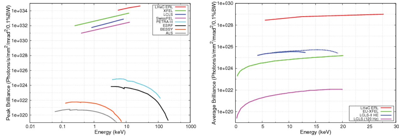
Figure 3: Peak (left) and average brilliance (right) for the LHeC-FEL compared with several existing or planned light sources. The lower curves on the left combine different undulator radiation harmonics. On the right, for LCLS-II-HE the solid curve refers to 8 GeV operation with unmodified injector, while the dashed curve assumes an injector upgrade [26].
