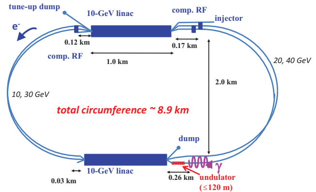
Figure 1: LHeC ERL reconfigured for FEL operation.
