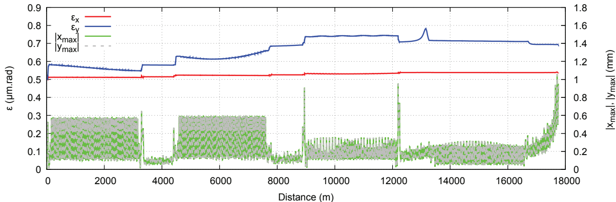
Figure 4: Simulated evolution of the two transverse normalized emittances (after subtracting dispersive contributions) and maximum particle position while decelerating the spent beam over 2 complete LHeC turns from 40 to 0.6 GeV.
