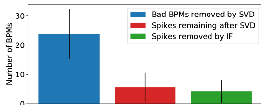
Figure 2: This summary represents the number of outliers in \beta -beating and phase advance averaged over 10 measurements of Beam 1 and Beam 2 performed during MDs in 2018.
