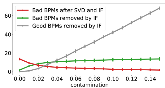
Figure 3: Adjustment of contamination factor of IF algorithm and its effect on the trade-off between cleaning of bad BPMs and removal of good ones.
