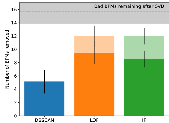
Figure 5: The comparison is carried out on 20 simulations for each plane, the results are averaged. Each bar represents the number of BPMs removed by the method. Dark fraction corresponds to the number of removed BPMs that are actually bad.
