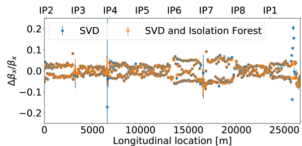
Figure 1: The comparison between beta-beating computed before and after IF cleaning demonstrates that IF anomaly detection significantly reduces the number of unphysical spikes and reduces the size of errorbars. The optics is computed for Beam 2 in horizontal plane with \beta^*=50 cm.
