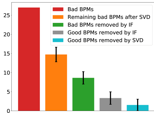
Figure 4: Averaged results of faulty BPMs detection on 20 simulated measurements using contamination factor 0.02.
