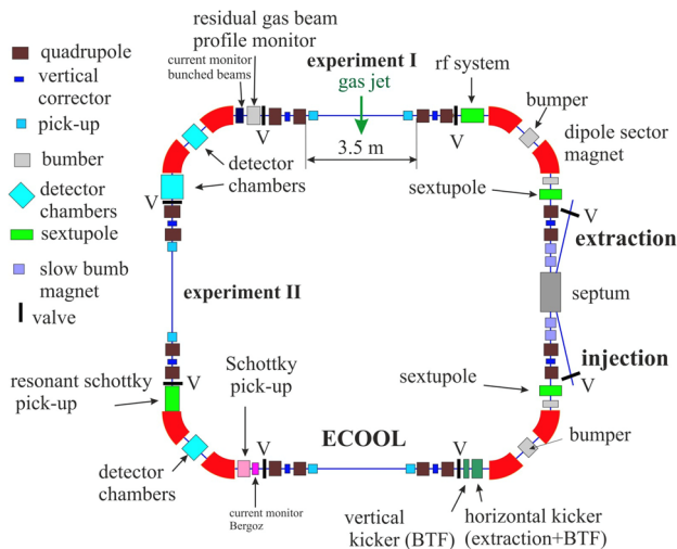
Figure 2: Layout for a new compact ISOLDE storage ring by M. Grieser, MPI-K Heidelberg
