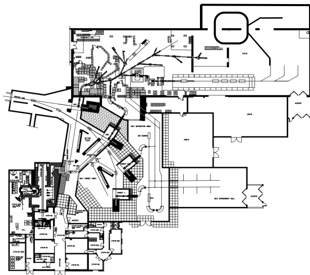
Figure 1: Preliminary layout of the ISOLDE target area with beam lines to the experimental hall and the implantation of the ISR.
