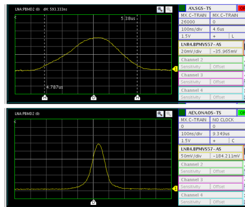
Figure 6: Bunch length before (top) and after (bottom) combined bunch rotation and bunched beam cooling.
