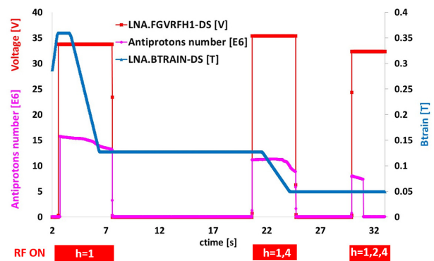
Figure 4: Antiproton cycle with three RF segments and h = 1, 4, 2 . Traces: Btrain [blue], voltage program [red], bunched beam intensity [pink].
