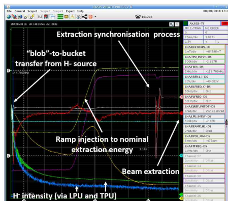
Figure 5: Typical H - production cycle in 2018.
