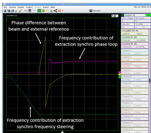
Figure 3: Extraction synchronisation process for an antiproton beam at h = 4 and a reference at h = 1 .
