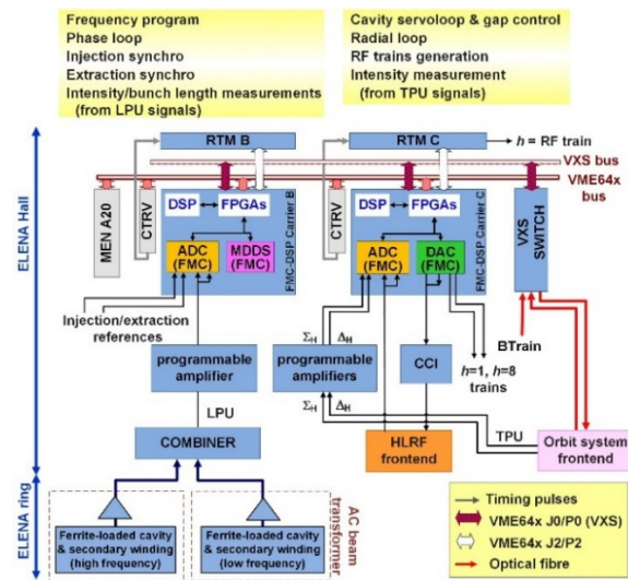
Figure 2: LLRF layout. Keys: MDDS – Master Direct Digital Synthesiser, ADC – Analogue-to-Digital Converter, DAC – Digital-to-Analogue Converter, CTRV – Timing Receiver Module, MEN A20 – Master VME board, RTM – Rear Transition Module, CCI – Cavity Control Interface, LPU/TPU – Longitudinal/Transverse Pick-Up.
