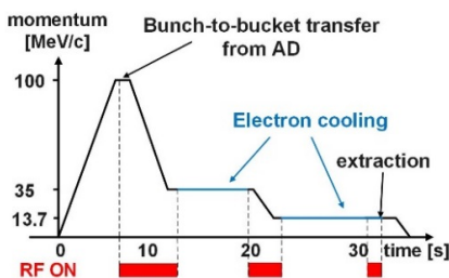
Figure 1: ELENA cycle for antiprotons operation.
