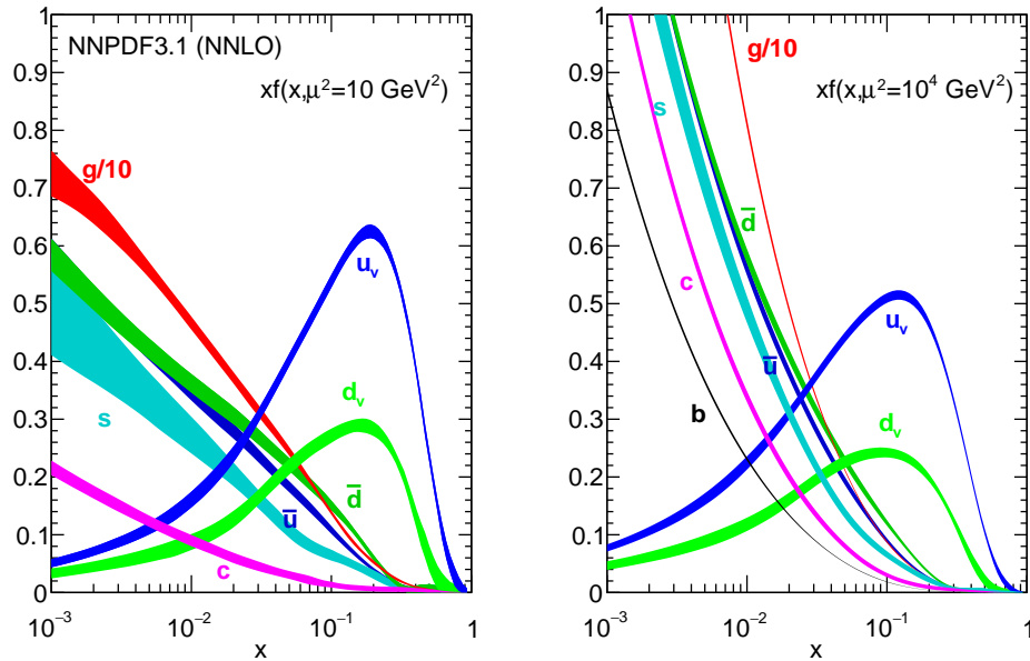
Fig. 4.4: Different PDFs as obtained at NNLO level (NNPDF3.1) from Ref. [173], evaluated at \mu^2 = 10 \text{ GeV}^2 (left) and \mu^2 = 10^4 \text{ GeV}^2 (right).
