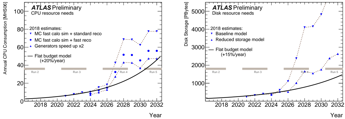
Fig. 11.2: Estimated CPU (left) and total disk resources (right) needed by the ATLAS experiment as a function of time for both data and simulation processing. Plots taken from [732].
