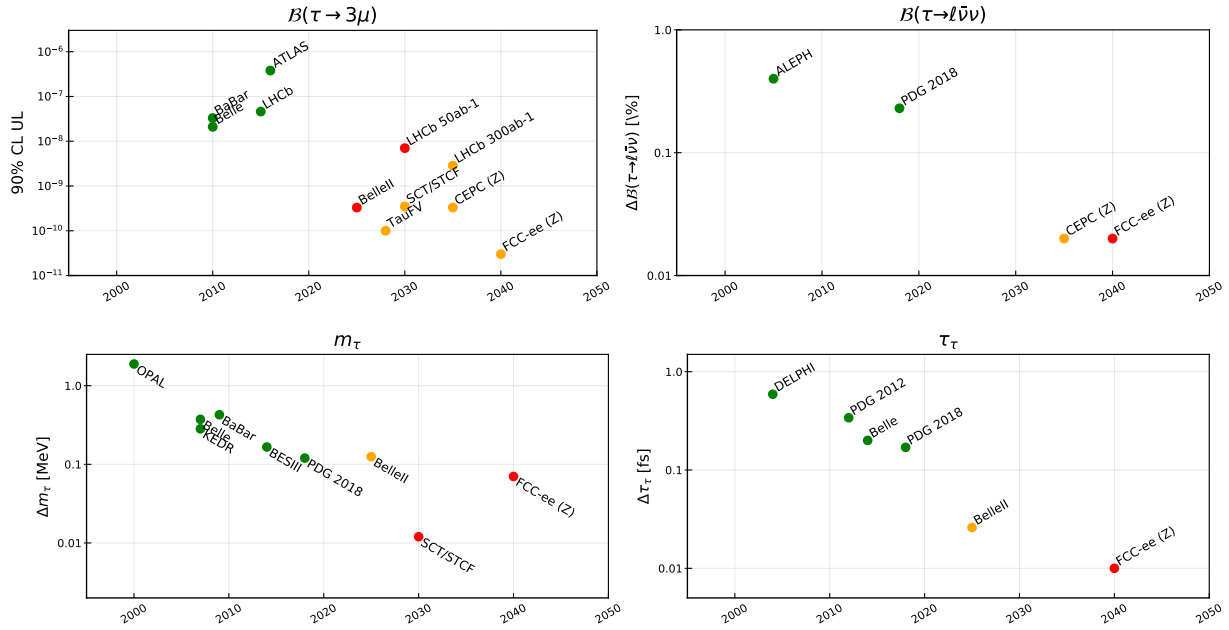
Fig. 5.11: Expected sensitivity and projected precision of present and future experiments for \tau \rightarrow 3\mu , \tau \rightarrow \ell\bar{\nu}\nu decays, m_\tau and \tau_\tau [338]. Green denotes current measurements, red points correspond to estimates of future experimental sensitivities based on dedicated studies (relying on extrapolation from past established performances) while orange corresponds to estimates of experimental sensitivities including novel features (for which extrapolation from past experience is more difficult).
