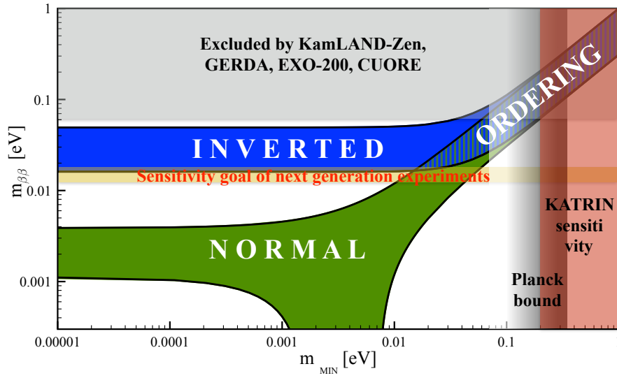
Fig. 6.5: The effective mass m_{\beta\beta} controlling the rate of the neutrino-less double beta decay versus the mass of the lightest eigenstate [388]. The limits from the current and future experiments are shown.
