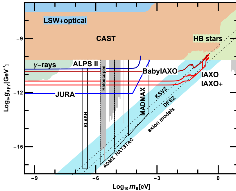
Fig. 9.7: Current exclusion of ALPs and axions coupling to photons in the sub-eV mass-scale (see, e.g., [356,620] for details) with experimental prospects. Astrophysical limits are shown in green, pure laboratory experiments are indicated in blue, helioscopes in red and haloscopes in grey. The turquoise shaded region indicates the typical coupling range expected for QCD axion models. Couplings to other particles than photons are discussed in the supporting note [524].
