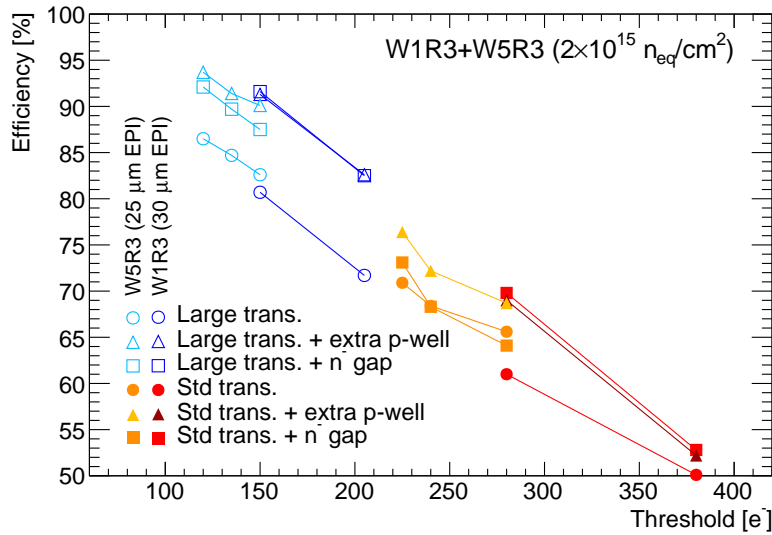
Figure 15. Efficiency versus threshold mean for neutron irradiated Mini-MALTA samples at 2 \times 10^{15} 1 MeV n_{eq}/cm^2 ( -10 V substrate voltage, -20^\circ\text{C} ). Different sensor regions are presented: standard MALTA-like (circles), modified with extra deep p-well (triangles) and modified with extra n^- gap (rectangles). Results are also shown for sensor regions with standard (open markers) and enlarged (full markers) transistors, as well as for sensors with different epitaxial layer thicknesses: 25 \mu\text{m} (orange or light blue symbols) and 30 \mu\text{m} (red or dark blue symbols).
