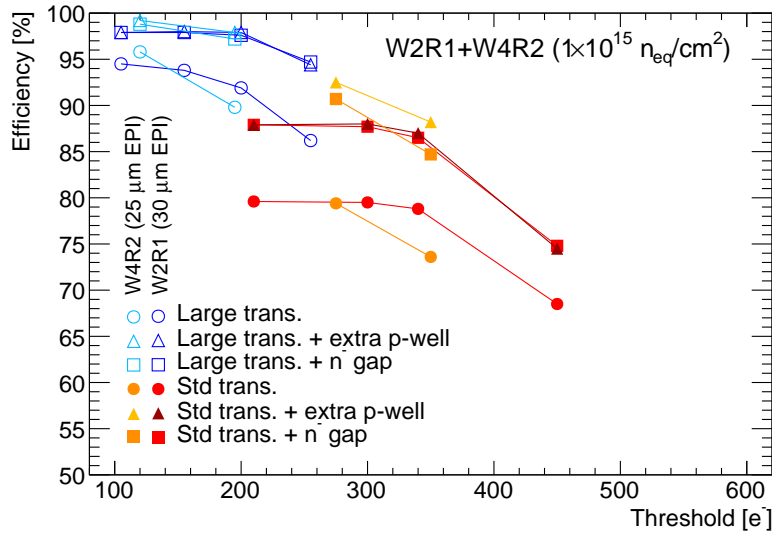
Figure 14. Efficiency versus threshold mean for neutron irradiated Mini-MALTA samples at 1 \times 10^{15} 1 MeV n_{eq}/cm^2 ( -6 V substrate voltage, -20^\circ\text{C} ). Different sensor regions are presented: standard MALTA-like (circles), modified with extra deep p-well (triangles) and modified with extra n^- gap (rectangles). Results are also shown for sensor regions with standard (open markers) and enlarged (full markers) transistors, as well as for sensors with different epitaxial layer thicknesses: 25 \mu\text{m} (orange or light blue symbols) and 30 \mu\text{m} (red or dark blue symbols).
