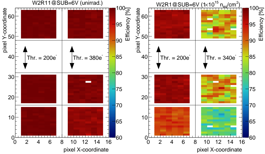
Figure 10. 2D efficiency maps for non-irradiated (left) and irradiated Mini-MALTA samples at 1 \times 10^{15} 1 \text{ MeV } n_{eq}/\text{cm}^2 (right). Different sensor regions are visible: standard MALTA-like (bottom part of each chip), modified with extra deep p-well (middle part) and modified with extra n^- gap (top part). Results are also shown for sensor regions with standard (right side of each chip) and enlarged (left side) transistors. The chips were operated at -6 \text{ V} substrate voltage and -20^\circ\text{C} , and were tuned for low threshold.
