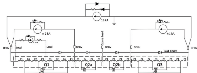
Figure 1: Circuit layout of the HL-LHC inner triplet, showing the quadrupoles Q1, Q2a, Q2b, Q3, the main, and trim power converters with their crowbars, the Coupling Loss Induced Quench protection systems (C) and the cold diodes [5, 6].
