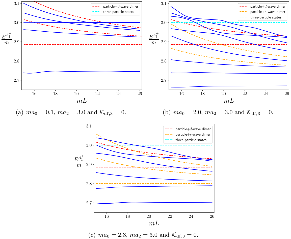
Figure 12. Finite-volume spectra (solid blue lines) of the three-particle systems in the \mathbb{A}_1^+ irrep with both s - and d -wave two-particle interactions. Noninteracting three-particle levels, as well as those involving particle + dimer, are also shown. (In the upper right panel, the cyan dashed line at E = 3m has been shifted slightly downward to make it visible.) See text for further discussion.
