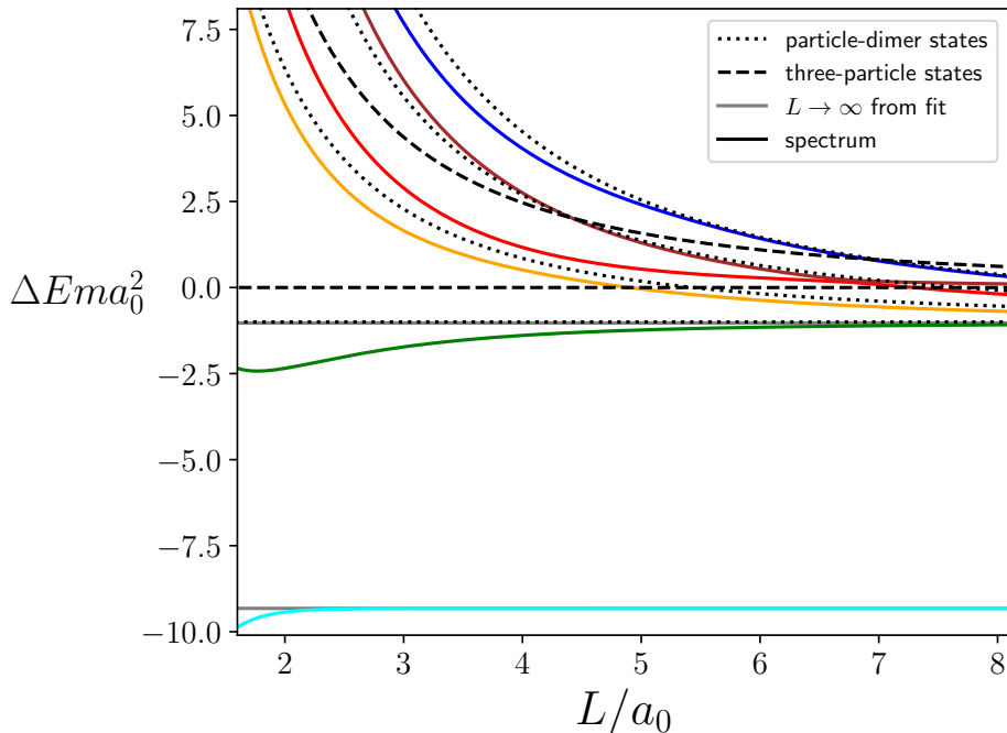
Figure 6. Spectrum as a function of the box size for ma_0 = 16 and \mathcal{K}_{\text{df},3}^{\text{iso}} = 0 , with \Delta E = E - 3m the nonrelativistic energy. In order to facilitate comparison with Ref. [40], the quantities plotted are made dimensionless using appropriate factors of a_0 , and thus differ from those in Figs. 4 and 5.
