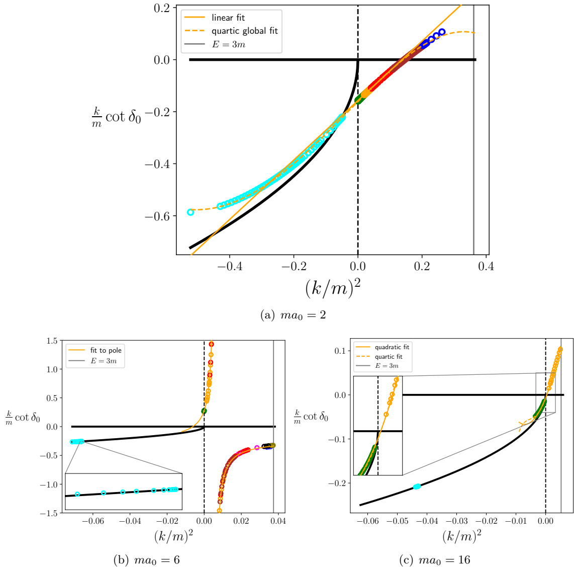
Figure 7. k \cot \delta_0(k) for particle-dimer scattering as a function of the relative center-of-mass momentum k , as determined from the three-particle finite-volume spectrum in the 2 + 1 regime using Eq. (4.8). We set \mathcal{K}_{\text{df},3}^{\text{iso}} = 0 throughout, and consider three different choices of ma_0 . Different colors represent data points coming from different states in the spectrum, and there is considerable overlap of points for k^2 > 0 . The solid vertical line near the right-hand edge of each plot shows the value of (k/m)^2 corresponding to the three-particle threshold, i.e. E = 3m . The curved solid line for negative k^2 shows -|k| = -\sqrt{-k^2} . A bound state is present whenever k \cot \delta_0(k) passes through this line. The fits and other aspects of the plots are described in the text.
