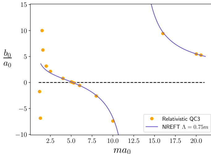
Figure 8. Ratio of particle-dimer scattering length, b_0 , to the fundamental scattering length, a_0 , as a function of ma_0 . Orange points give the results obtained from the analysis described in this subsection applied to the output of the three-particle quantization condition (QC3). The solid (blue) line is the result from (infinite-volume) NREFT, discussed in more detail in Appendix B. The rapid variation of points on the left-side of the plot correspond to a narrow pole in the relation between b_0 and a_0 that only arises in the relativistic theory.
