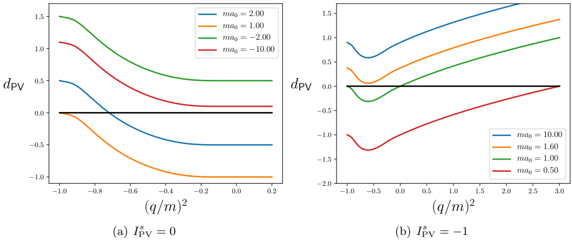
Figure 2. Plots of the denominator of \tilde{\mathcal{K}}_2^s , d_{\text{PV}}(q^2) , vs. q^2/m^2 for a range of choices of am with I_{\text{PV}}^s = 0 (left) and I_{\text{PV}}^s = -1 (right). There is a pole in \tilde{\mathcal{K}}_2^s whenever d_{\text{PV}}(q^2) vanishes. See text for further discussion.
