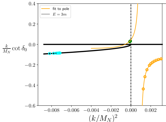
Figure 10. s -wave phase shift as a function of the center-of-mass frame momentum for the simplified toy model describing nucleon-deuteron scattering. Parameters are M_N a_0 = 20.56 and M_N^2 \mathcal{K}_{\text{df},3}^{\text{iso}} = -33500 . Notation as in Fig. 7. The fit is discussed in the text.
