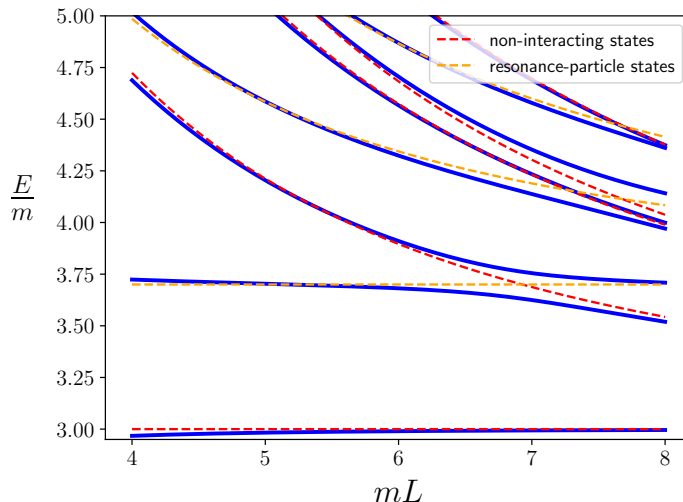
Figure 11. Three-particle spectrum (solid blue lines) in the isotropic approximation in the presence of a two-particle resonance with g = 1 , m_R = 2.7m and \mathcal{K}_{\text{df},3} = 0 . Noninteracting three-particle states (red dashed lines) and noninteracting particle + resonance states (orange dashed lines) are shown for comparison.
