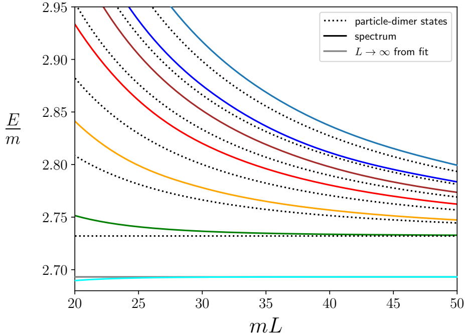
Figure 5. Low-lying spectrum for ma_0 = 2 and \mathcal{K}_{df,3}^{\text{iso}} = 0 for larger mL . This is the continuation to larger volumes of the spectrum shown in the bottom right-hand panel of Fig. 4. Note the highly compressed vertical scale. The horizontal line for the lowest level gives the L \rightarrow \infty asymptote for the trimer energy, using a fit described in the text.
