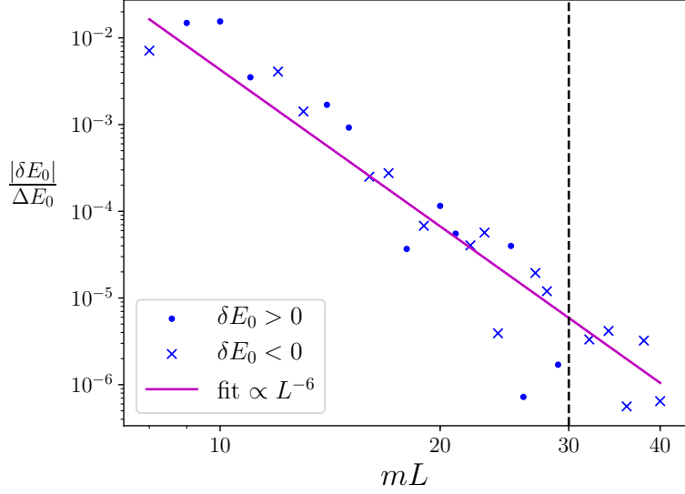
Figure 14. I_{\text{PV}} -dependence of the ground-state energy E_0(L) , with \delta E_0 defined in Eq. (A.3). We plot the ratio to \Delta E_0 = E_0 - 3m in order to give a sense of the relative size of the shift. The vertical line at mL = 30 indicates the point at which matching is performed, so that \delta E_0 vanishes.
