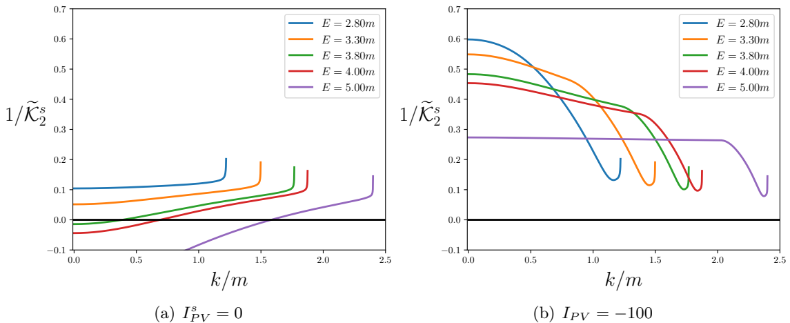
Figure 3. 1/\tilde{\mathcal{K}}_2^s vs |\vec{k}|/m , with \vec{k} the spectator momentum for the Breit-Wigner form of the phase shift given in Eq. (2.10), with the resonance parameters set to g = 1 and m_R = 2.7m . Thus the resonance only leads to a zero crossing for E > 3.7m . Results are shown for (a) I_{PV}^s = 0 and (b) I_{PV}^s = -100 .
