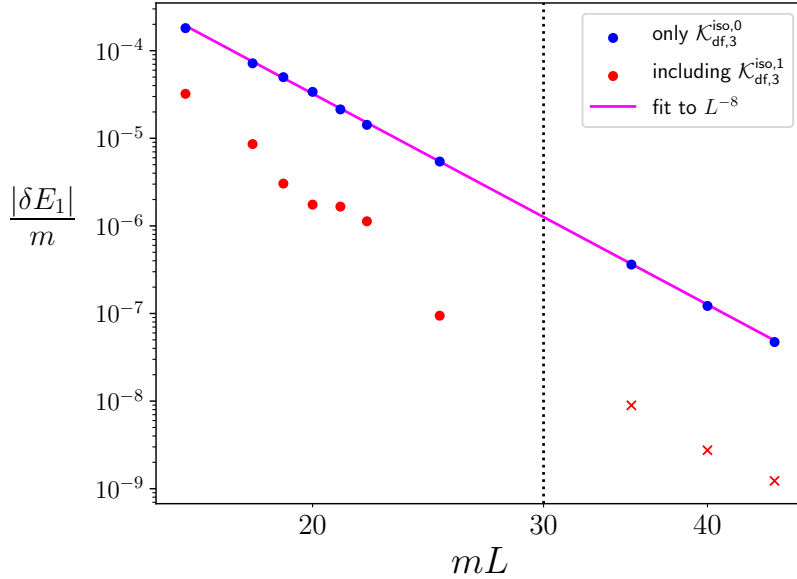
Figure 16. |\delta E_1| as a function of mL when tuning with only a constant \mathcal{K}_{\text{df},3}^{\text{iso},0} (filled blue circles) or with the linear dependence on \Delta given in Eq. (A.6) (filled red circles and crosses). The solid (magenta) line shows a fit to the blue points assuming an L^{-8} -dependence. The vertical line indicates the value of mL at which the tuning is done. Thus the corresponding red point vanishes at this value and is not shown. \delta E_1 is positive for the red circles and negative for the red crosses.
