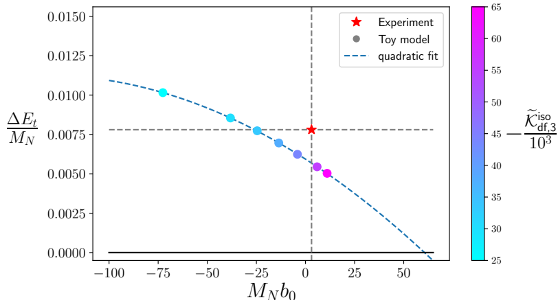
Figure 9. Correlation between the triton (trimer) binding energy and the particle-dimer (nucleon-deuteron) scattering length. This is usually referred to as the Phillips line. The value of \tilde{\mathcal{K}}_{\text{df},3}^{\text{iso}} = M_N^2 \mathcal{K}_{\text{df},3}^{\text{iso}} used for each point can be determined from the color gradient at right. For further discussion see the text.
