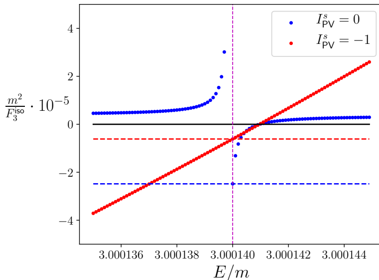
Figure 13. Determining the I_{\text{PV}}^s dependence of \mathcal{K}_{\text{df},3} in the isotropic approximation using the ground-state energy, E_0 , for ma_0 = 0.1 and mL = 30 . Blue and red points show m^2/F_3^{\text{iso}} for, I_{\text{PV}}^s = 0 and -1 , respectively. The vertical purple dashed line shows our chosen tuning energy, while the horizontal dashed curves show the resulting values of -\mathcal{K}_{\text{df},3}^{\text{iso}} .
