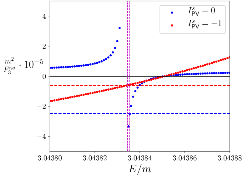
Figure 15. As for Fig. 13 but for the first excited state. The dashed magenta lines correspond to the values of E_1(I_{\text{PV}} = 0; mL = 30) and E_1(I_{\text{PV}} = -1; mL = 30) obtained from the constant approximations m^2 \mathcal{K}_{\text{df},3}^{\text{iso}}(I_{\text{PV}} = 0) = 2.4828 \cdot 10^5 and m^2 \mathcal{K}_{\text{df},3}^{\text{iso}}(I_{\text{PV}} = -1) = 6.1365 \cdot 10^4 . The discrepancy between the two magenta lines is due to our neglect of the higher-order terms in the threshold expansion of \mathcal{K}_{\text{df},3} .
