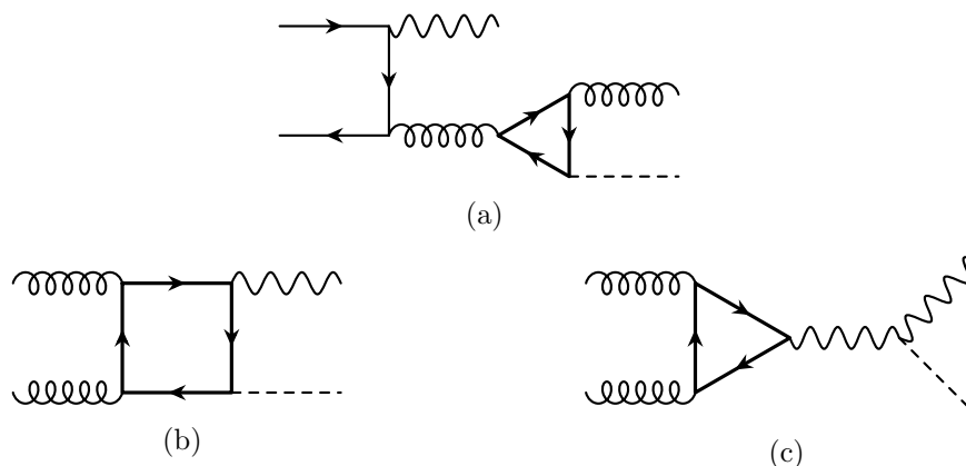
Figure 3. Representative Feynman diagrams of the heavy-quark-loop-induced amplitudes at \mathcal{O}(\alpha_s^2) included in our calculation. Figure (a) depicts an R_T -type amplitude, which is present for both ZH and WH production channels. Figures (b), (c) illustrate representative gluon-gluon induced heavy quark loop amplitudes, which are only present for ZH production.
