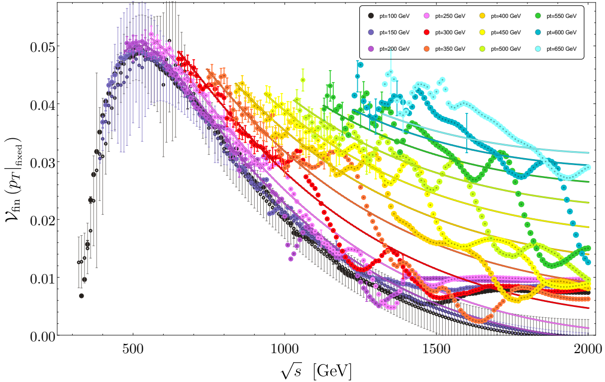
Figure 5: \mathcal{V}_{\text{fin}} as a function of \sqrt{s} for fixed values of p_T . The data points and the corresponding uncertainty bars are obtained from the grid [42]. The solid lines are based on the Padé-improved high-energy expansion. For high values of p_T the uncertainties of the Padé results are smaller than the thickness of the lines. The uncertainties shown for p_T values below 200 GeV are taken over from Fig. 4.
