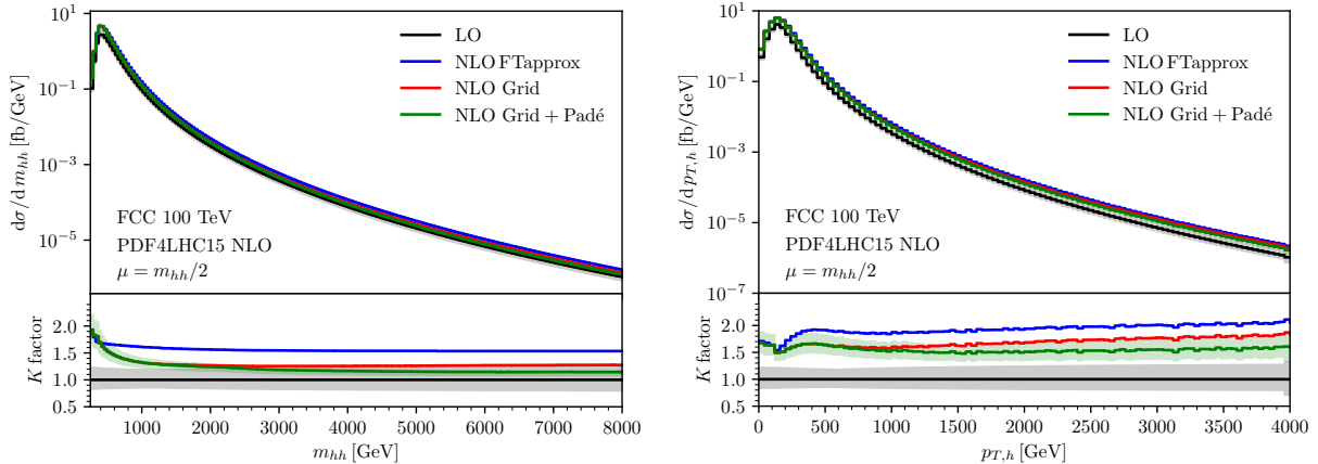
Figure 9: m_{hh} and p_{T,h} distributions for a hadronic centre-of-mass energy \sqrt{s_H} = 100 TeV.
