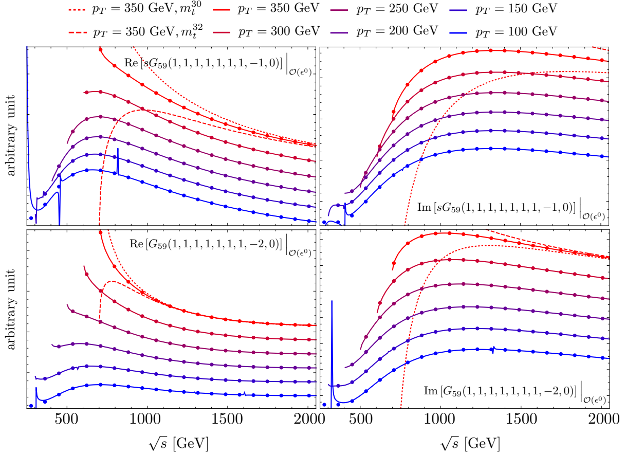
Figure 2: Real and imaginary parts of the master integrals G_{59}(1, 1, 1, 1, 1, 1, 1, -1, 0) and G_{59}(1, 1, 1, 1, 1, 1, 1, -2, 0) as a function of \sqrt{s} and various fixed values of p_T . Solid lines are obtained from the Padé-improved expansion in m_t . The values of p_T decrease from top to bottom. The dots are numerical results obtained with pySecDec , which have small error bars which are not visible in the plot. For the renormalization scale \mu = m_t has been chosen.
