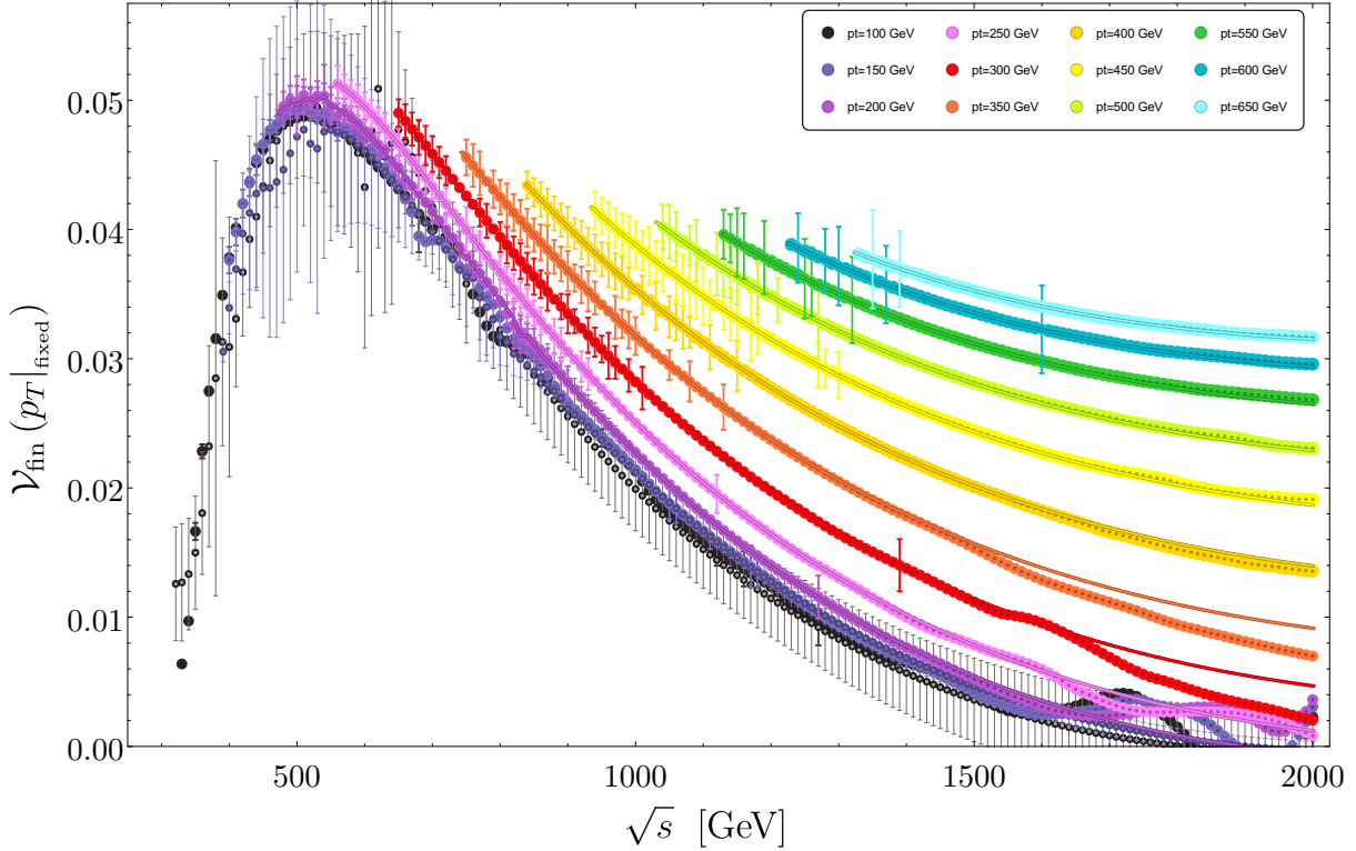
Figure 7: \mathcal{V}_{\text{fin}} as a function of \sqrt{s} for fixed values of p_T . The data points are obtained from the improved version of the grid and the solid lines are based on the Padé-improved high-energy expansion.
