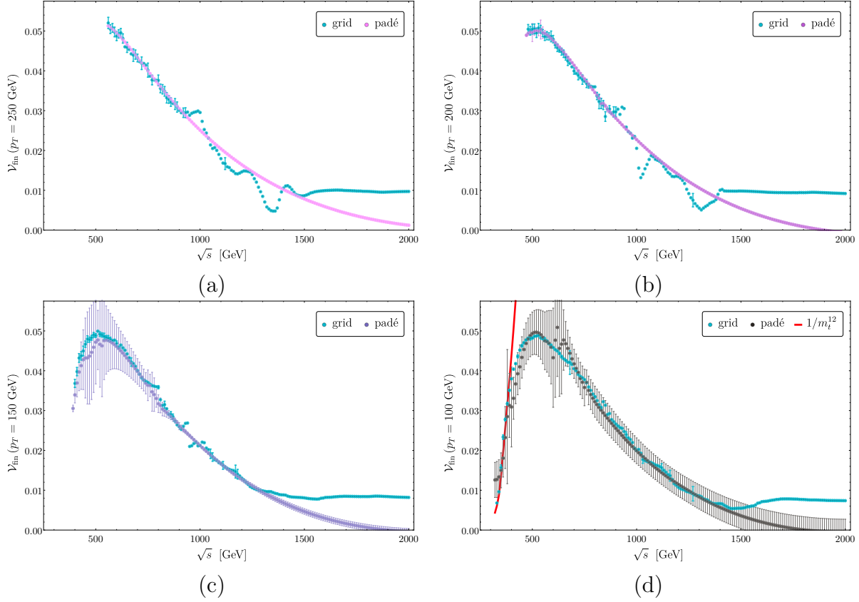
Figure 4: \mathcal{V}_{\text{fin}} as a function of \sqrt{s} for selected values of p_T : (a) p_T = 250 GeV, (b) p_T = 200 GeV, (c) p_T = 150 GeV, (d) p_T = 100 GeV. Both the grid points [12, 42] and the combined Padé improved results are shown. For p_T = 100 GeV we also show the large- m_t expansion including terms up to order 1/m_t^{12} .
