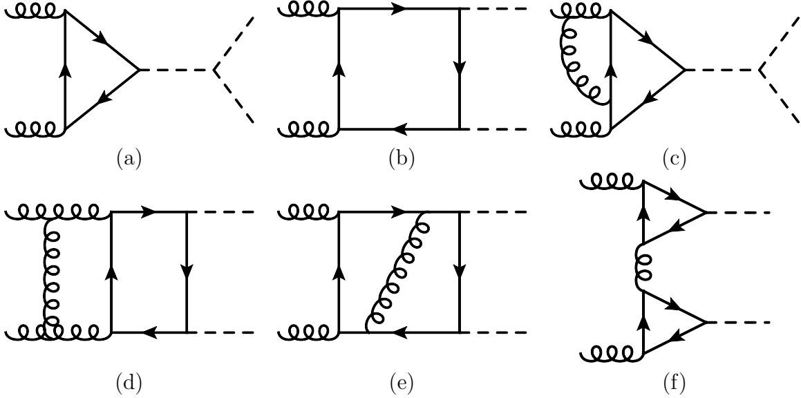
Figure 1: One- and two-loop Feynman diagrams contributing to gg \rightarrow HH . Solid, curly, and dashed lines represent fermions, gluons, and Higgs bosons respectively.
