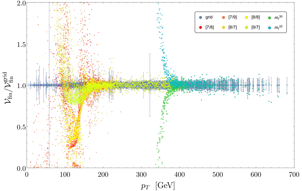
Figure 3: \mathcal{V}_{\text{fin}} normalized to the central values provided in [42] as a function of p_T . The dark blue data points with error bars are obtained from [12,42]. The data points without uncertainty bars are based on \mathcal{V}_{\text{fin}}^N , see legend and text for details.
