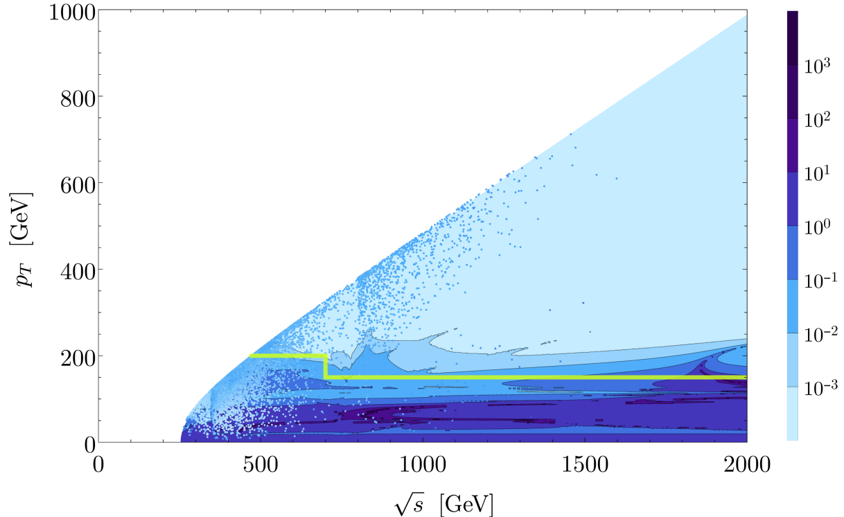
Figure 6: Relative uncertainty of the Padé results in the \sqrt{s} - p_T plane. The points of [42] are overlaid. Note that a logarithmic scale is used for the relative uncertainty.
