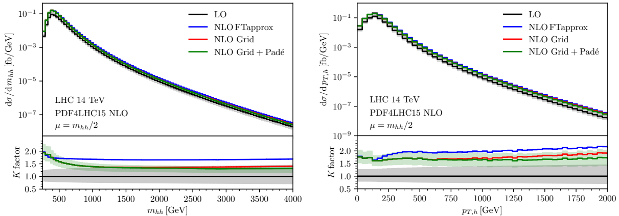
Figure 8: m_{hh} and p_{T,h} distributions for a hadronic centre-of-mass energy \sqrt{s_H} = 14 TeV.
