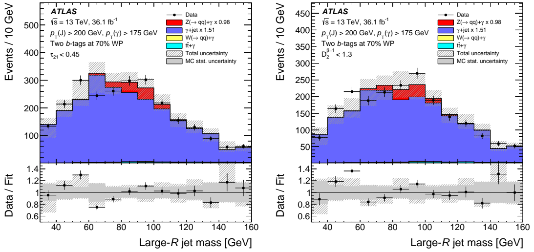
Figure 19: Z \rightarrow b\bar{b} candidate jet mass after applying the \tau_{21} < 0.45 (left) or D_2^{\beta=1} < 1.3 (right) requirement. Events with two b -tagged track-jets are used. The \gamma + jets background and the Z \rightarrow b\bar{b} signal are normalised to data by applying a scale factor of 1.51 and 0.98, respectively.
