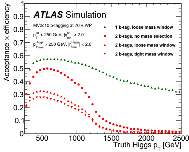
Figure 6: The Higgs boson acceptance times efficiency is shown for a few working points: the double and single b -tagging with the loose mass window requirement and the double b -tagging with the tight, loose and no mass window requirements.
