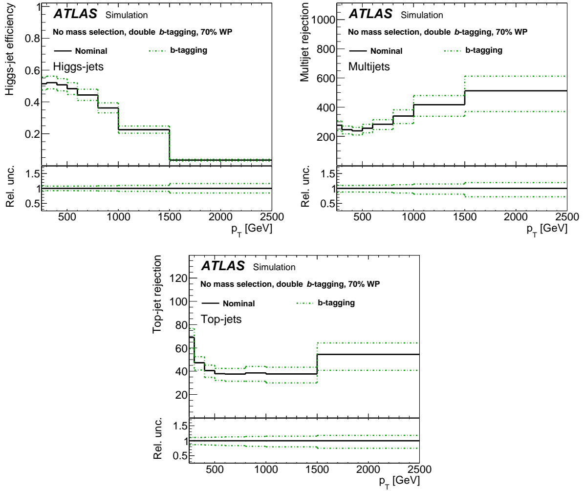
Figure 2: The Higgs-jet efficiency (top left) and rejection against multijet (top right) and top-jet backgrounds (bottom) as a function of the jet p_T for the 70% double- b -tagging working point. The nominal curves correspond to the requirement on the MV2c10 discriminant described in Section 6.2. The b -tagging-related uncertainties defined in Section 5 are shown.
