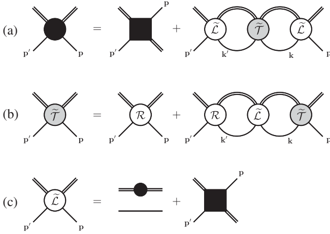
FIG. 4. Diagrammatic representation of (a) the 3 \rightarrow 3 amplitude Eq. (16) in terms of the ladder series and the B -matrix divergence-free amplitude dressed by initial and final state rescatterings, (b) the integral equation for the B -matrix divergence-free amplitude Eq. (17), and (c) the B -matrix rescattering function Eq. (19).
