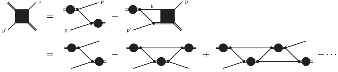
FIG. 3. Diagrammatic representation for the ladder series generated by particle exchanges, Eq. (15), where the black box represents \mathcal{D}_{\mathbf{p}'\mathbf{p}} .
