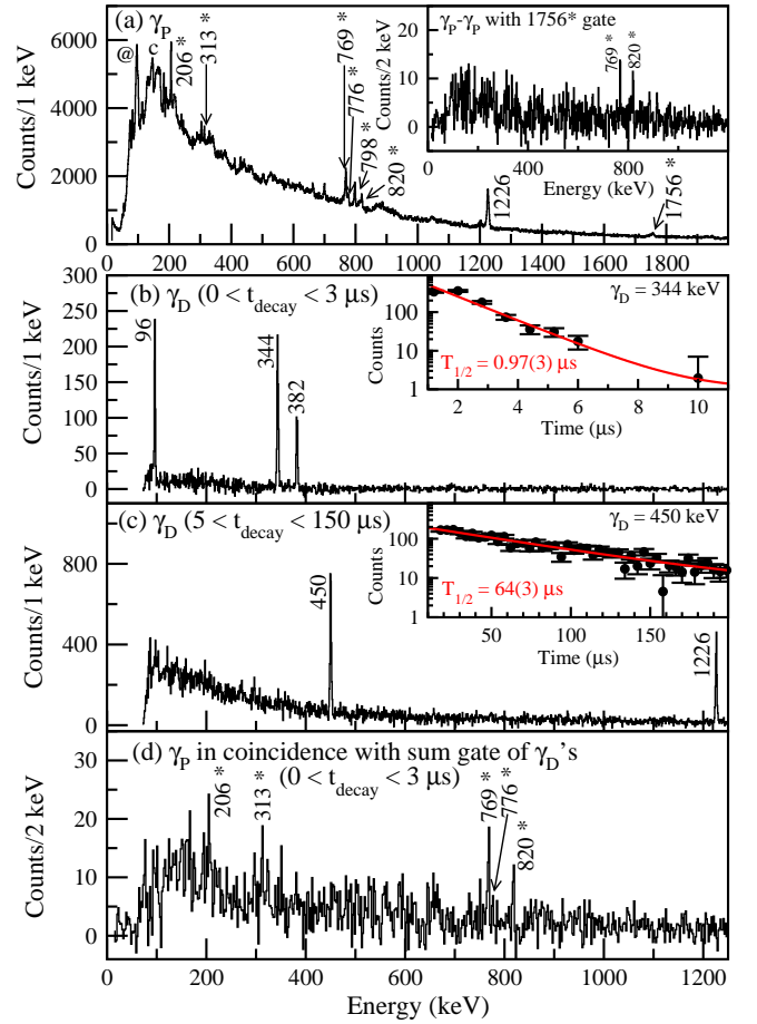
FIG. 11. (Color online) A - and Z -gated \gamma -ray spectra for ^{131}\text{Sb} : The tracked Doppler corrected prompt singles \gamma -ray ( \gamma_P ) spectrum with the new \gamma -ray transitions marked with asterisk. The inset shows the tracked Doppler corrected prompt \gamma_P - \gamma_P coincidence spectrum with gate on the newly identified 1756 keV transition. (b) and (c) The delayed singles \gamma -ray ( \gamma_D ) spectra for 0 < t_{\text{decay}} < 3 \mu\text{s} and 5 < t_{\text{decay}} < 150 \mu\text{s} , respectively. The insets in (b) and (c) shows the decay curves along with the fits for the 344 and 450 keV transitions, respectively. (d) Tracked Doppler corrected \gamma_P in coincidence with the sum gate of the \gamma_D 's, namely 96, 344 and 382 keV delayed transitions (for 0 < t_{\text{decay}} < 3 \mu\text{s} ).
