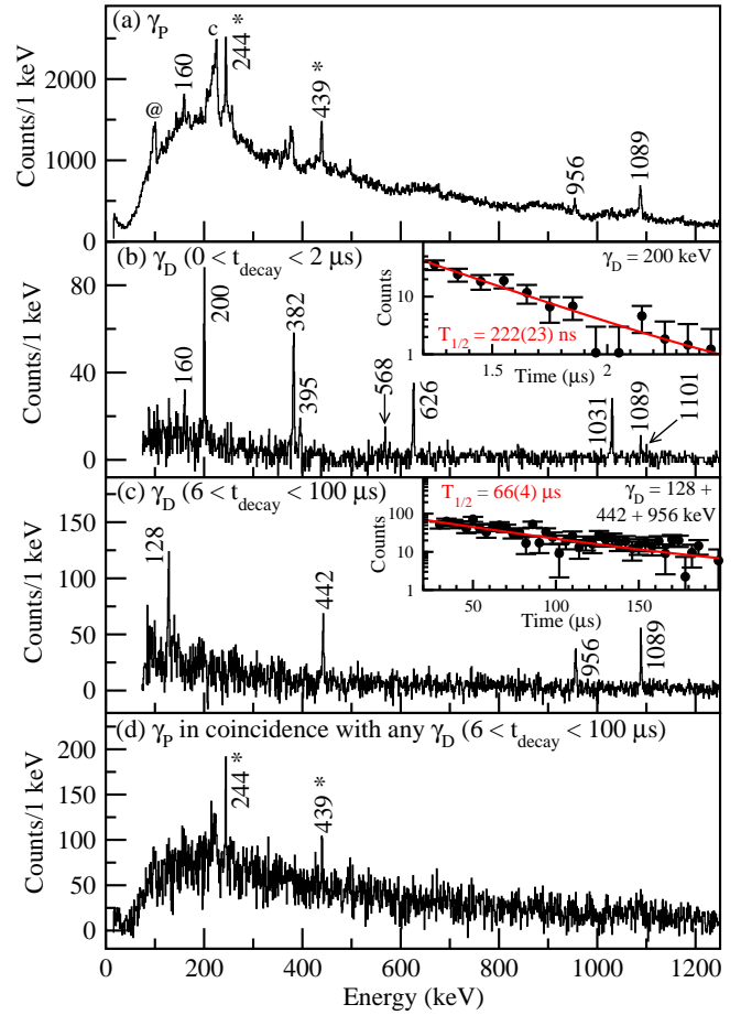
FIG. 3. (Color online) A- and Z- gated \gamma -ray spectra for ^{123}\text{Sb} : (a) The tracked Doppler corrected prompt \gamma -ray ( \gamma_P ) spectrum with the new \gamma -ray transitions marked with asterisk. (b) and (c) The delayed \gamma -ray ( \gamma_D ) spectra for 0 < t_{\text{decay}} < 2 \mu\text{s} and 6 < t_{\text{decay}} < 100 \mu\text{s} , respectively. The insets in (b) and (c) show the decay curves along with the fits for the 200 and 128 + 442 + 956 keV transitions, respectively. (d) \gamma_P in coincidence with any \gamma_D for 6 < t_{\text{decay}} < 100 \mu\text{s} .
