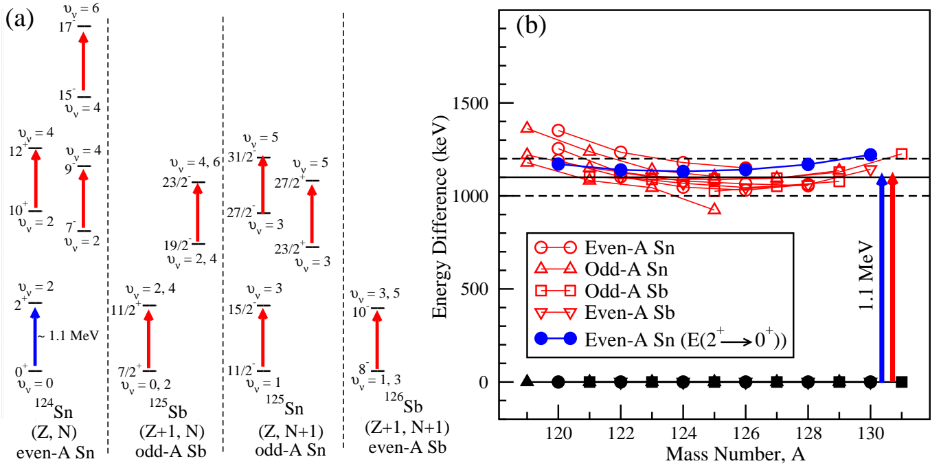
FIG. 18. (Color online) (a) The states with different neutron seniorities at different excitation energies in even-A Sn ( Z, N ) ( ^{124}\text{Sn} ), odd-A Sb ( Z+1, N ) ( ^{125}\text{Sb} ), odd-A Sn ( Z, N+1 ) ( ^{125}\text{Sn} ), and even-A Sb ( Z+1, N+1 ) ( ^{126}\text{Sb} ) isotopes. The blue and red arrows represent the energy required to break the first pair of neutrons from seniority \nu_n = n to \nu_n = n + 2 ( n = 0, \dots, 4 ) in even-A Sn ( E(2^+ \rightarrow 0^+) ) and other isotopes, respectively. (b) Plot of the energy differences between states with neutron seniority \nu_n = n and \nu_n = n + 2 ( n = 0, \dots, 4 ), as shown in (a), for odd-A and even-A ^{119-130}\text{Sn} and ^{121-131}\text{Sb} nuclei.
