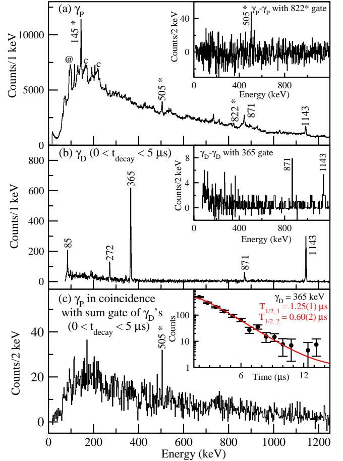
FIG. 10. (Color online) A - and Z -gated \gamma -ray spectra for ^{130}\text{Sb} : (a) Tracked Doppler corrected prompt singles \gamma -ray spectrum ( \gamma_P ). The newly identified prompt \gamma rays are marked with an asterisk. The inset shows the tracked Doppler corrected \gamma_P - \gamma_P coincidence spectrum with gate on the newly identified 822 keV prompt \gamma -ray. (b) The delayed singles \gamma -ray spectrum ( \gamma_D ) for 0 < t_{\text{decay}} < 5 \mu\text{s} . The inset shows the \gamma_D - \gamma_D coincidence spectrum with gate on the delayed 365 keV \gamma -ray. (c) The tracked Doppler corrected \gamma_P in coincidence with the delayed \gamma rays = 365 and 1143 keV transitions, for 0 < t_{\text{decay}} < 5 \mu\text{s} . The newly identified prompt transitions are marked with an asterisk. The inset shows the decay curve along with the two-component fit for the delayed 365 keV transition.
