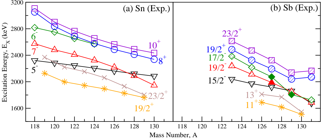
FIG. 13. (Color online) Evolution of the experimental (a) 5^- (black triangle down), 6^- (green diamond), 7^- (red triangle up), 8^+ (blue circle), 10^+ (violet square), 23/2^+ (brown x), and 19/2^+ (orange star) states in ^{118-130}\text{Sn} (open symbols), and (b) 15/2^- (black triangle down), 17/2^- (green diamond), 19/2^- (red triangle up), 19/2^+ (blue circle), 23/2^+ (violet square), 13^+ (brown x), and 11^+ (orange star) states in ^{123-131}\text{Sb} (shaded symbols) with mass number, A . The filled symbols are the newly observed states from the present experiment.
