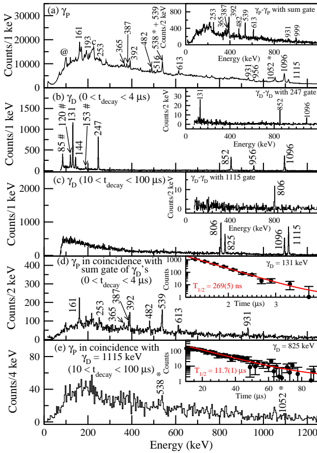
FIG. 7. (Color online) A- and Z-gated \gamma -ray spectra for ^{127}\text{Sb} : (a) The tracked Doppler corrected prompt singles \gamma -ray ( \gamma_P ) spectrum with the new \gamma -ray transitions marked with asterisk. The inset shows the prompt \gamma_P - \gamma_P coincidence spectrum with a sum gate on \gamma_P 's, namely 387, 392, 539 and 613 keV \gamma rays. (b) and (c) The delayed singles \gamma -ray ( \gamma_D ) spectra for 0 < t_{\text{decay}} < 4 \mu\text{s} and 10 < t_{\text{decay}} < 100 \mu\text{s} , respectively. The insets in (b) and (c) shows the delayed \gamma_D - \gamma_D coincidence spectra with gate on 247 and 1115 keV \gamma rays. (d) Tracked Doppler corrected \gamma_P in coincidence with the sum gate of the \gamma_D 's, namely 85, 120, 131, 144, 247, 852, 956 and 1096 keV \gamma rays (for 0 < t_{\text{decay}} < 4 \mu\text{s} ). The inset shows the decay curve along with the fit for the 131 keV transition. (e) Tracked Doppler corrected \gamma_P in coincidence with the \gamma_D = 1115 keV \gamma -ray (for 10 < t_{\text{decay}} < 100 \mu\text{s} ). The inset shows the decay curve along with the fit for the 825 keV transition.
