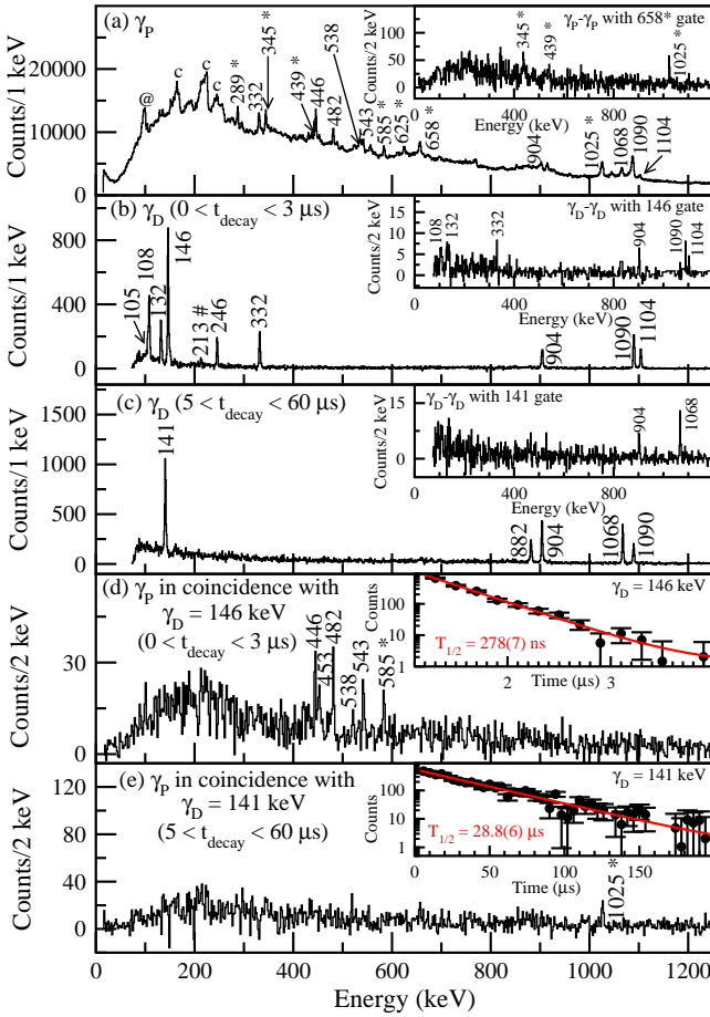
FIG. 5. (Color online) A- and Z- gated \gamma -ray spectra for ^{125}\text{Sb} : (a) The tracked Doppler corrected prompt singles \gamma -ray ( \gamma_P ) spectrum with the new \gamma -ray transitions marked with asterisk. The inset shows the tracked Doppler corrected prompt \gamma_P - \gamma_P coincidence spectrum with gate on the newly observed 658 keV \gamma -ray (b) and (c) The delayed singles \gamma -ray ( \gamma_D ) spectra for 0 < t_{\text{decay}} < 3 \mu\text{s} and 5 < t_{\text{decay}} < 60 \mu\text{s} , respectively. The insets in (b) and (c) shows the delayed \gamma_D - \gamma_D coincidence spectra with gate on 146 and 141 keV \gamma rays, respectively. (d) Tracked Doppler corrected \gamma_P in coincidence with \gamma_D = 146 keV \gamma -ray (for 0 < t_{\text{decay}} < 3 \mu\text{s} ). The inset shows the decay curve along with the fit for the 146 keV transition. (e) \gamma_P in coincidence with the \gamma_D = 141 keV \gamma -ray (for 5 < t_{\text{decay}} < 60 \mu\text{s} ). The inset shows the decay curve along with the fit for the 141 keV transition.
