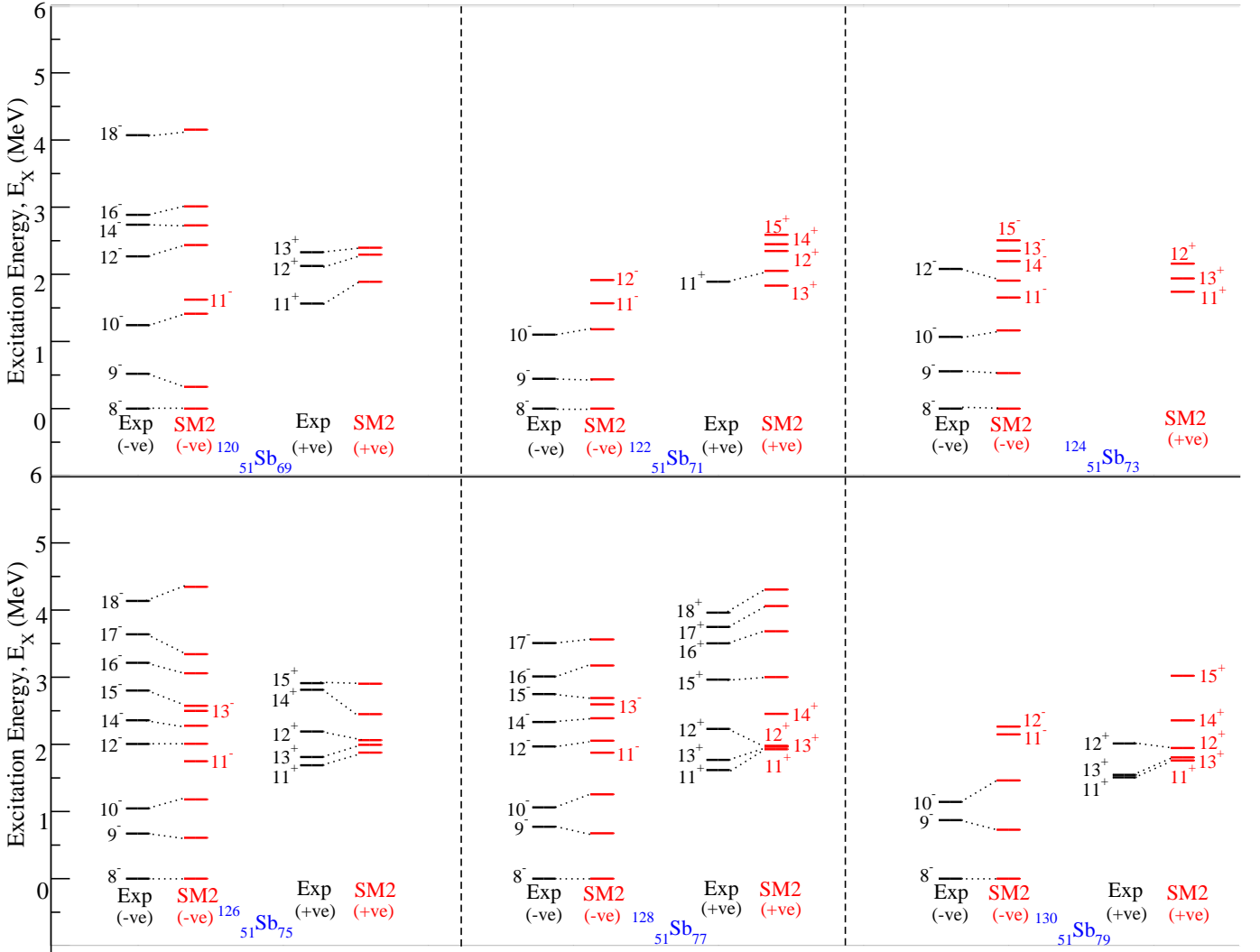
FIG. 16. (Color online) Comparison of experimental (Exp.) (shown in black) [6, 35, 36, 43, 45] and theoretical calculations (from shell model (SM2)) (shown in red) level schemes for even-A ^{122-130}\text{Sb} isotopes for both positive (+ve) and negative (-ve) parities. The experimental and shell model states of the same spin-parity are joined with dotted lines to show the agreement.
