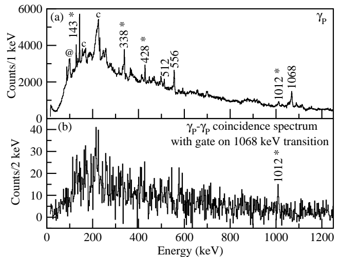
FIG. 4. A- and Z-gated \gamma -ray spectra for ^{124}\text{Sb} : (a) The tracked Doppler corrected prompt \gamma -ray ( \gamma_P ) singles spectrum. (b) The prompt \gamma - \gamma ( \gamma_P - \gamma_P ) spectrum with gate on 1068 keV transition. The newly identified prompt transitions are marked with an asterisk.
