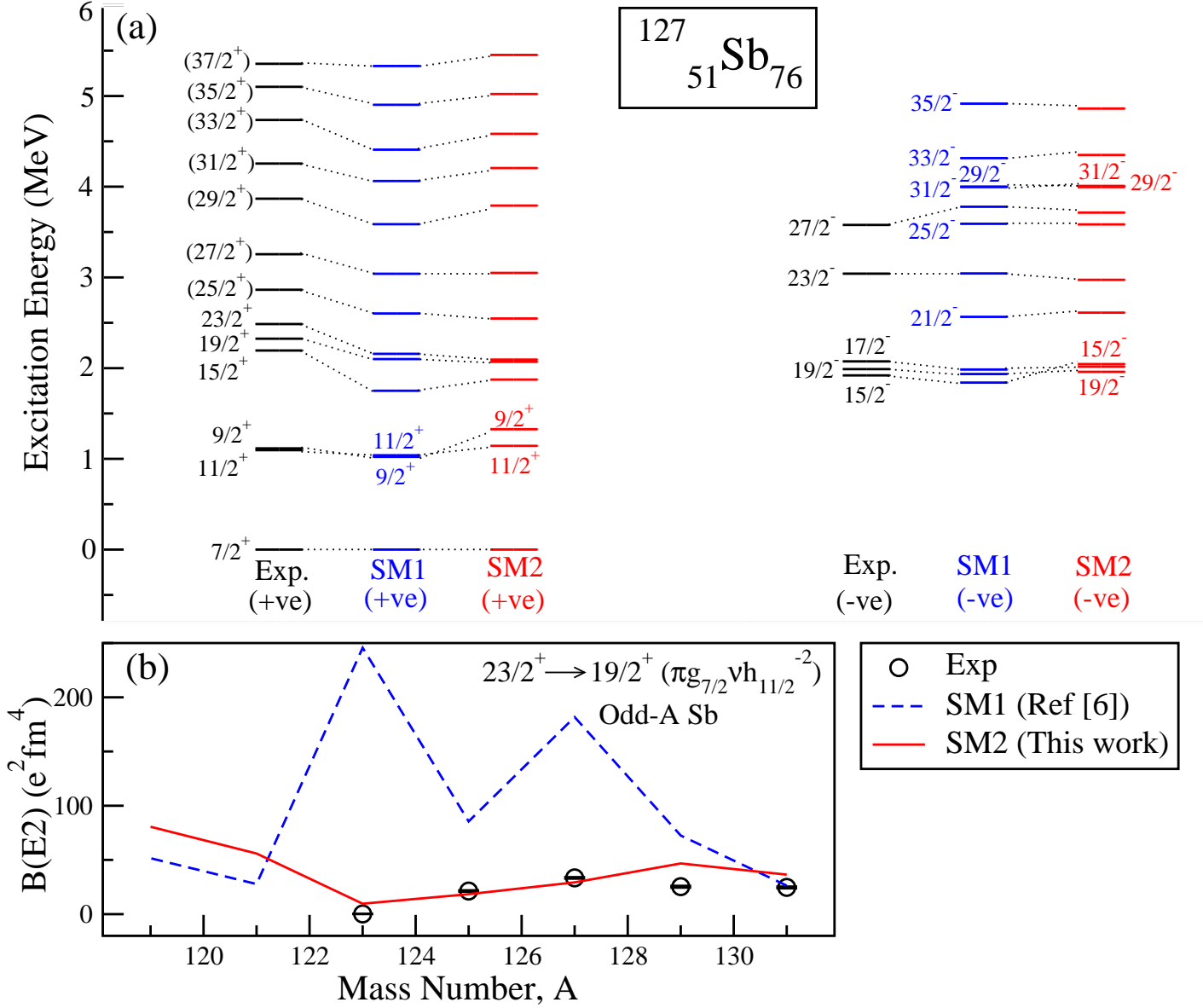
FIG. 14. (Color online) (a) Comparison of the experimental level schemes with that obtained from shell model calculations using the interaction in Ref. [6] (SM1 blue) and the modified interaction in the present work (SM2 red) for both positive and negative-parity states in ^{127}\text{Sb} . The different states with the same spin have been joined by dotted lines to show the agreement. (b) The experimental and calculated B(E2) values (black square) for the 23/2^+ \rightarrow 19/2^+ in odd-A ^{123-131}\text{Sb} (see text).
