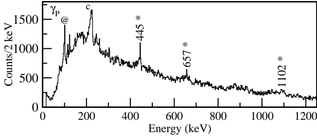
FIG. 2. A- and Z- gated \gamma -ray spectrum for ^{122}\text{Sb} : The tracked Doppler corrected prompt singles \gamma -ray ( \gamma_P ) spectrum. The newly identified \gamma rays are marked with an asterisk.
