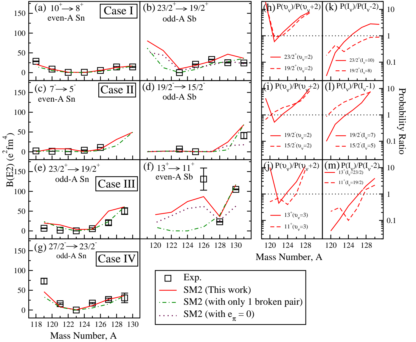
FIG. 17. (Color online) The experimental B(E2) values (black square) for the (a) 10^+ \rightarrow 8^+ in even- A ^{118-130}\text{Sn} [16, 21, 46], (b) 23/2^+ \rightarrow 19/2^+ in odd- A ^{123-131}\text{Sb} (see text) (c) 7^- \rightarrow 5^- in even- A ^{118-126}\text{Sn} [21], (d) 19/2^- \rightarrow 15/2^- transitions in odd- A ^{123-131}\text{Sb} (see text), (e) 23/2^+ \rightarrow 19/2^+ in odd- A ^{119-129}\text{Sn} [20, 21], (f) 13^+ and 11^+ states in the even- A ^{126-130}\text{Sb} (see text), and (g) 27/2^- \rightarrow 23/2^- in odd- A ^{119-129}\text{Sn} isotopes [20, 21, 47]. The shell model calculations using the full interaction SM2 (red solid line), SM2 restricted to only one broken neutron pair (green dash-dotted line) and SM2 with e_\pi = 0 (purple dotted line) are also shown. The probability ratios for the (h-j) neutron seniority mixing ( (P(v_\nu)/P(v_\nu+2)) ) and (k-m) neutron-angular momentum mixing ( (P(I_\nu)/P(I_\nu-2)) ) and ( (P(I_\nu)/P(I_\nu-1)) ) are also shown.
