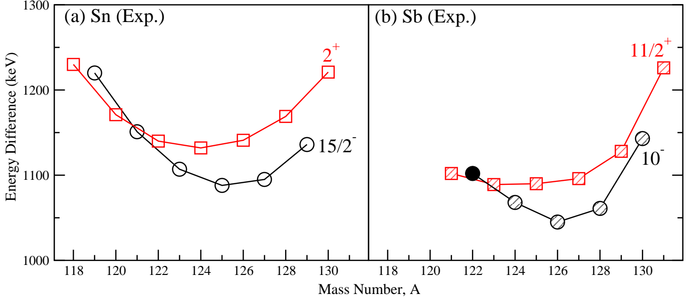
FIG. 12. (Color online) Evolution of the experimental energy differences, as a function of mass number, in Sn (open symbols) (a) E(2^+) - E(0^+) (red square), E(15/2^-) - E(11/2^-) (black circle), and in Sb (shaded symbols) (b) E(11/2^+) - E(7/2^+) (red square), E(10^-) - E(8^-) (black circle). The filled symbol is the newly observed state from the present experiment.
