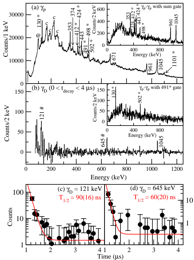
FIG. 6. (Color online) A - and Z -gated \gamma -ray spectra for ^{126}\text{Sb} : (a) Tracked Doppler corrected Prompt \gamma -ray singles spectrum ( \gamma_P ). The inset shows the tracked Doppler corrected \gamma_P - \gamma_P coincidence spectrum with sum gate on \gamma_P 's, namely the 353, 443 and 961 keV transitions. The newly identified prompt \gamma rays are marked with an asterisk. (b) The delayed singles \gamma -ray spectrum ( \gamma_D ) for 0 < t_{\text{decay}} < 4 \mu\text{s} . The newly identified delayed \gamma rays are marked with hash. The inset shows the tracked Doppler corrected \gamma_P - \gamma_P coincidence spectrum with gate on the newly identified 491 keV prompt \gamma -ray. (c) and (d) The decay curve along with the fit for the delayed 121 and 645 keV transitions, respectively.
