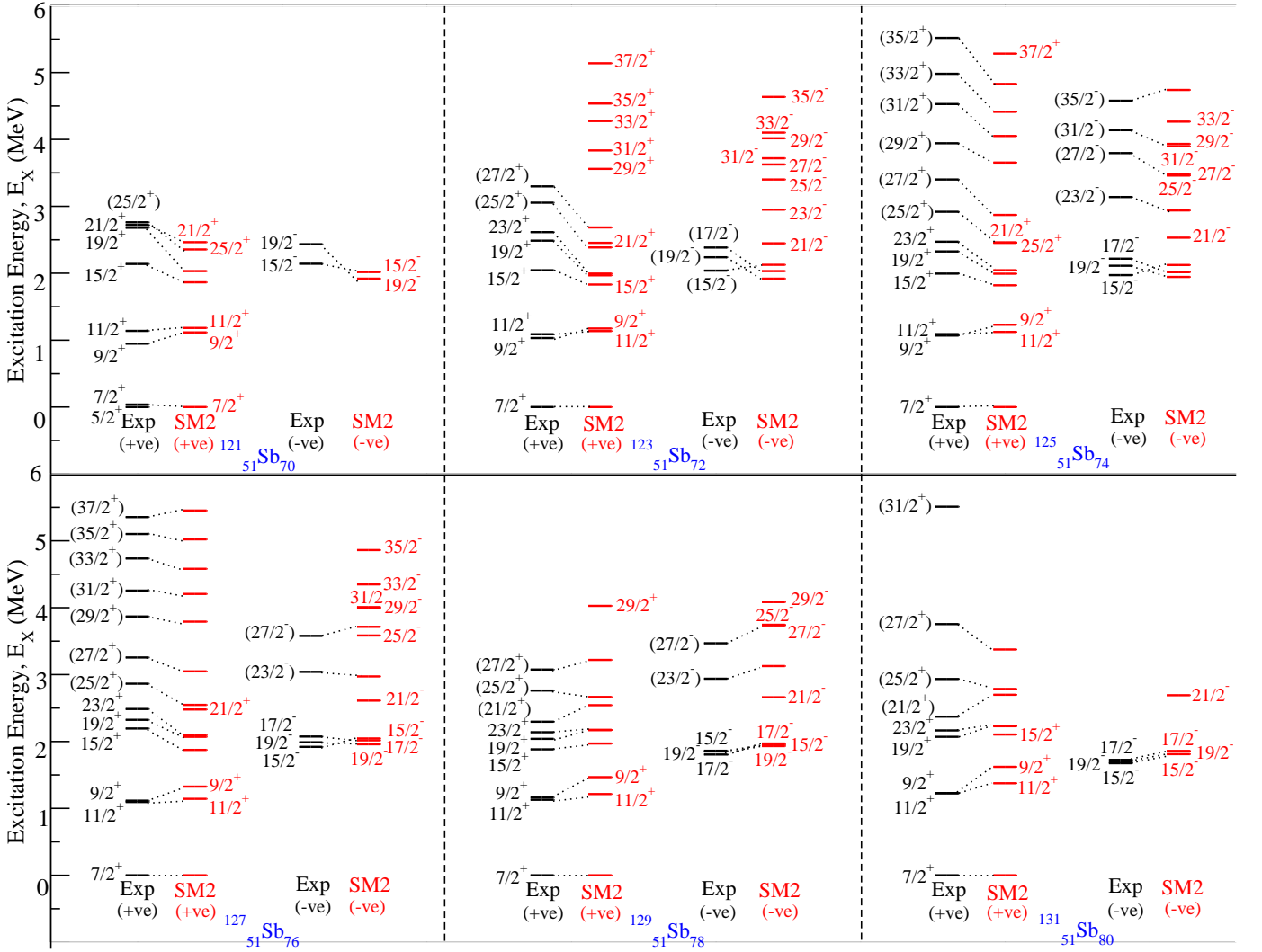
FIG. 15. (Color online) Comparison of experimental (Exp.) (shown in black) [22–26] and theoretical calculations (from shell model (SM2)) (shown in red) level schemes for odd-A ^{121-131}\text{Sb} isotopes for both positive (+ve) and negative (-ve) parities. The experimental and shell model states of the same spin-parity have been joined with dotted lines to show the agreement.
