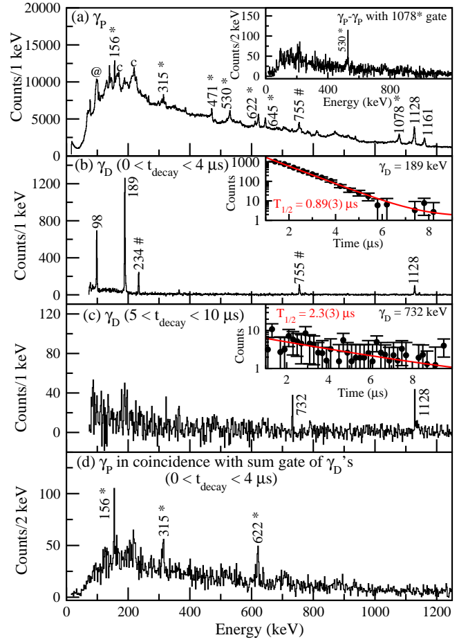
FIG. 9. (Color online) A - and Z -gated \gamma -ray spectra for ^{129}\text{Sb} : (a) The tracked Doppler corrected prompt singles \gamma -ray ( \gamma_P ) spectrum with the new \gamma -ray transitions marked with asterisk. The inset shows the tracked Doppler corrected prompt \gamma_P - \gamma_P coincidence spectrum with gate on the newly identified 1078 keV transition. (b) and (c) The delayed singles \gamma -ray ( \gamma_D ) spectra for 0 < t_{decay} < 4 \mu\text{s} and 5 < t_{decay} < 10 \mu\text{s} , respectively. The insets in (b) and (c) shows the decay curves along with the fits for the 189 and 732 keV transitions, respectively. (d) Tracked Doppler corrected \gamma_P in coincidence with the sum gate of the \gamma_D 's, namely 98, 189, 234 and 755 keV delayed transitions (for 0 < t_{decay} < 4 \mu\text{s} ).
