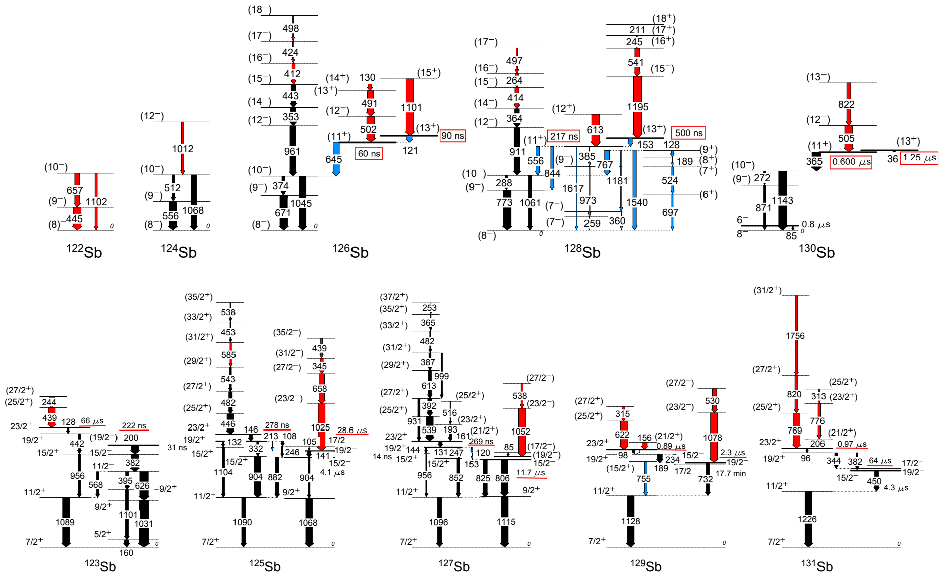
FIG. 1. (Color online) The level schemes of ^{122}\text{--}^{131}\text{Sb} . The newly observed \gamma -ray transitions above and below the isomer are indicated in red and blue, respectively. The width of the arrows represent the intensity of the transitions. The isomeric states are indicated by a thick line. The previously known half-lives but remeasured in this work have been underlined by a red line, whereas the newly measured half-lives have been marked with a red box. The half-lives not measured in this work are also shown.
