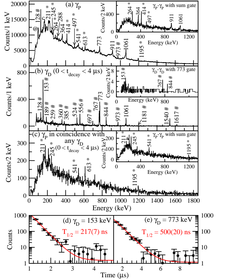
FIG. 8. (Color online) A- and Z- gated \gamma -ray spectra for ^{128}\text{Sb} : (a) Tracked Doppler corrected Prompt singles \gamma -ray spectrum ( \gamma_P ). The newly identified prompt and delayed \gamma rays are marked with an asterisk and hash, respectively. The inset shows the \gamma_P - \gamma_P coincidence spectrum with sum gate on the \gamma_P 's, namely the 264, 364 and 414 keV transitions. (b) The delayed singles \gamma -ray spectrum ( \gamma_D ) for 0 < t_{\text{decay}} < 4 \mu\text{s} . The newly identified delayed \gamma rays are marked with hash. The inset shows the \gamma_D - \gamma_D coincidence spectrum with gate on the delayed 773 keV \gamma -ray. (c) The \gamma_P in coincidence with any delayed \gamma -ray for 0 < t_{\text{decay}} < 4 \mu\text{s} . Again, the newly identified prompt transitions are marked with an asterisk. The inset shows the \gamma_P - \gamma_P coincidence spectrum with sum gate on many \gamma_P 's, namely the 541 and 1195 keV transitions. (d) and (e) shows the decay curves along with the fits for the delayed 153 and 773 keV transitions, respectively.
