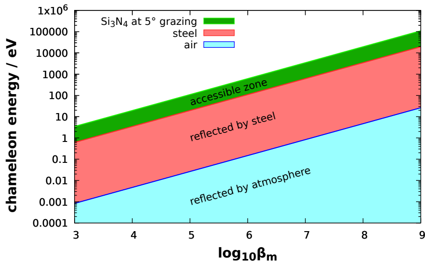
Figure 6: The accessible chameleon energy range with the present setup. Only chameleons with masses in the green band between the red and green lines contribute to the radiation pressure on the KWISP sensor.
