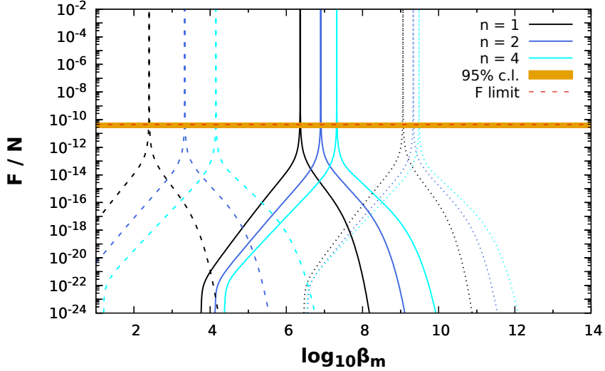
Figure 11: Expected force at the sensor calculated from the solar chameleon flux assuming \beta_\gamma = 10^{10.32} , interaction zone length L_i = 0.05 \cdot R_{Sun} and detector parameters. Solid lines correspond to a dark energy scale \Lambda = 2.4 \cdot 10^{-3} eV, dashed ones to \Lambda = 1 \cdot 10^{-5} eV, and dotted lines to \Lambda = 0.1 eV. The interaction zone length is an upper limit according to current Solar models. The flux and consequently the expected force are scaled accordingly for values down to L_i = 0.01 \cdot R_{Sun} while the resonance peak is arbitrarily limited to F = 10^{-2} N by the axis scale. The orange band represents 95% confidence interval centred at the average force value shown by the red dashed line.
