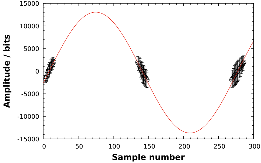
Figure 9: Calibration graph showing the result of the sine fit. The data points were fitted with the function I(x) = A \cdot \sin(\omega \cdot x + b) + B and the values A = (133 \pm 4) \cdot 10^2 , B = -324 \pm 64 , \omega = 0.02336 \pm 4 , \varphi = -0.178 \pm 6 were derived.
