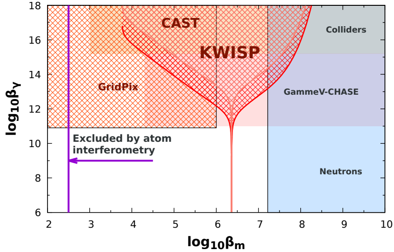
Figure 12: The exclusion limit for Chameleons at CAST are shown with hatched pattern. The KWISP measurement of this work is illustrated in red colour and comparison to other experimental techniques ([19, 20, 21, 22]) is made, assuming a dark energy scale \Lambda = 2.4 \cdot 10^{-3} eV and n = 1 . The limit from the previous CAST measurement [17] is based on chameleon-to-photon conversion only. In the parameter space of realistic solar models the expected chameleon production maximum, in darker shade, takes place for B = 30 T and the tachocline length L_i = 0.05 R_{Sun} while the minimum, in lighter shade, is expected for B = 10 T and the tachocline length L_i = 0.01 R_{Sun} .
