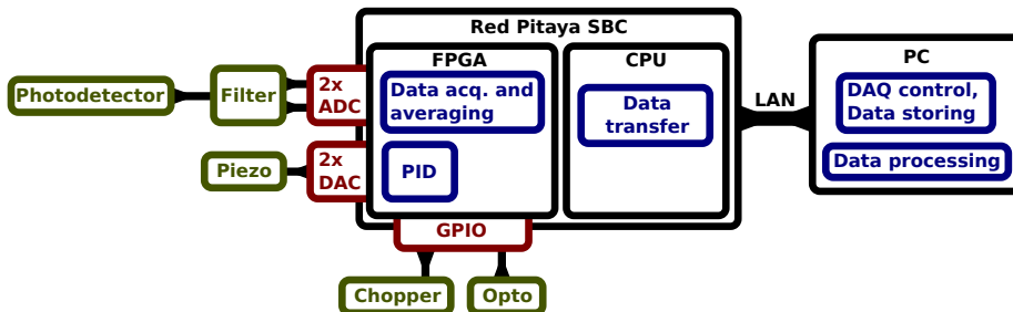
Figure 2: DAQ block schematic.
