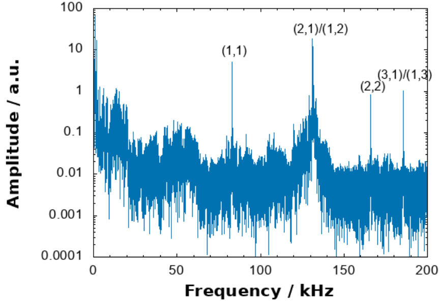
Figure 7: Background noise spectrum taken in the laboratory with a the 5 \times 5 \text{ mm}^2 , 100 nm thick membrane. The mechanical vibration peaks can be distinguished from background since their frequencies have well defined ratios (see Table 1). Integration time was 9 s with an input beam intensity of 5.0 mW (see also text).
