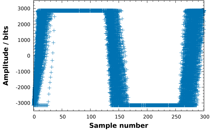
Figure 8: Calibration graph. Overlay of the cycles used for calibration. Only the first 532 nm of OPL change are used.
