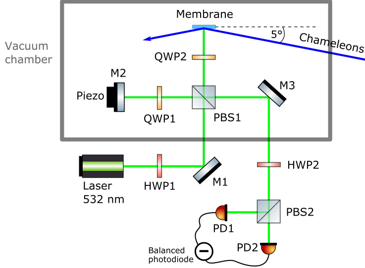
Figure 1: Schematic layout of the the optical setup (see text).
