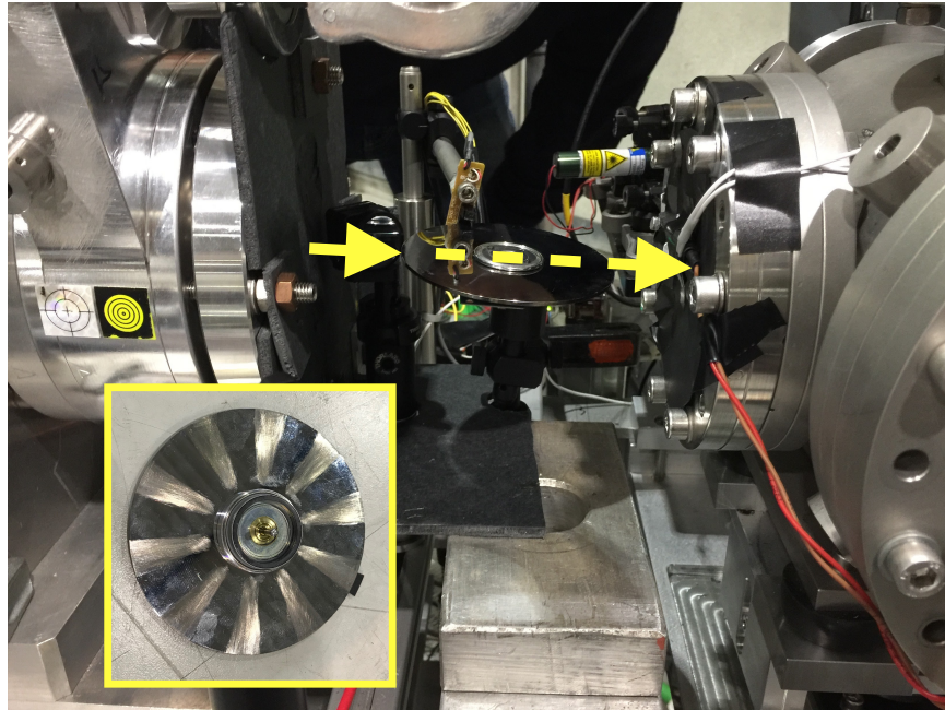
Figure 5: The chopper disk mounted between the vacuum chamber (at right) and the telescope (at left). In the photograph the chameleon beam comes from the left hand side, as indicated by the arrows. The segmented surface of the disk faces downwards and it is illustrated in the framed inset.
