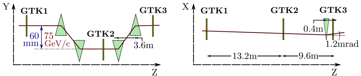
Figure 2. Schematic view of the GTK. The green triangles represent bending magnets. The beam is deflected by 1.2 \text{ mrad} in the XZ plane to compensate the effect of the STRAW spectrometer dipole magnet.
