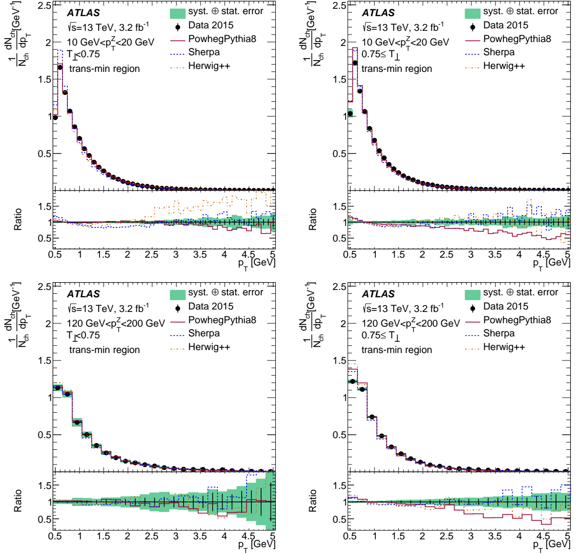
Figure 6: Measured p_T spectra in the trans-min region for T_\perp < 0.75 (left) and 0.75 \leq T_\perp (right) for events with 10 < p_T^Z < 20 GeV (upper row) and 120 < p_T^Z < 200 GeV (lower row). Predictions of POWHEG+PYTHIA, SHERPA, and Herwig++ are compared with the data. The ratios shown are predictions over data.
