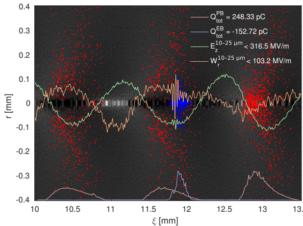
Figure 2: Loading of the field after \approx 1.1 m of plasma for a 400 \text{ A}/60 \mu\text{m} electron beam. A sample of electrons (blue) and protons (red) are plotted with their respective projection at the bottom. The total charge within the region of the plot is given as the first two lines of the legend. The longitudinal e-field E_z is shown in green. The transverse wakefield W_r = E_r - v_z B_\theta is shown in orange, where v_z = c is the moving frame of the simulation. The fields are averages over 15 \mu\text{m} near the axis.
