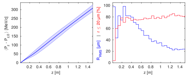
Figure 4: The 400 \text{ A}/60 \mu\text{m} electron beam as it travels through plasma. The left plot shows the mean energy of the beam with the RMS energy spread as a shaded bar. The right plot shows the RMS radius in blue, and the percentage of macro particles the are within 20 \mu\text{m} of the axis in red.
