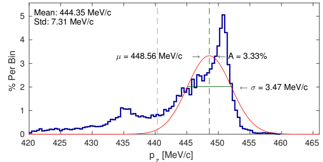
Figure 3: Electron beam momentum spread after \approx 1.1 m of plasma for the 400 \text{ A}/60 \mu\text{m} beam. 75 % of the beam charge is accelerated to more than 440 \text{ MeV/c} , the vertical grey line. The fit is applied to the data above this line, R^2 = 0.755 .
