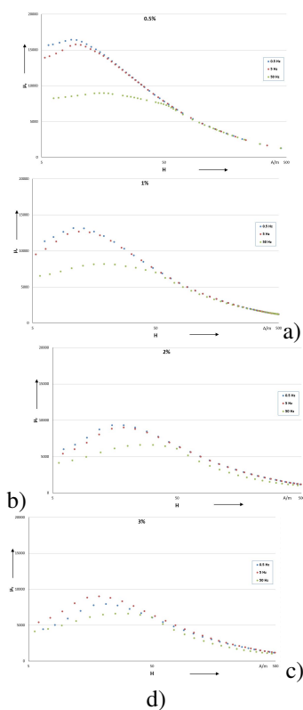
Figure 9: Magnetic permeability of strained Cryophy for varying frequencies, a) 0.5%; b) 1%; c) 2%; d) 3%.
