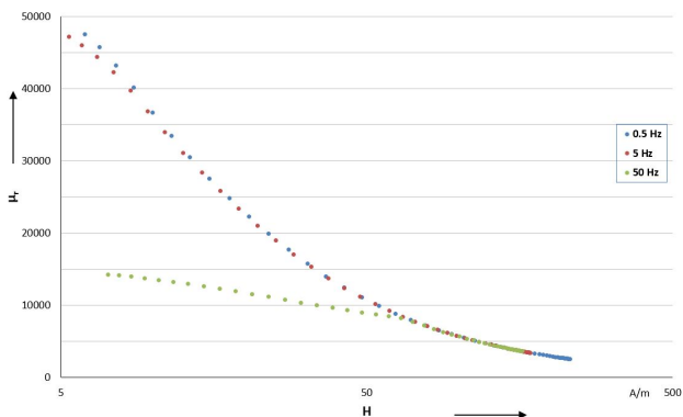
Figure 8: Magnetic permeability of Cryophy for varying frequencies.
