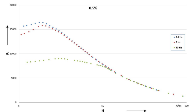
Figure 7: Magnetic permeability of Cryophy for varying strain states.
