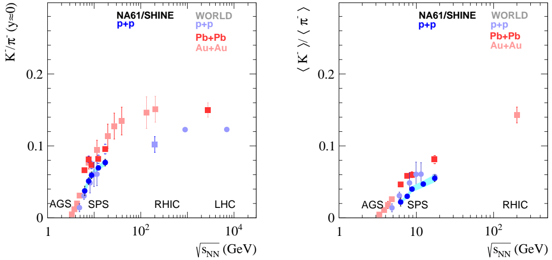
Figure 2: Energy dependence of the K^-/\pi^- ratio at mid-rapidity ( left ) and in the full phase-space ( right ). The NA61/SHINE results for inelastic p+p interactions are shown together with the world data on p+p interactions as well as central Pb+Pb and Au+Au collisions [21, 23, 25–38]. Shaded bands show the systematic uncertainty.
