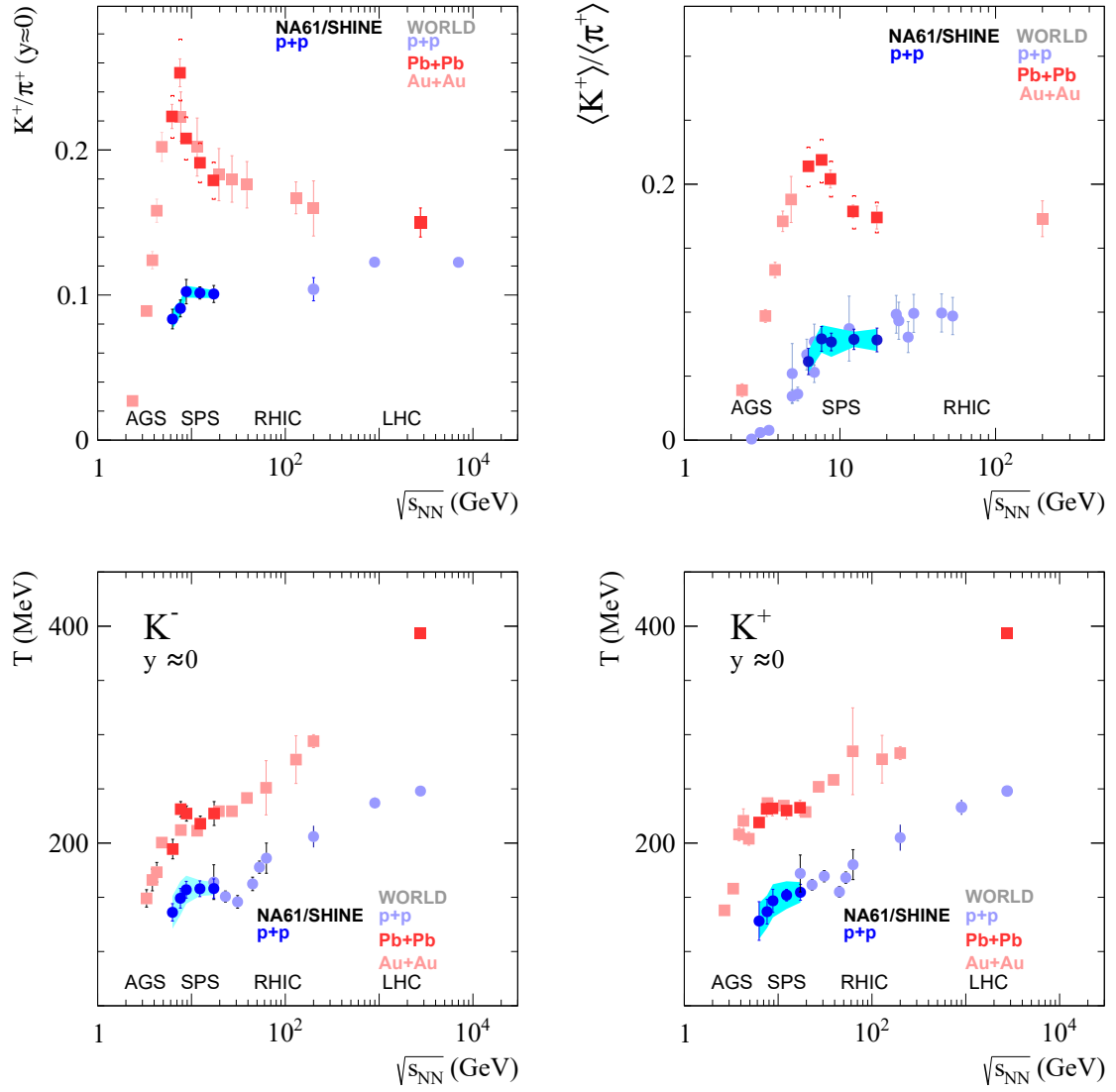
Figure 1: Energy dependence of the K^+/\pi^+ ratio at mid-rapidity ( top-left ) and in the full phase-space ( top-right ) as well as the inverse slope parameter T of transverse mass spectra at mid-rapidity for K^- ( bottom-left ) and K^+ ( bottom-right ) mesons. The NA61/SHINE results for inelastic p+p interactions are shown together with the world data on p+p interactions as well as central Pb+Pb and Au+Au collisions [21, 23, 25–38]. Shaded bands show the systematic uncertainty.
