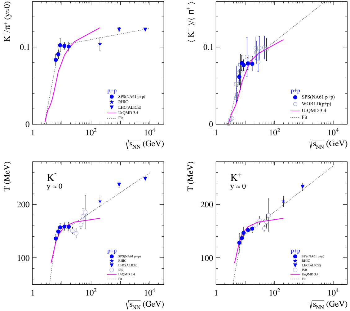
Figure 3: Energy dependence of the K^+/\pi^+ ratio in inelastic p+p interactions at mid-rapidity ( top-left ) and in the full phase-space ( top-right ) as well the inverse slope parameter T of transverse mass spectra at mid-rapidity for K^- ( bottom-left ) and K^+ ( bottom-right ) mesons. The data are fitted by two straight lines in order to locate a position of the break in the energy dependence. The experimental results are compared with predictions of the resonance-string model, UrQMD [41].
