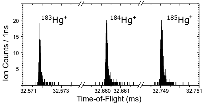
FIG. 6. Time-of-Flight spectra obtained for ^{183-185}\text{Hg} , when the GPS mass separator was set to A = 183, A = 184, A = 185 respectively, after 1000 revolutions in the MR-ToF MS at which a mass resolving power of about 1.2 \times 10^5 was reached. At this resolving power, all isotopic and isobaric contaminants are cleared from the spectra.
