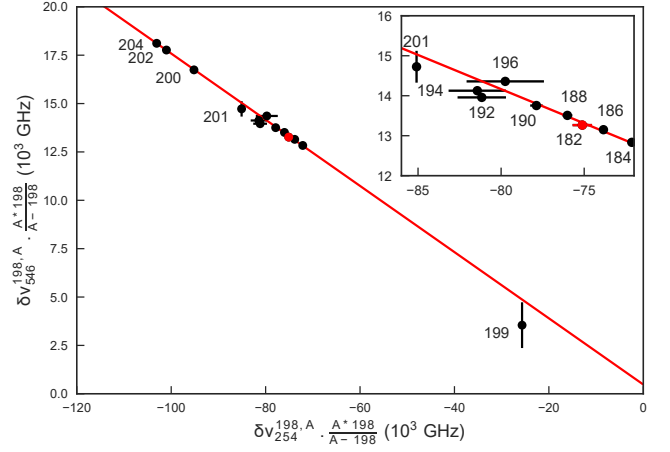
FIG. 8. King plot of the modified isotope shifts in the 546-nm line versus those in the 254-nm line with 198 Hg as reference isotope. Inset: zoom around the area of the plot where most of the points are clustered. The new data point for 182 Hg fits well to the King-plot line from [4].
