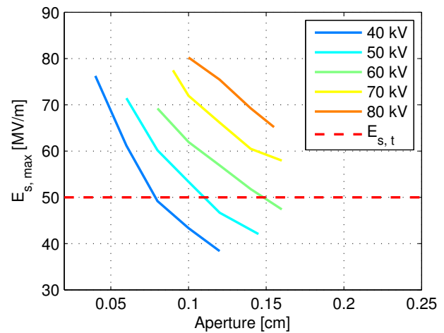
Figure 2: Parametric scan of the inter-vane voltage as a function of the input minimum aperture between the vane and the resulting maximum surface field in the RFQ.
