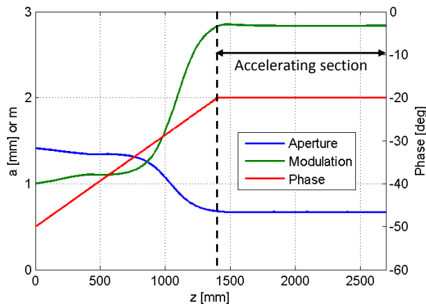
Figure 3: Phase, aperture and modulation along the RFQ.
