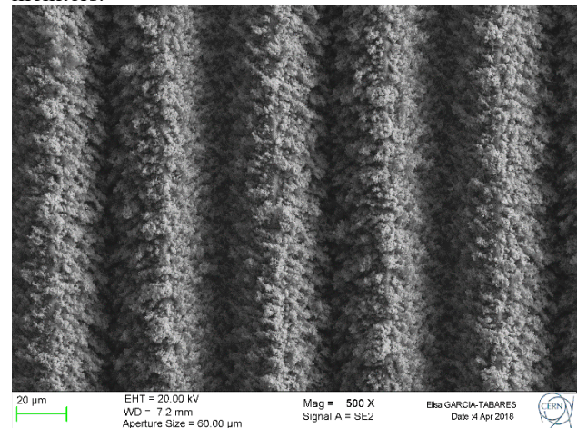
Figure 2: Top view of LESS treated surface.
