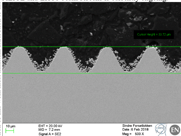
Figure 3: Cross-section of LESS treated surface.
