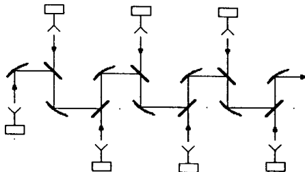
Figure 14: The simplest scheme of quasi-optical RF power summator
