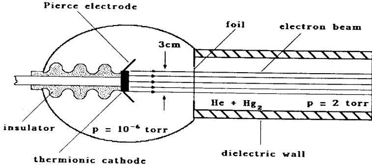
Figure 9: Microwave deflector
