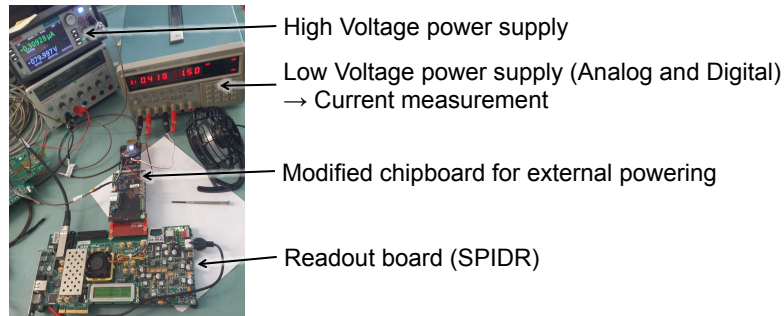
Figure 3: Laboratory setup for the power consumption measurements.
