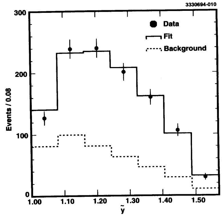
FIG. 11. Differential yield, dN/d\tilde{y} , for B^- \rightarrow D^{*0} \ell^- \bar{\nu} events and \bar{B}^0 \rightarrow D^{*+} \ell^- \bar{\nu} events combined with the projection of the unbinned simultaneous fit superimposed. The solid histogram represents the result of the fit using \mathcal{F}(y) = 1 - a^2(y - 1) . The dashed histogram shows the sum of the background levels.
