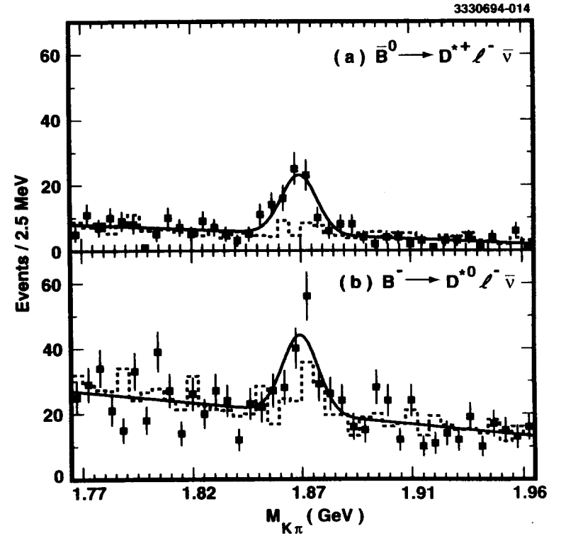
FIG. 5. Invariant mass of K^- \pi^+ combinations passing a \delta_m cut in the Correlated Background Region of the decay modes (a) \bar{B}^0 \rightarrow D^{*+} \ell^- \bar{\nu} and (b) B^- \rightarrow D^{*0} \ell^- \bar{\nu} . The dashed histograms show the scaled M_{K\pi} distributions of events in the \delta_m sideband. The solid lines show the fits used to determine the yields.
