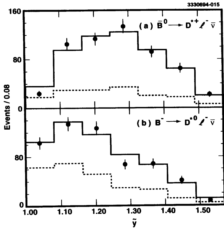
FIG. 10. Differential yield, dN/d\tilde{y} , for (a) \bar{B}^0 \rightarrow D^{*+} \ell^- \bar{\nu} events and (b) B^- \rightarrow D^{*0} \ell^- \bar{\nu} events in the data, with the projections of the unbinned fits superimposed. The solid histogram represents the result of the fit using \mathcal{F}(y) = 1 - a^2(y - 1) . The dashed histogram shows the level of the background from all sources.
