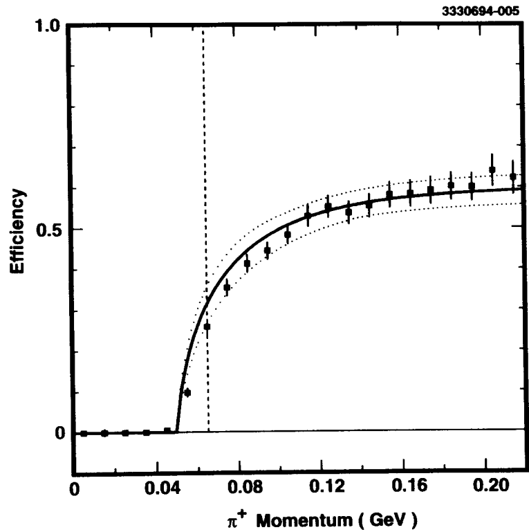
FIG. 6. Monte Carlo reconstruction efficiency versus momentum (filled diamonds) for charged slow pion candidates. Overlaid (solid curve) is the efficiency as determined from the inclusive D^{*+} decay angle distribution in data. The 1\sigma variations in the parameters of this curve are shown by the dotted lines. The dashed line indicates the minimum momentum cut used in this analysis. The efficiency shown here includes the geometric acceptance of 71%.
