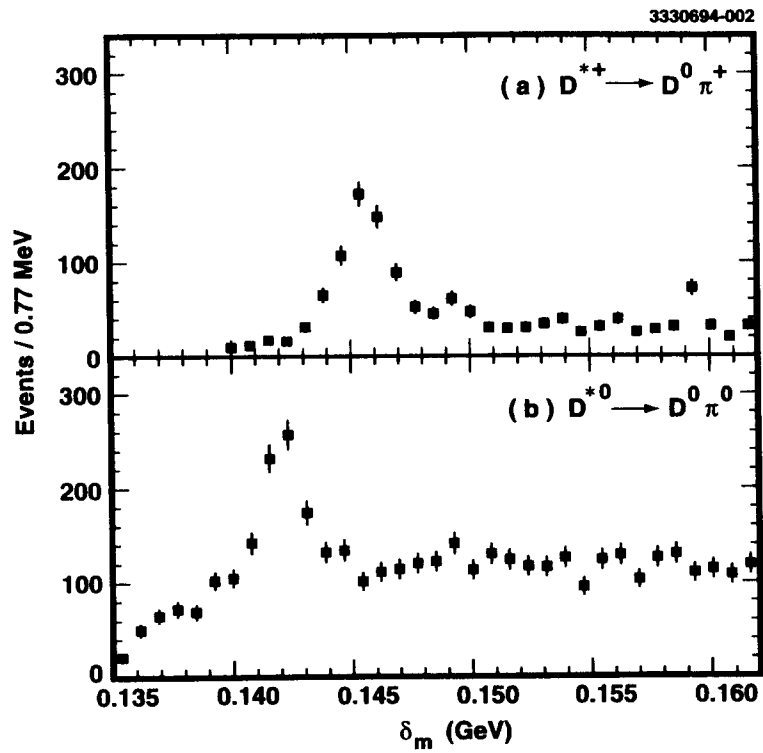
FIG. 2. Mass difference ( \delta_m ) distributions of events falling in the Signal Region of the decay modes (a) \bar{B}^0 \rightarrow D^{*+} \ell^- \bar{\nu} and (b) B^- \rightarrow D^{*0} \ell^- \bar{\nu} . All candidates are required to have M_{K\pi} within 100 MeV of the measured D^0 mass.
