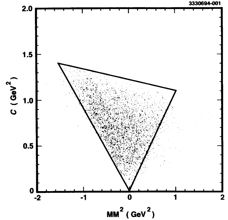
FIG. 1. Kinematic boundary for \bar{B} \rightarrow D^* \ell \bar{\nu} decays in the plane of C vs. MM^2 , for lepton momentum in the range 1.4 < |\mathbf{p}_\ell| < 2.4 GeV (solid line). This is the Signal Region for this analysis. The dots, including those outside the kinematic boundary, are Monte Carlo signal events. Final state radiation and bremsstrahlung occasionally force reconstructed events outside of the kinematic boundary.
