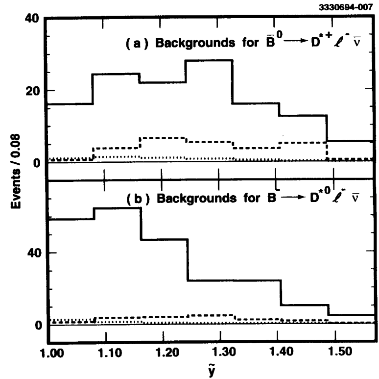
FIG. 9. The \tilde{y} distributions of the backgrounds for (a) \bar{B}^0 \rightarrow D^{*+} \ell^- \bar{\nu} events and for (b) B^- \rightarrow D^{*0} \ell^- \bar{\nu} events. The solid line is the combinatoric background, the dashed line is the correlated background, and the dotted line is the uncorrelated background. The area of the curves are normalized to represent the background levels in the data.
