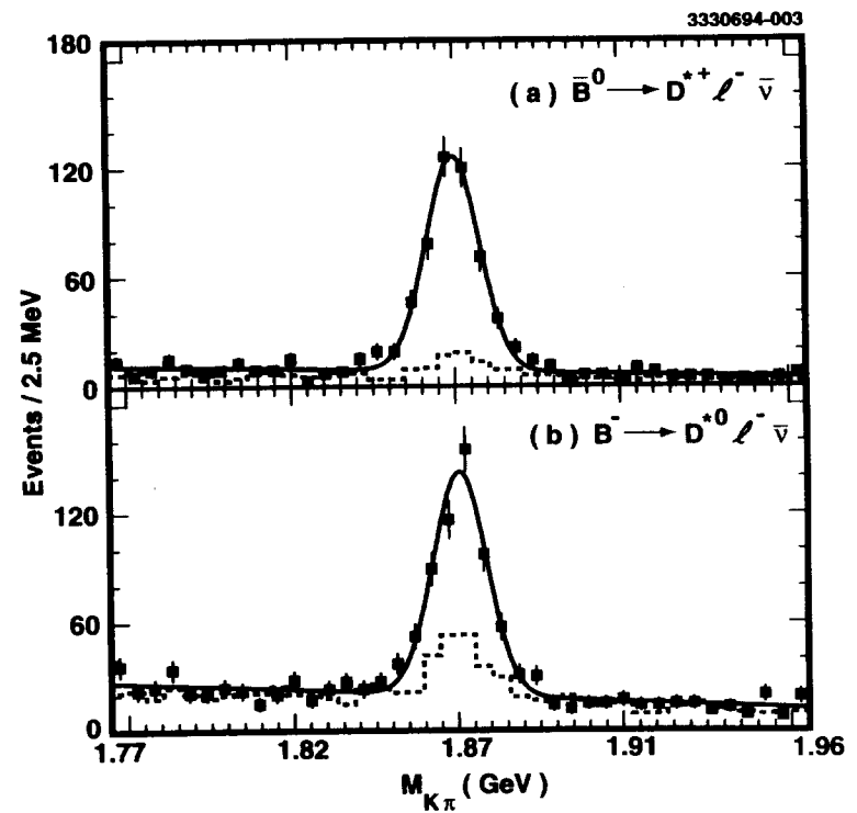
FIG. 3. Invariant mass of K^-\pi^+ combinations passing a \delta_m cut in the Signal Region of the decay modes (a) \bar{B}^0 \rightarrow D^{*+} \ell^- \bar{\nu} and (b) B^- \rightarrow D^{*0} \ell^- \bar{\nu} . The dashed histograms show the scaled M_{K\pi} distributions of events in the Signal Region, but in the \delta_m sideband. The solid lines show the fits used to determine the yields.
