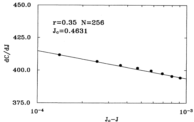
FIG. 13. The derivative of the specific heat dC/dJ as a function of J_c - J on semilogarithmic axes for N = 256 .
