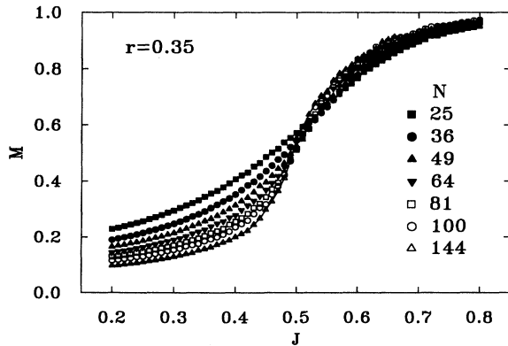
FIG. 9. The magnetization M versus J , for fixed hard-core repulsion parameter r = 0.35 and different system sizes. The solid line is a spline through the data for N = 144 .
