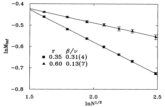
FIG. 10. Finite-size scaling of the magnetization at the inflection point M_{\text{inf}} versus the total number of Ising spins, N , for choices of the hard-core repulsion parameter corresponding to r = 0.35 and r = 0.6 .
