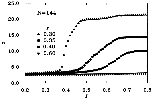
FIG. 4. The average number of neighbors z as a function of J on a lattice with N = 144 spins for several choices of the hard-core repulsion r .
