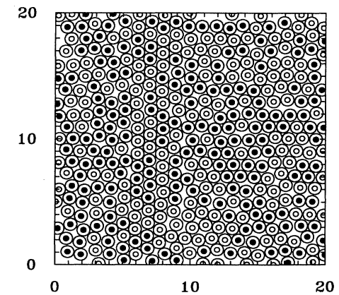
FIG. 3. A particular configuration of the system with N = 400 spins and r = 0.98 for J = 0.25 . The hard-core repulsion radius is shown as a circle around the spin. Spins with S = \pm 1 are indicated with open and solid circles, respectively.
