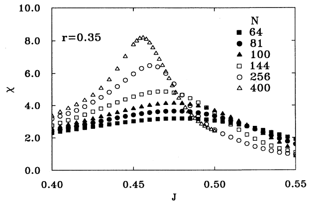
FIG. 7. The magnetic susceptibility \chi versus J for fixed hard-core repulsion parameter r = 0.35 and different system sizes.
