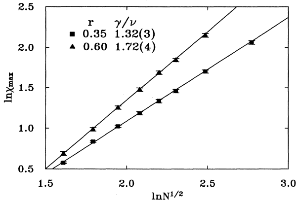
FIG. 8. The peak in the magnetic susceptibility \chi_{\max} versus the number of Ising spins N for choices of the hard-core repulsion parameter corresponding to r = 0.35 and r = 0.6 .
