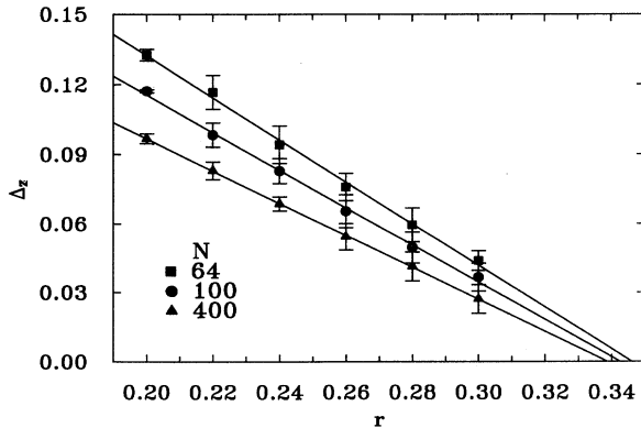
FIG. 6. The latent heat per bond \Delta_z along the first-order transition line, plotted against the hard-core repulsion parameter r . The tricritical point is located where the latent heat vanishes.
