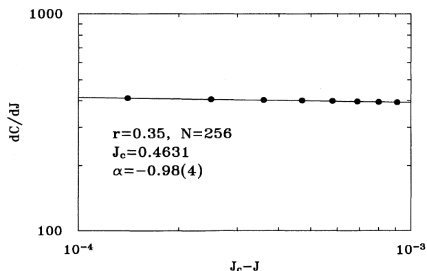
FIG. 12. The derivative of the specific heat dC/dJ as a function of J_c - J on logarithmic axes for N = 256 .
