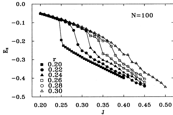
FIG. 5. The average energy per bond E_z as a function of J for several choices of the hard-core repulsion r for a system with N = 100 sites.
