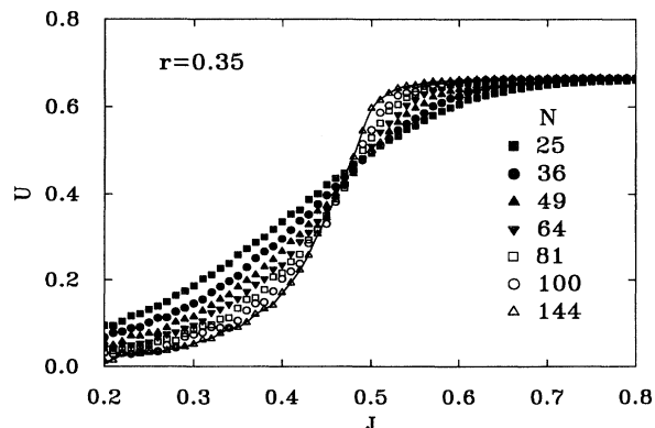
FIG. 14. The Binder fourth-order cumulant U as a function of J for fixed hard-core repulsion r = 0.35 and on several lattices with N spins. The solid line is a spline through the data for N = 144 .
