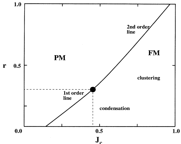
FIG. 15. The phase diagram for the dynamical random Ising model on a two-dimensional flat surface. The tricritical point (denoted by the solid circle) separates the first-order from the second-order transition lines. The paramagnetic (PM) and ferromagnetic (FM) phases are also shown.
