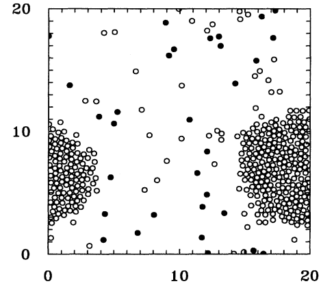
FIG. 2. A particular configuration of the system with N = 400 spins and r = 0.4 for J = 0.65 . Spins with S = \pm 1 are indicated with open and solid circles, respectively.
