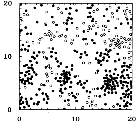
FIG. 1. A particular configuration of the system with N = 400 spins and r = 0.4 for J = 0.35 . Spins with S = \pm 1 are indicated with open and solid circles, respectively.
