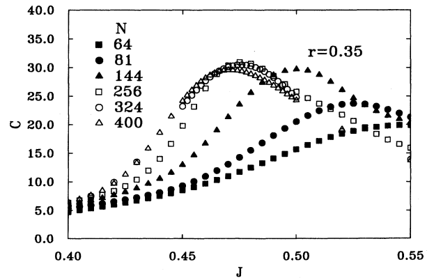
FIG. 11. Plot of the specific heat C versus ferromagnetic coupling J at r=0.35 , showing the absence of a growth in the peak with increasing lattice size (for the larger systems), in contrast to the behavior of the magnetic susceptibility. The errors (not shown) are smaller than the size of the symbols.
