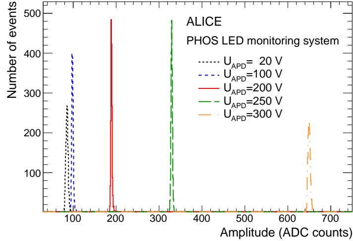
Figure 4: [Color online] The amplitude of the LED peak for different APD bias voltages, for one example channel.
