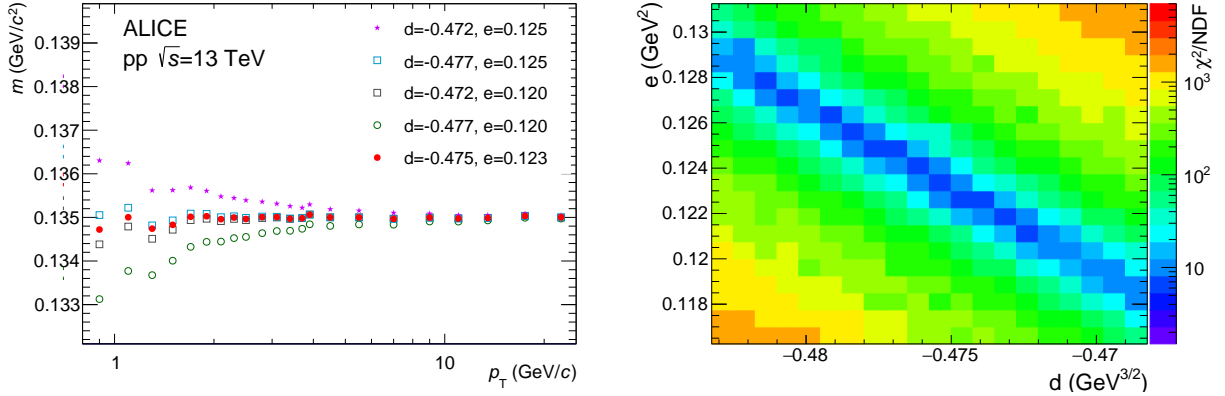
Figure 15: [Color online] Left: the \pi^0 peak position as a function of the transverse momentum for several values of nonlinearity parameters ( d, e ), with default values for a, b and c . Right: the deviation from a constant value of the \pi^0 peak position expressed in \chi^2/NDF as a function of the nonlinearity parameters ( d, e ).
