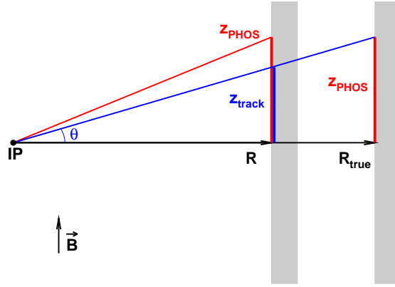
Figure 12: [Color online] An illustration of the dependence of \langle dz \rangle , from equation (6), with z , in a radially shifted detector. The magnetic field of 0.5 T is along the z direction.
