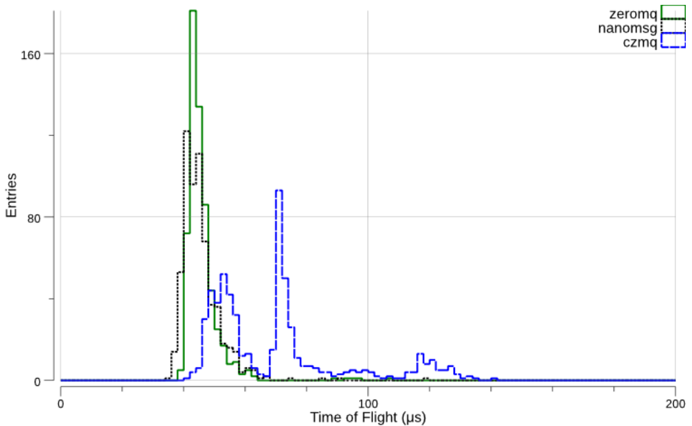
Figure 2: Distribution of the time of flight of a single token (uint64) through a pipeline p = \{ source | processor | sink \} , for different transports and protocols: zeromq, nanomsg and czmq. czmq is the C/C++ ZeroMQ library called from Go.
