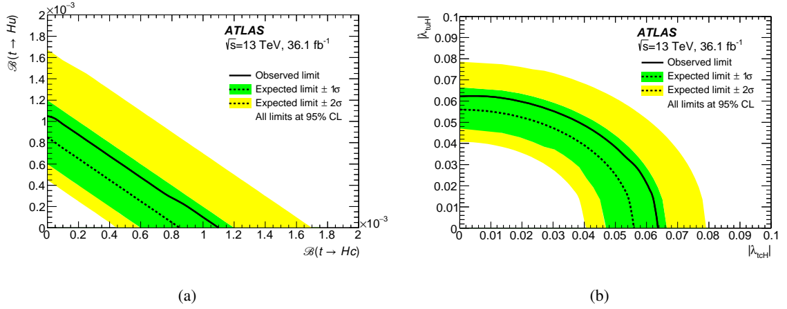
Figure 15: 95% CL upper limits (a) on the plane of \mathcal{B}(t \rightarrow Hu) versus \mathcal{B}(t \rightarrow Hc) and (b) on the plane of |\lambda_{tuH}| versus |\lambda_{tCH}| for the combination of the searches. The observed limits (solid lines) are compared with the expected (median) limits under the background-only hypothesis (dotted lines). The surrounding shaded bands correspond to the 68% and 95% CL intervals around the expected limits, denoted by \pm 1\sigma and \pm 2\sigma , respectively.
