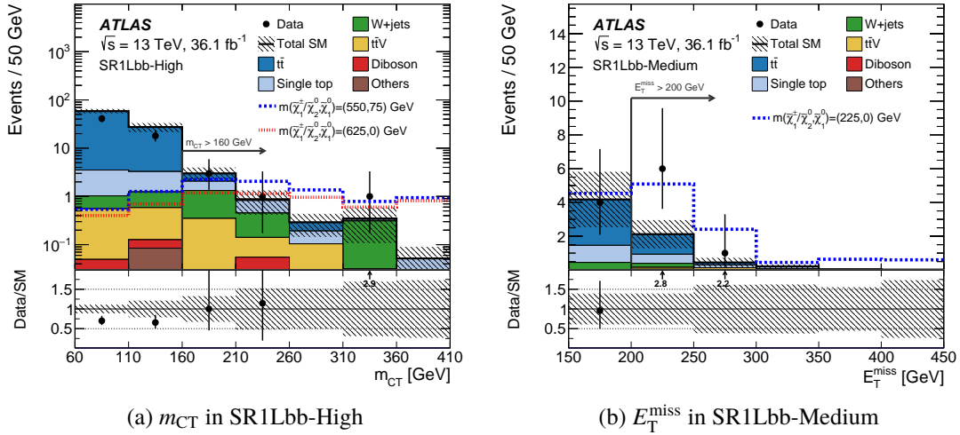
Figure 9: Data and SM predictions in SRs for the 1l b\bar{b} analysis for (a) m_{CT} in SR1Lbb-High and (b) E_T^{\text{miss}} in SR1Lbb-Medium. All SRs selections but the one on the quantity shown are applied. All uncertainties are included in the uncertainty band. Example SUSY models are superimposed for illustrative purposes.
