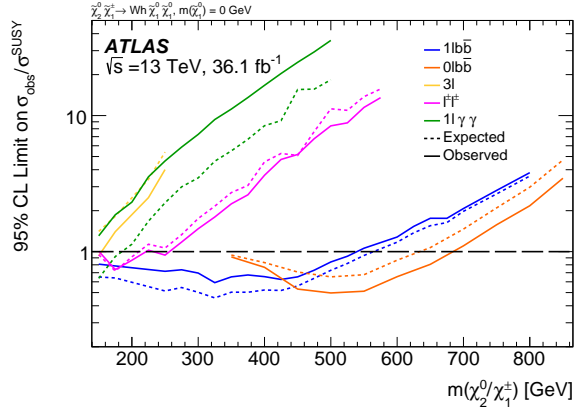
(b) 1-D exclusion for m(\tilde{\chi}_1^0) = 0 \text{ GeV} .
