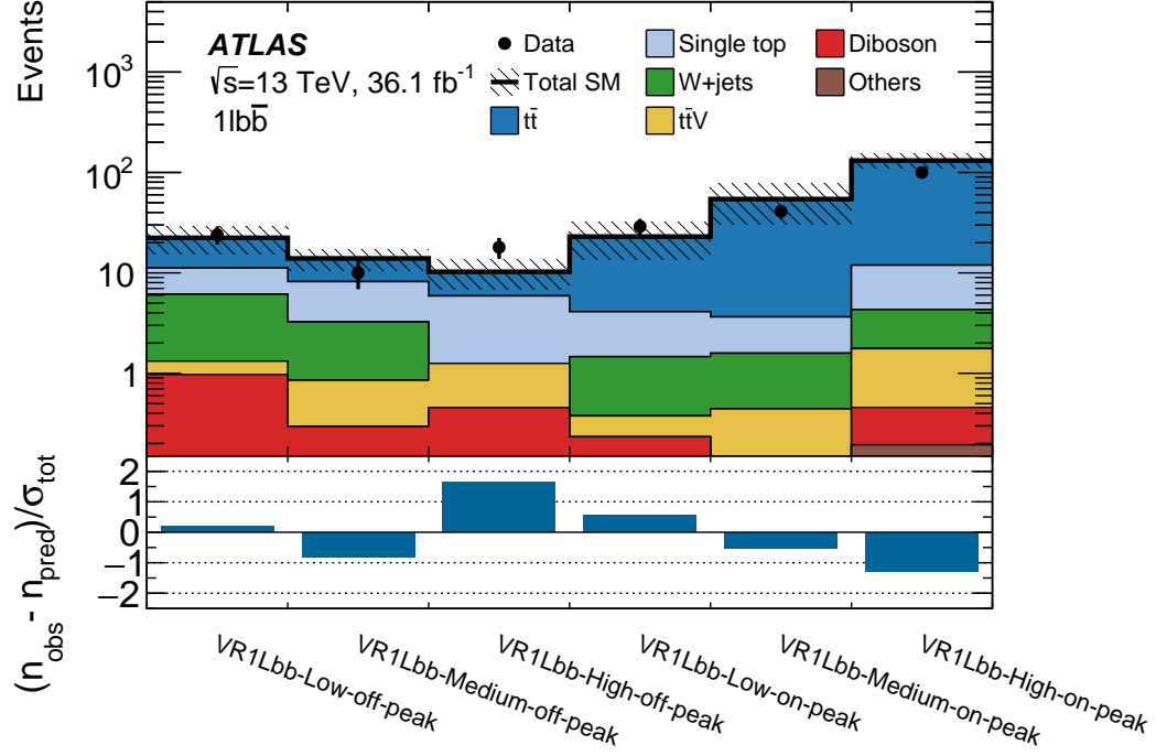
Figure 5: Comparison of the predicted backgrounds with the observed numbers of events in the validation regions associated with the 1lbb channel. The normalization of the backgrounds is obtained from the fit to the CRs. The upper panel shows the observed number of events and the predicted background yield. All uncertainties are included in the uncertainty band. The lower panel shows the pulls in each VR.
