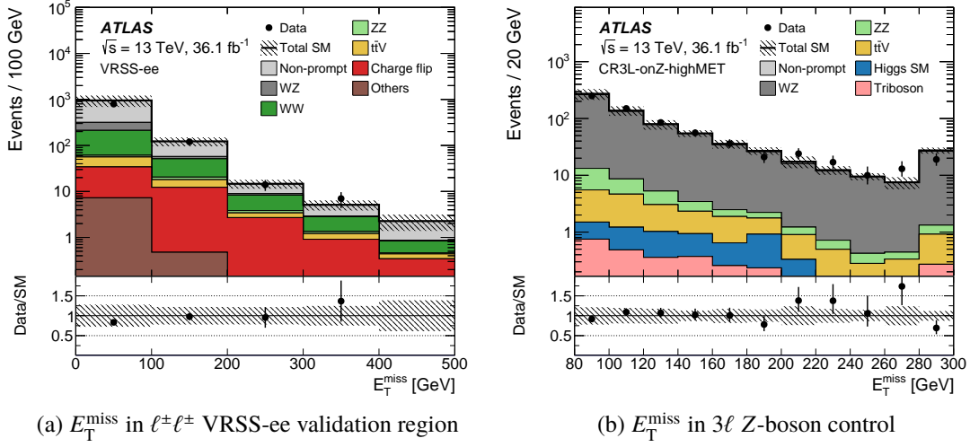
Figure 6: (a) E_T^{\text{miss}} distribution in the electron-type VRSS-ee for \ell^\pm\ell^\pm channel (used to estimate FNP leptons background) and (b) E_T^{\text{miss}} distribution in the on-shell Z-boson CR for 3\ell (used to estimate the WZ normalization).
