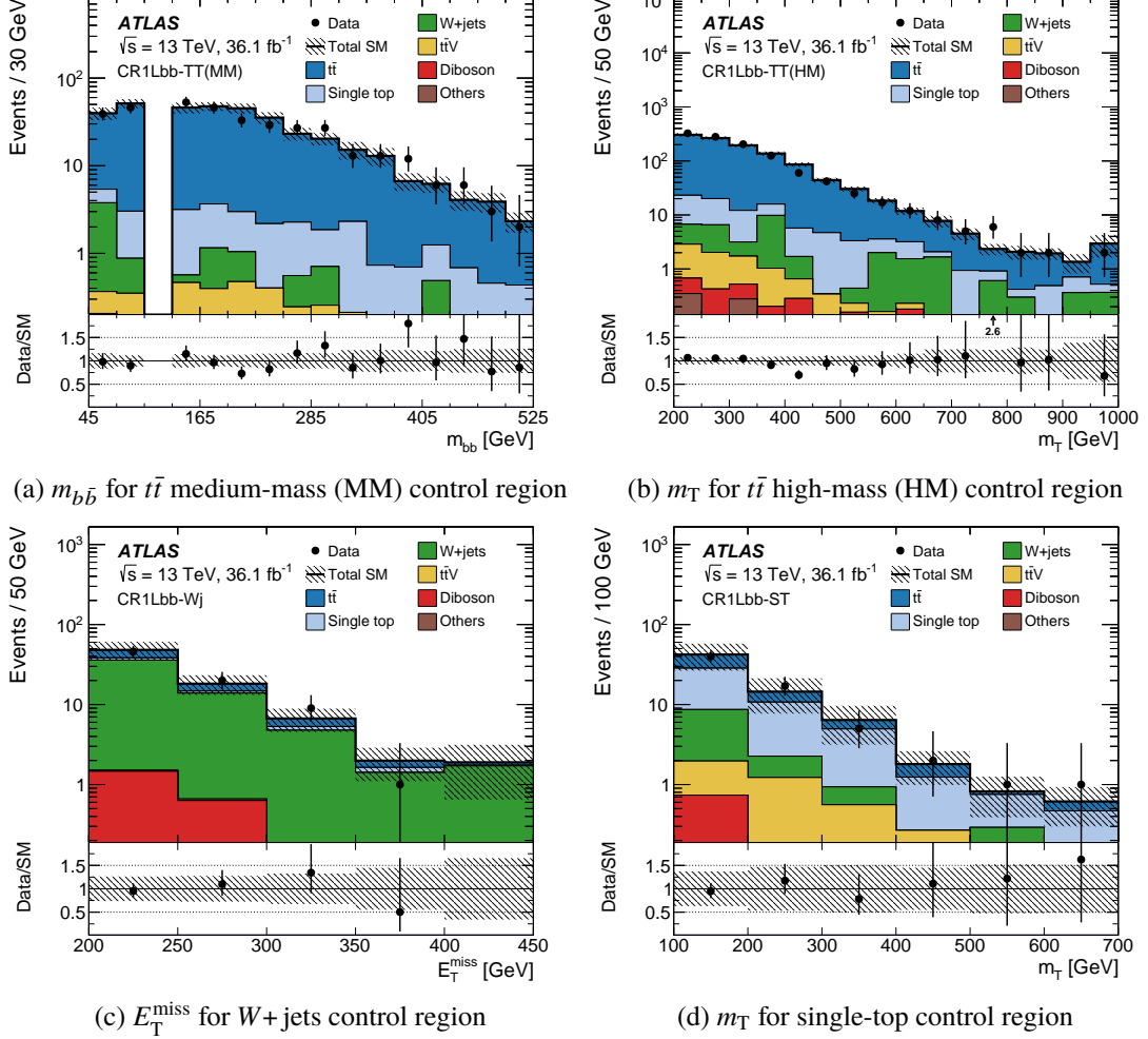
Figure 4: Comparison of data with SM predictions in t\bar{t} , W + jets, and single-top control regions for representative kinematic distributions: (a) m_{b\bar{b}} for CR1Lbb-TT medium, (b) m_T for CR1Lbb-TT high, (c) E_T^{\text{miss}} for CR1Lbb-Wj and (d) m_T for CR1Lbb-ST. Predictions from MC simulation are shown after the background-only fit. The uncertainty bands include statistical and systematic uncertainties.
