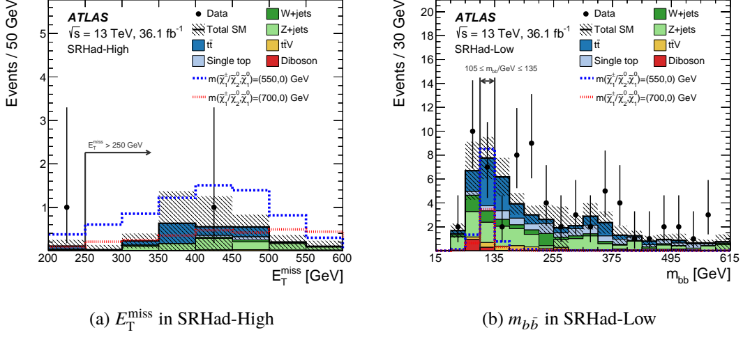
Figure 8: Data and SM predictions in SRs for the 0l b\bar{b} analysis for (a) E_T^{\text{miss}} in SRHad-High and (b) m_{b\bar{b}} in SRHad-Low. All SRs selections but the one on the quantity shown are applied. All uncertainties are included in the uncertainty band. Two example SUSY models are superimposed for illustrative purposes.
