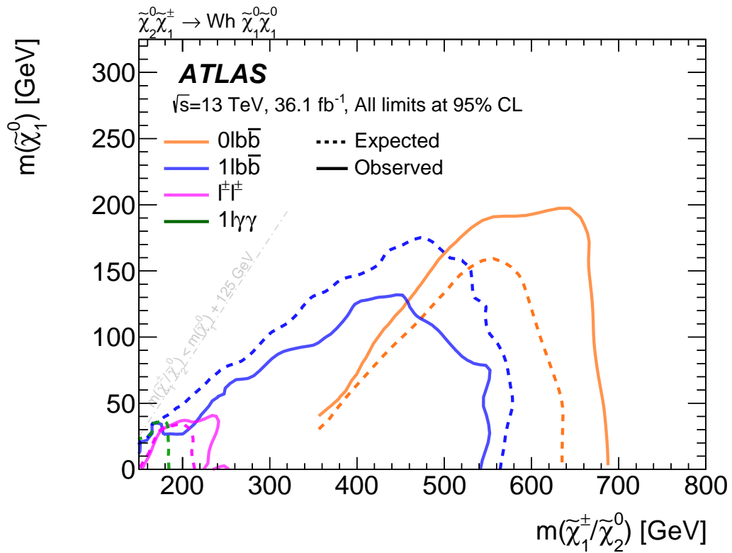
Figure 14: Comparison of the expected and observed exclusions for each analysis channel studied. Only the expected exclusion is shown for the 1l\gamma\gamma channel since the observed exclusion does not appear due to the excess observed.
