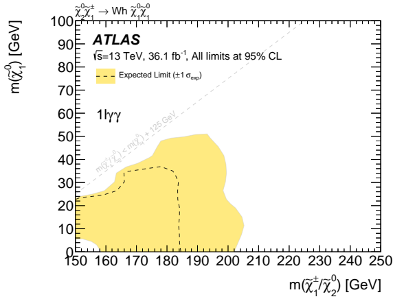
(c) 1l\gamma\gamma
