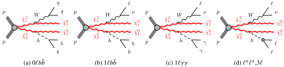
Figure 1: Diagrams illustrating the signal scenarios considered for the pair production of chargino and next-to-lightest neutralino targeted by the (a) hadronic ( 0\ell b\bar{b} ) and (b) 1\ell b\bar{b} , (c) 1\ell\gamma\gamma , (d) \ell^\pm\ell^\pm, 3\ell leptonic channel selections. In (a) and (b) the Higgs boson decays into two b -quarks. In (c), the diphoton channel is shown with h \rightarrow \gamma\gamma . In (d), the visible multilepton final state of the Higgs boson is shown. Leptons are either electrons or muons.
