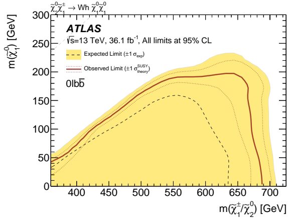
(a) 0l\bar{b}\bar{b}
