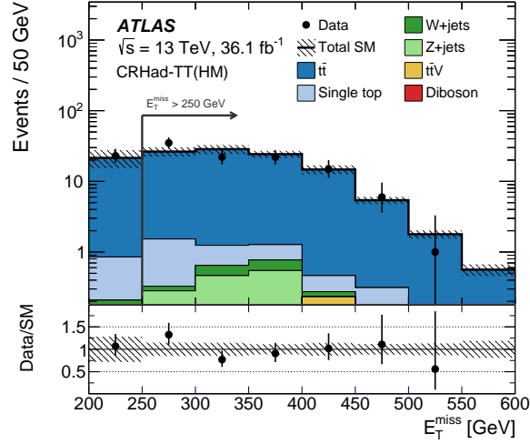
(a) t\bar{t} high-mass control region
