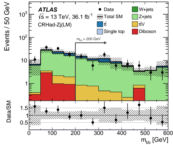
(b) Z + jets low-mass control region
