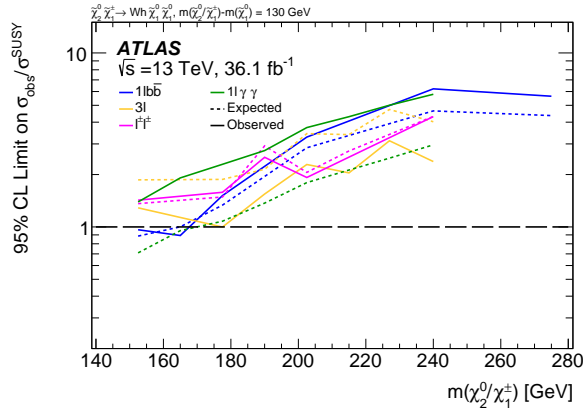
(a) 1-D exclusion for m(\tilde{\chi}_2^0) - m(\tilde{\chi}_1^0) = 130 \text{ GeV} .
