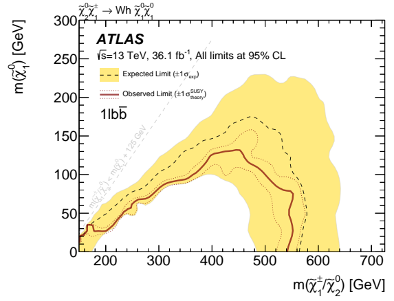
(b) 1l\bar{b}\bar{b}
