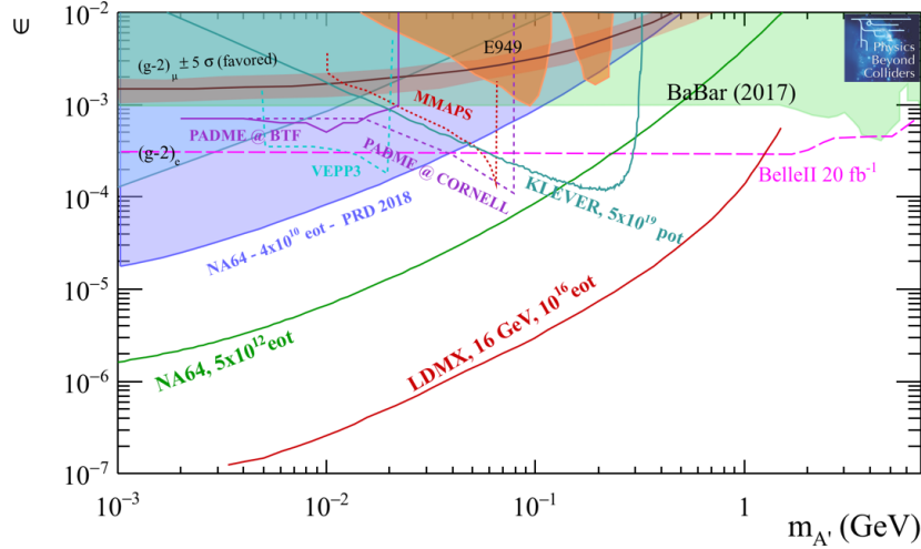
Figure 22: Dark Photon decaying to invisible final states. Prospects for PBC projects on a timescale of 5 years (NA64 ++ ( e ), green line) and 10-15 years (LDMX, red line and KLEVER, cyan line) compared to the current bounds (solid areas) and future experimental landscape (other solid and dashed lines) as explained in Figure 21.
