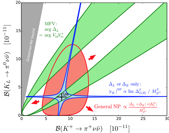
Figure 42: Scheme for BSM modifications of K \rightarrow \pi \nu \bar{\nu} BRs. Reproduced from Ref. [340].
