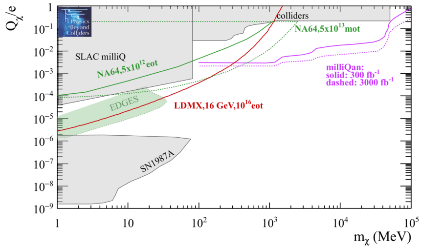
Figure 25: BC3: milli-charged particles. Current bounds (filled areas), experimental landscape and physics reach of PBC projects in 5 years time scale (NA64 ++ ( e ) and NA64 ++ ( \mu )), and on 10-15 years time scale (LDMX @ eSPS).
