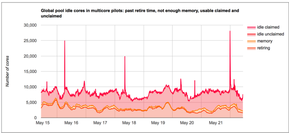
Fig. 4. Sources of idle CPU cores in the CMS Global Pool. Major contributions include retiring pilots and memory-starved pilots.
