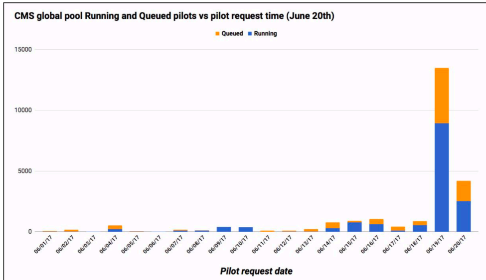
Fig. 6. Up to two-week-old glideins in the queues and running at sites in June 2017.
