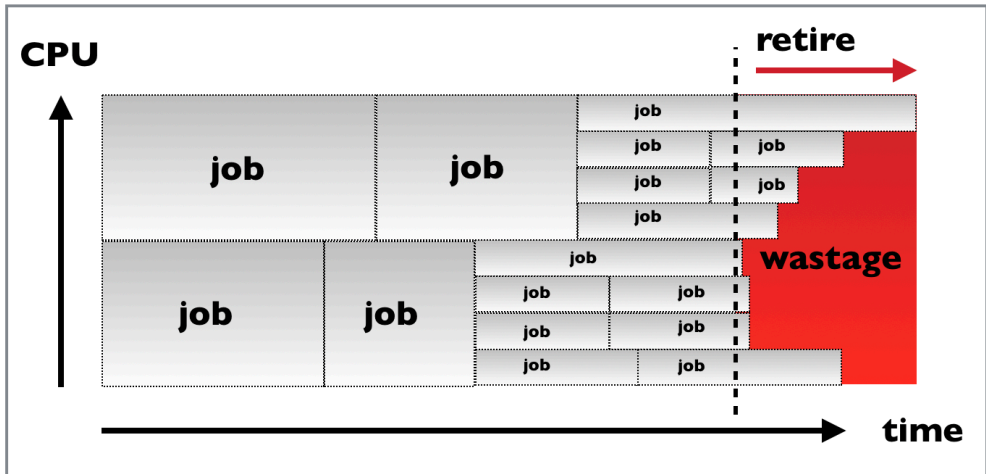
Fig. 2. Evolution of multi-core pilot fragmentation and draining.
