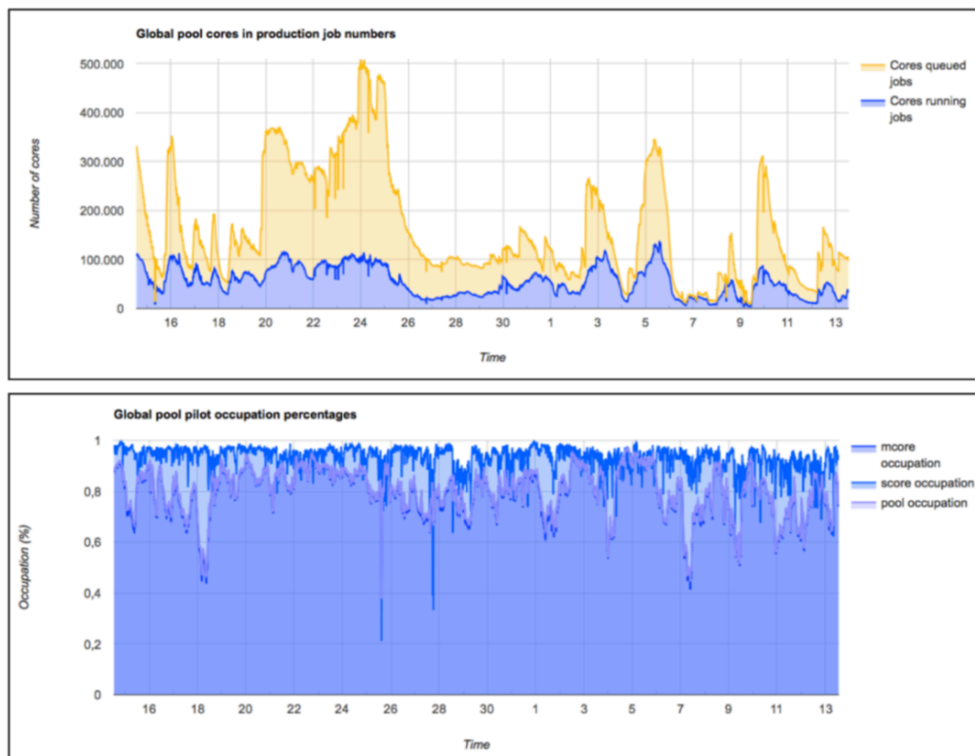
Fig. 5. Bursts of job submission and draining effect on the Global Pool.
