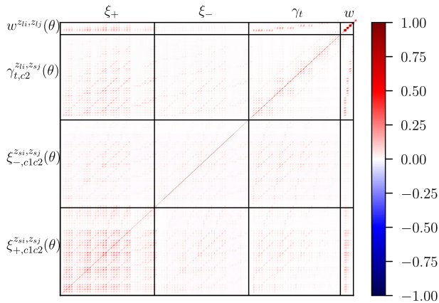
Figure D2. Correlation matrix for the multiprobe multicolour datavektor. The matrix contains 2240 \times 2240 elements, and includes shear ( \xi_{\pm} ), galaxy–galaxy lensing ( \gamma_l ), and galaxy clustering ( w ) measurements, including all cross-correlations between the various statistics. Within each block, elements are grouped by \theta bin, then by redshift bin couplet and finally by galaxy type pairing.
