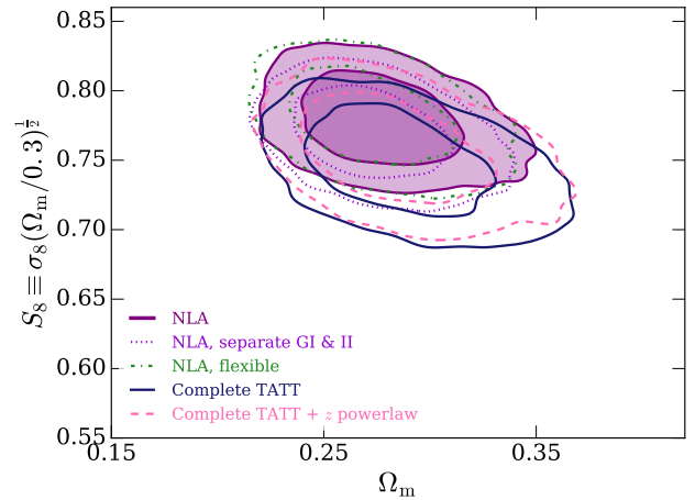
Figure 7. \Lambda CDM constraints on S_8 and \Omega_m from cosmic shear, galaxy clustering and galaxy-galaxy lensing, using the unsplit Y1 cosmology sample. The solid filled (purple) contours show the baseline analysis, which assumes the nonlinear alignment model for intrinsic alignments, and is equivalent to the blue contours in Figure 11 of Dark Energy Survey Collaboration (2017). The other lines show extended IA models, the parameters of which are listed in Table 1.
