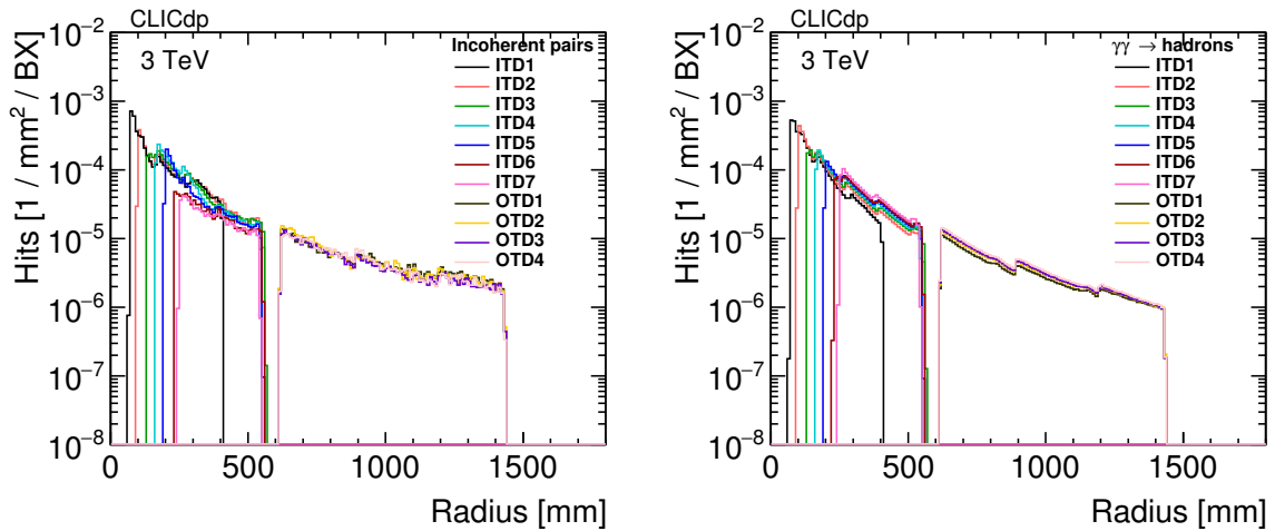
Figure 19: Hit densities per bunch crossing in the tracker disks from incoherent electron–positron pairs (left) and \gamma\gamma \rightarrow hadrons (right) at 3 TeV. Safety factors are not included.
