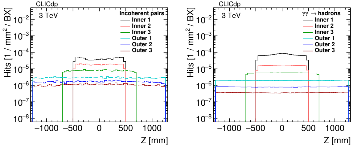
Figure 18: Hit densities per bunch crossing in the tracker barrel layers from incoherent electron–positron pairs (left) and \gamma\gamma \rightarrow hadrons (right) at 3 TeV. Safety factors are not included.
