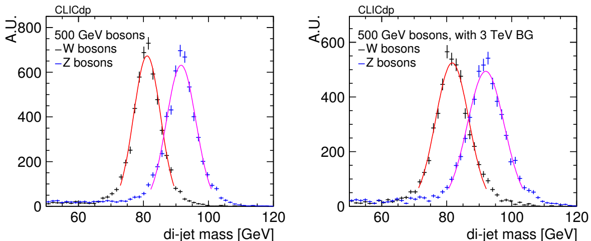
Figure 61: Di-jet mass distributions of hadronically decaying W and Z with E = 500 GeV in WW \rightarrow lvqq and ZZ \rightarrow v\nu q\bar{q} events, together with Gaussian fits of the di-jet mass for events without beam-induced backgrounds (left) and overlay of 3 TeV beam-induced backgrounds from \gamma\gamma \rightarrow hadrons (right).
