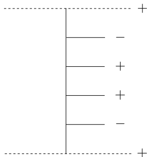
Figure 3. Region \varrho_{8,1} .
