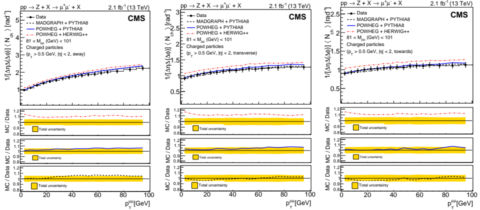
Fig. 3. Average charged particle density as a function of the dimuon transverse momenta in the away (left), transverse (center) and towards (right) regions. Figures were extracted from Ref. [3].
