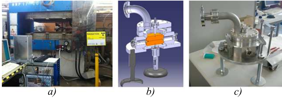
Figure 2: The facility for studying high-gradient DC breakdowns in the magnetic field at CERN: a) LES inside of electromagnet, b) 3D model of LES, c) the photo of LES.
