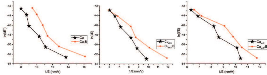
Figure 8: Dependence of the dark current on the electric field strength
