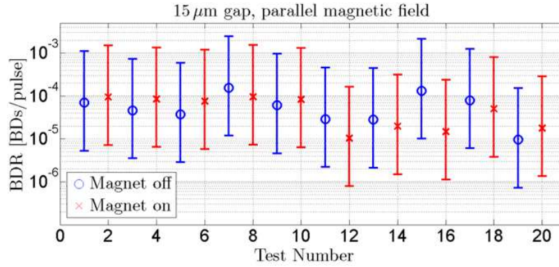
Figure 4: The measured BDR in the Large Electrodes System with a 15 \mu\text{m} gap size with and without an external about 0.5 T magnetic field applied parallel to the electrodes.
