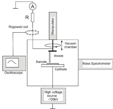
Figure 5: Block diagram of the installation for the study of high-voltage breakdowns
