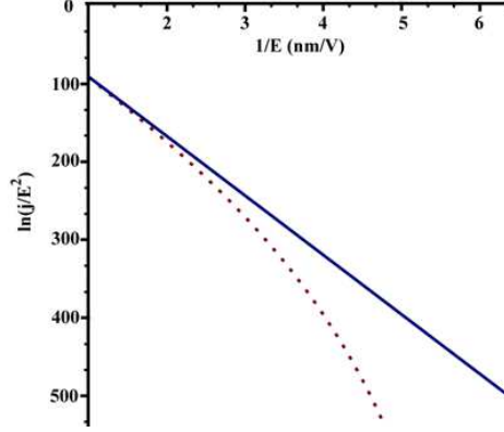
Figure 1: Influence of a magnetic field on a field emission current in logarithmic coordinates according to the generalized Fowler-Nordheim equation. Solid line shows the field emission current in the absence of a magnetic field. The current in the presence of an external magnetic field of 0.5 T parallel to the surface is shown with the dotted line.
