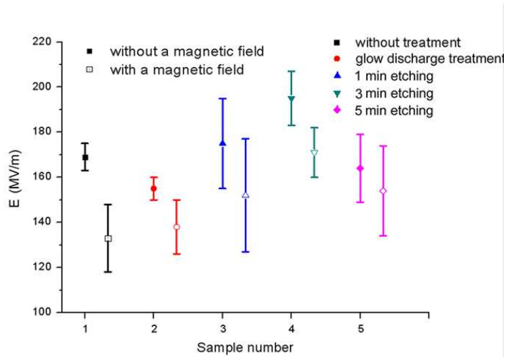
Figure 7: The dependence of breakdown voltages of different surface treatments for copper samples in the presence and absence of a magnetic field.
