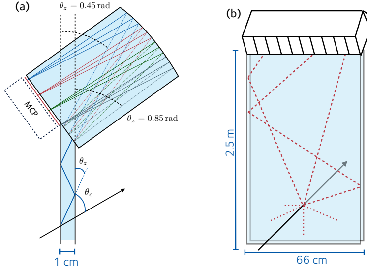
Figure 1: Schematics of a TORCH module showing possible reflection paths: (a) the focussing block and MCP plane, (b) a single LHCb module.
