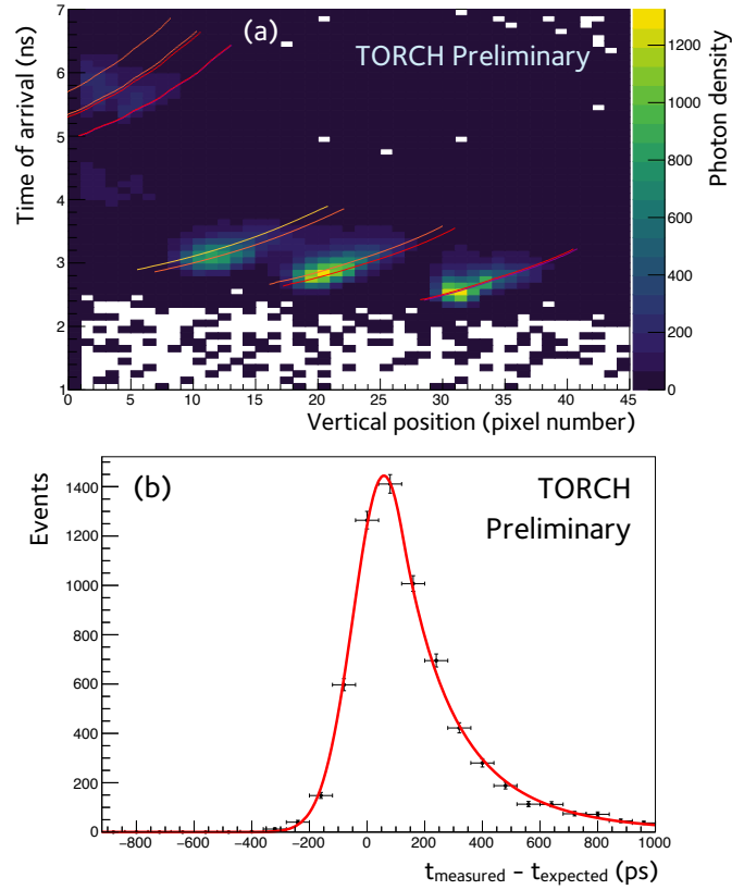
Figure 2: (a) The time-of-arrival of single Cherenkov photons from a 5 GeV/c pion beam, relative to a beam time-reference station, as a function of detected vertical column pixel number. The overlaid lines represent the simulated patterns for light reflected only off the front and back faces of the radiator plate (lower right distribution), light also undergoing one and two reflections off the side faces (lower central and left distributions, respectively), and multiple reflections from the bottom horizontal face (top left distributions). (b) The distribution of residuals between the measured Cherenkov photon arrival times with respect to the simulated distribution, with a “crystal ball” fit superimposed.
