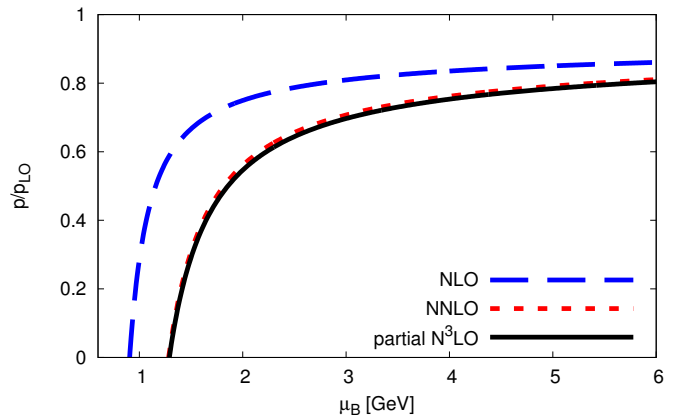
FIG. 2. The pressure of cold and dense massless QCD, normalized to the free pressure, as a function of baryon chemical potential for the renormalization scale choice \bar{\Lambda} = 2\mu_B/3 and \Lambda_{\overline{\text{MS}}} = 0.378 GeV.
