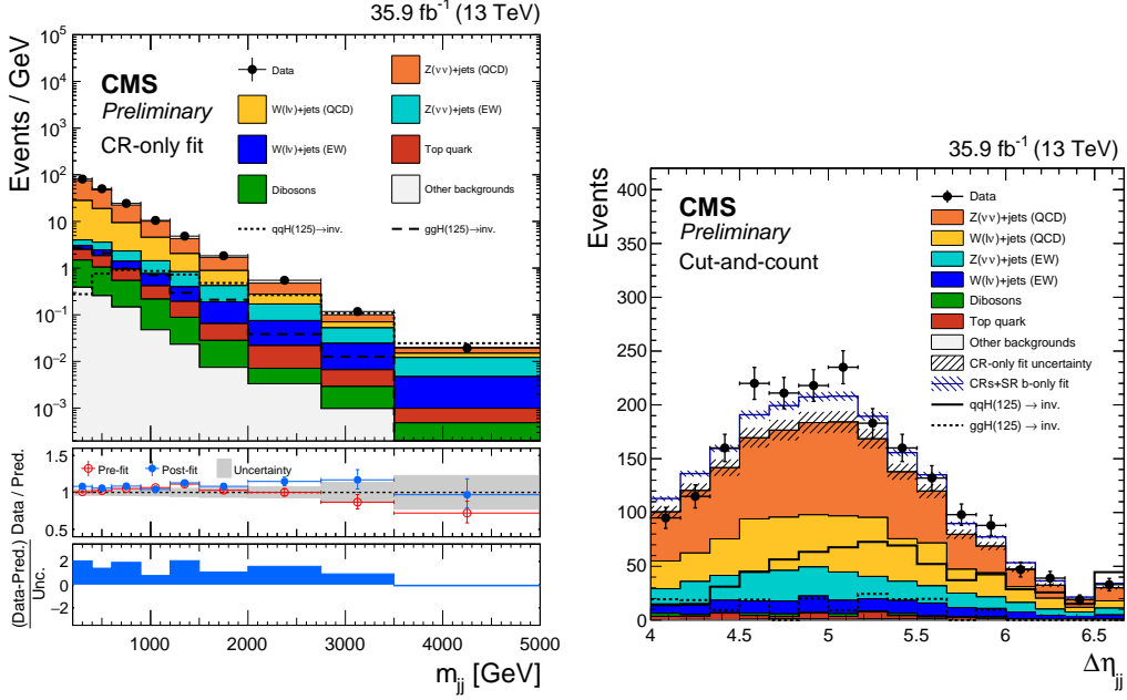
Figure 1: The observed m_{jj} distribution in the signal region compared to the post-fit backgrounds from various SM processes for the shape analysis obtained from a combined fit to the data in all the CRs, but excluding the SR (left). The observed \Delta\eta_{jj} distribution in the signal region compared to the post-fit backgrounds from various SM processes for the cut-and-count approach (right) [11].
