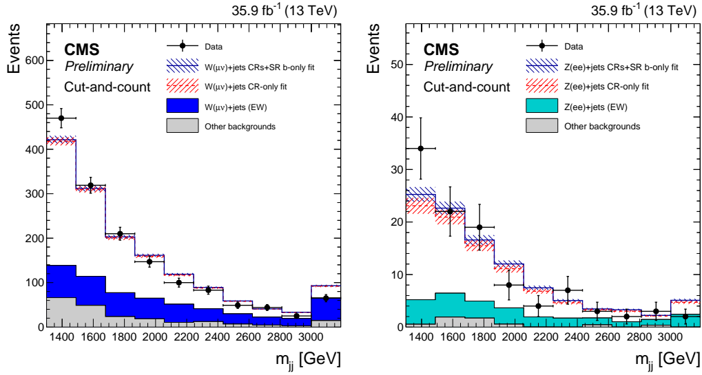
Figure 2: The observed m_{jj} distribution in the single muon (left) and dielectron (right) control regions compared to the post-fit backgrounds from various SM processes for the cut-and-count approach [11].
