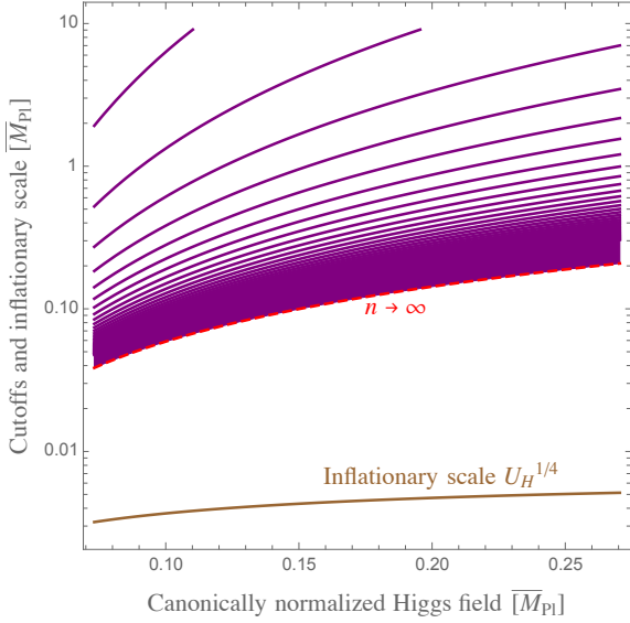
Figure 6: The same as in Fig. 5 but here the intermediate field regime ( \bar{M}_{Pl}/\xi_H \ll \bar{\phi} \ll \bar{M}_{Pl}/\sqrt{\xi_H} ) is shown.
