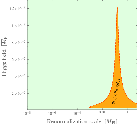
Figure 3: Configuration space in (B.3) and (B.4) for the parameters set in Fig. 1. This space opens up only at \bar{\mu} \gg |H_{\pm}| so no instability configurations are found.
