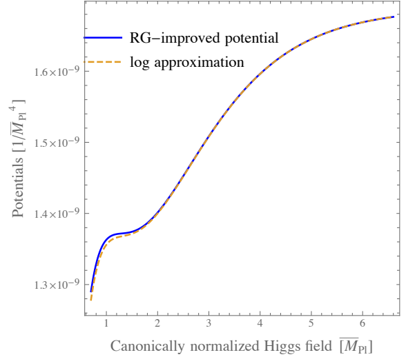
Figure 4: RG-improved potential and its approximation (log-approximation) based on the expansions in Eq. (34) for the parameters set in Fig. 1 and for \kappa \approx 1.8 .
