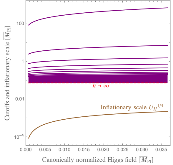
Figure 5: The cutoff of the theory obtained by reading the coefficients of the dimension- n operators \delta\phi^n (for n > 4 and varying n ) is compared to the inflationary scale. The parameters are chosen as in Fig. 4. In this plot the small field regime ( \bar{\phi} \ll \bar{M}_{\text{Pl}}/\xi_H ) is shown.
