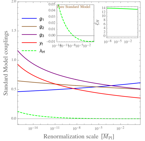
Figure 1: RG evolution of the relevant SM parameters close to criticality ( \lambda_H is nearly zero at the Planck scale). The values of the parameters are the following: M_1 = 10^{11} GeV, M_2 = 6.5 \times 10^{13} GeV, M_3 > \bar{M}_{\text{Pl}} , z = 0 , \xi = 1 , f_a \approx 2.5 \times 10^{10} GeV, \lambda_{HA}(M_A) \approx 0.016 , \lambda_A(M_A) \approx 0.1 , y(M_A) \approx 0.09 . The inset on the left shows the running of \lambda_H in the pure SM for the same values of the SM parameters.
