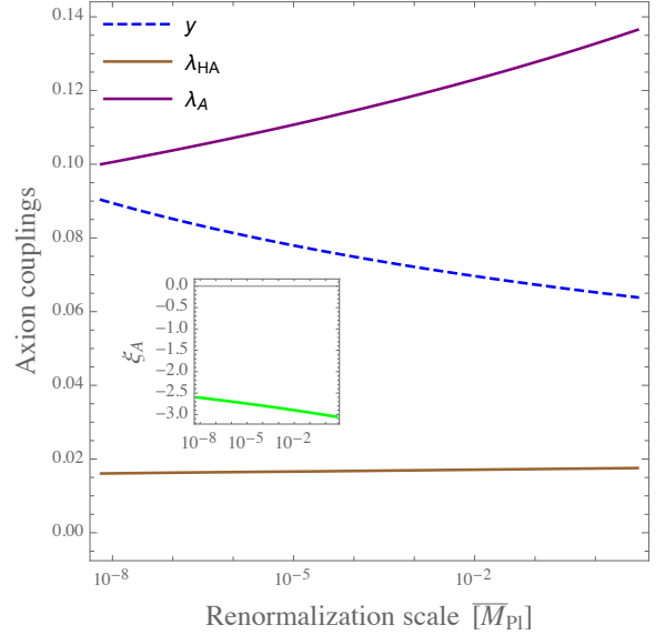
Figure 2: RG evolution of the couplings of the axion sector close to criticality ( \lambda_H is nearly zero at the Planck scale). The values of the parameters are as in Fig. 1 .
