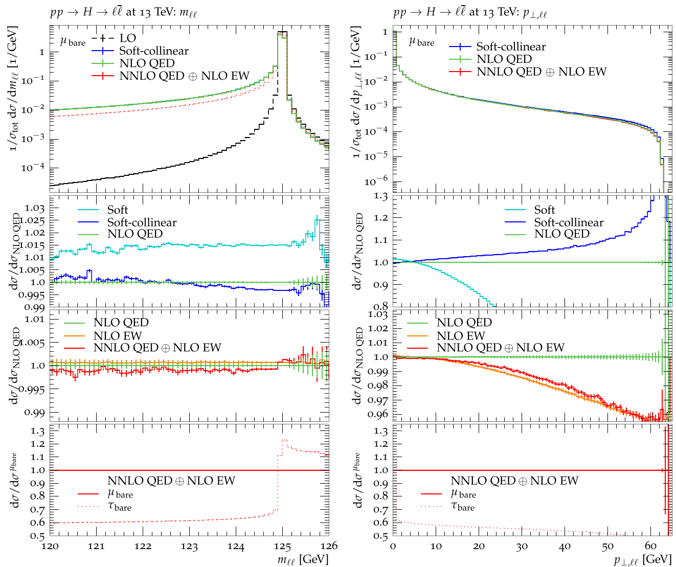
Fig. 8 Plots of the invariant mass of the two decay leptons, m_{\ell\ell} , on the left and the transverse momentum of the system of the two leptons, p_{\perp,\ell\ell} , on the right in the process pp \rightarrow H \rightarrow \ell^+\ell^- . Nominal predictions are shown for pp \rightarrow H \rightarrow \mu^+\mu^- at LO, in soft-collinear NLO
