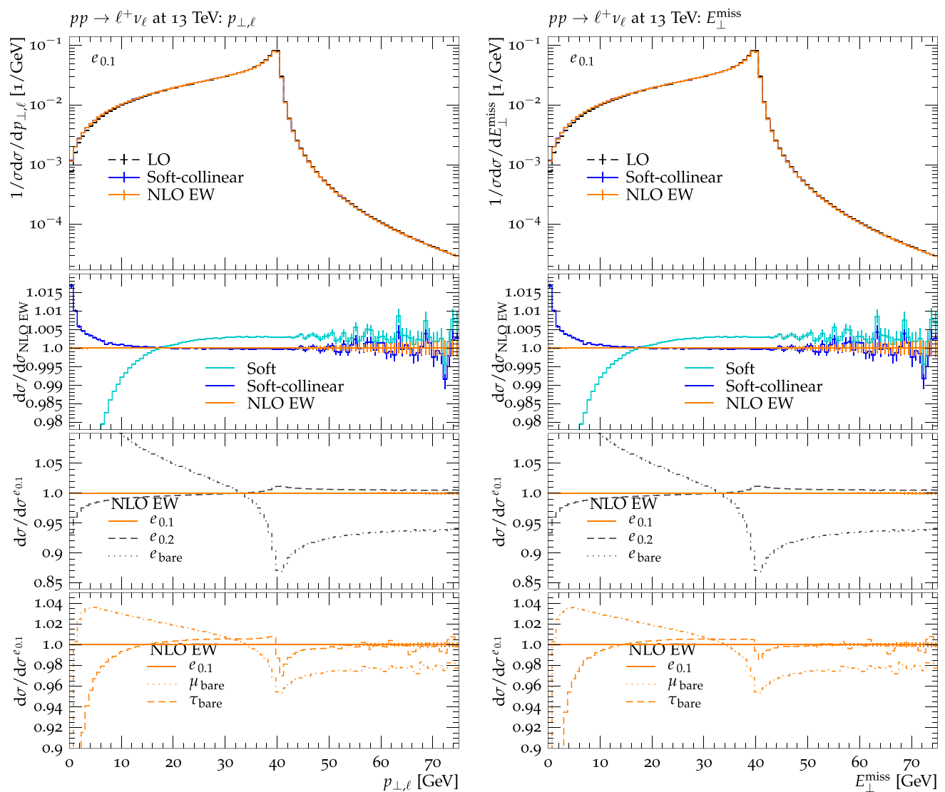
Fig. 6 Plots of the transverse momentum of the charged leptons, p_{\perp,\ell} , on the left and the missing transverse E_{\perp}^{\text{miss}} , on the right. Predictions and labels as in Fig. 5
