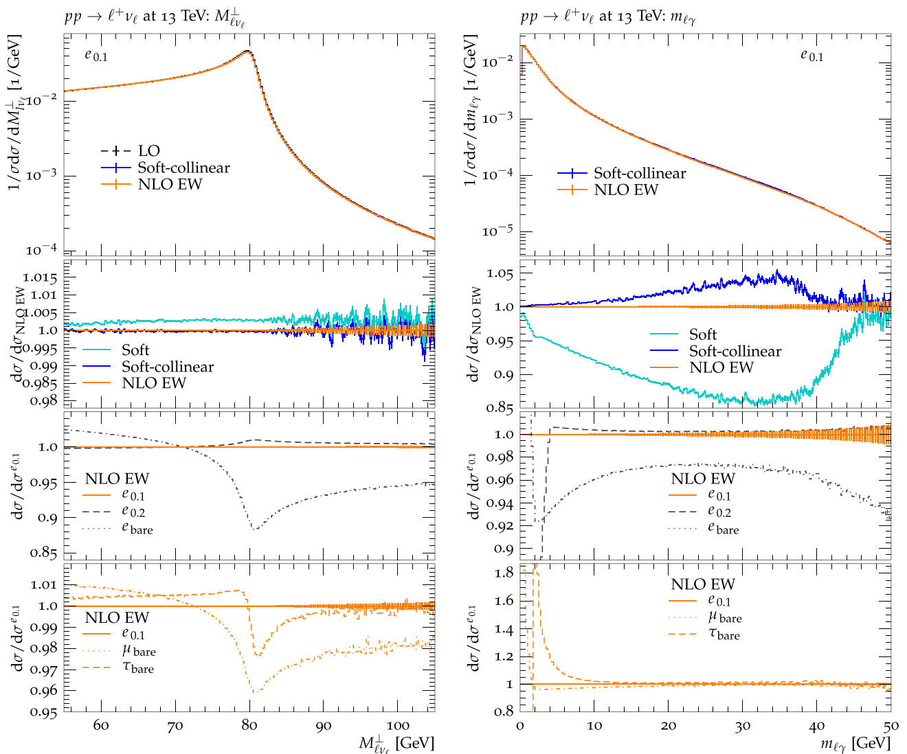
Fig. 5 Transverse mass of the lepton-neutrino system M_{\ell\nu_\ell}^\perp (left) and the invariant mass of the system of the charged lepton and the nearest photon, m_{\ell\gamma} (right) in pp \rightarrow W^+ \rightarrow \ell^+ \nu_\ell . Nominal predictions are shown for pp \rightarrow W^+ \rightarrow e^+ \nu_e at LO, in soft-collinear NLO approxima-
